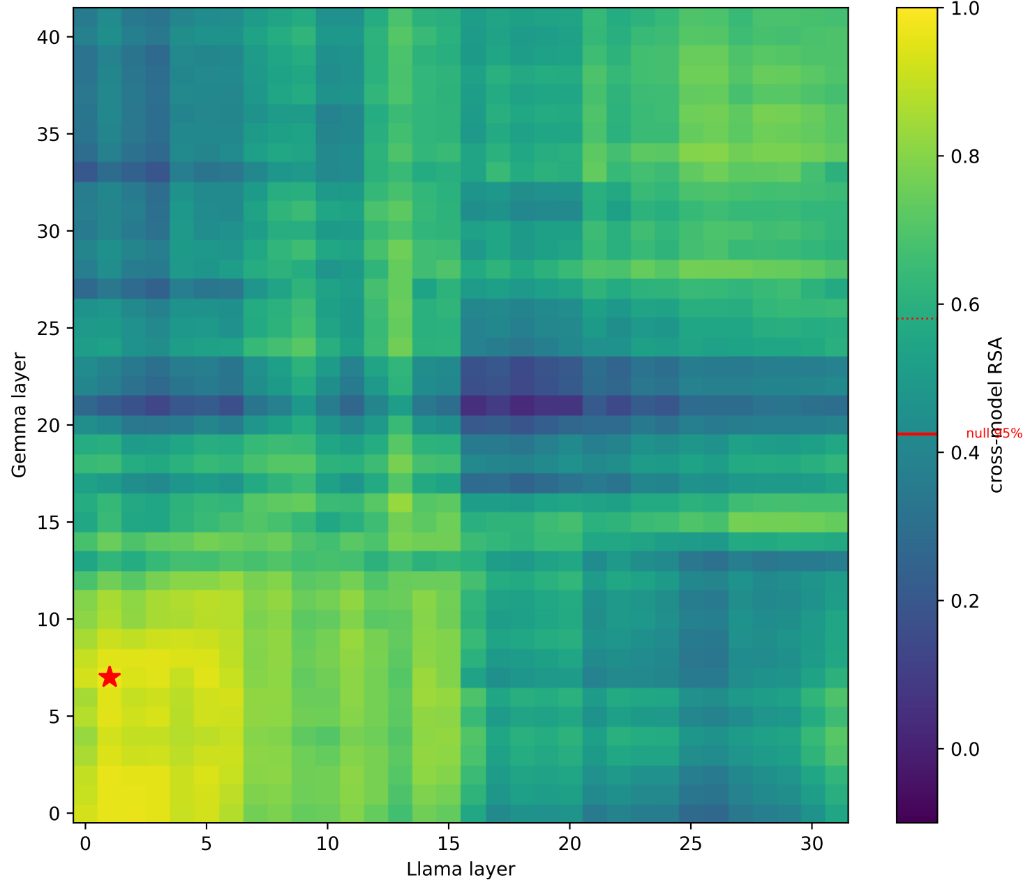
days (n=7): Gemma vs Llama cross-model RSA (max 0.97; null95=0.42, null99=0.58)
