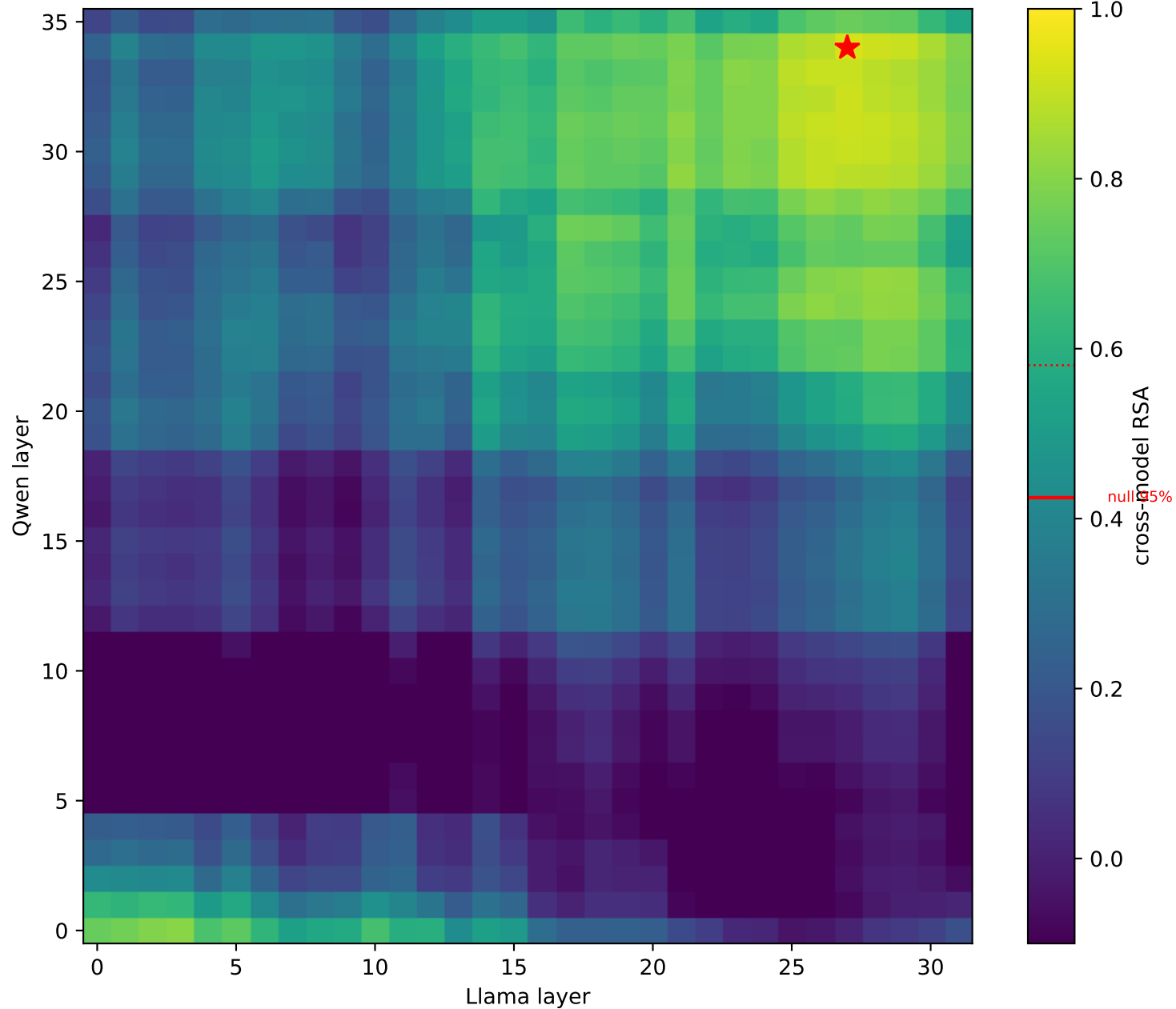
days (n=7): Qwen vs Llama cross-model RSA (max 0.93; null95=0.42, null99=0.58)
