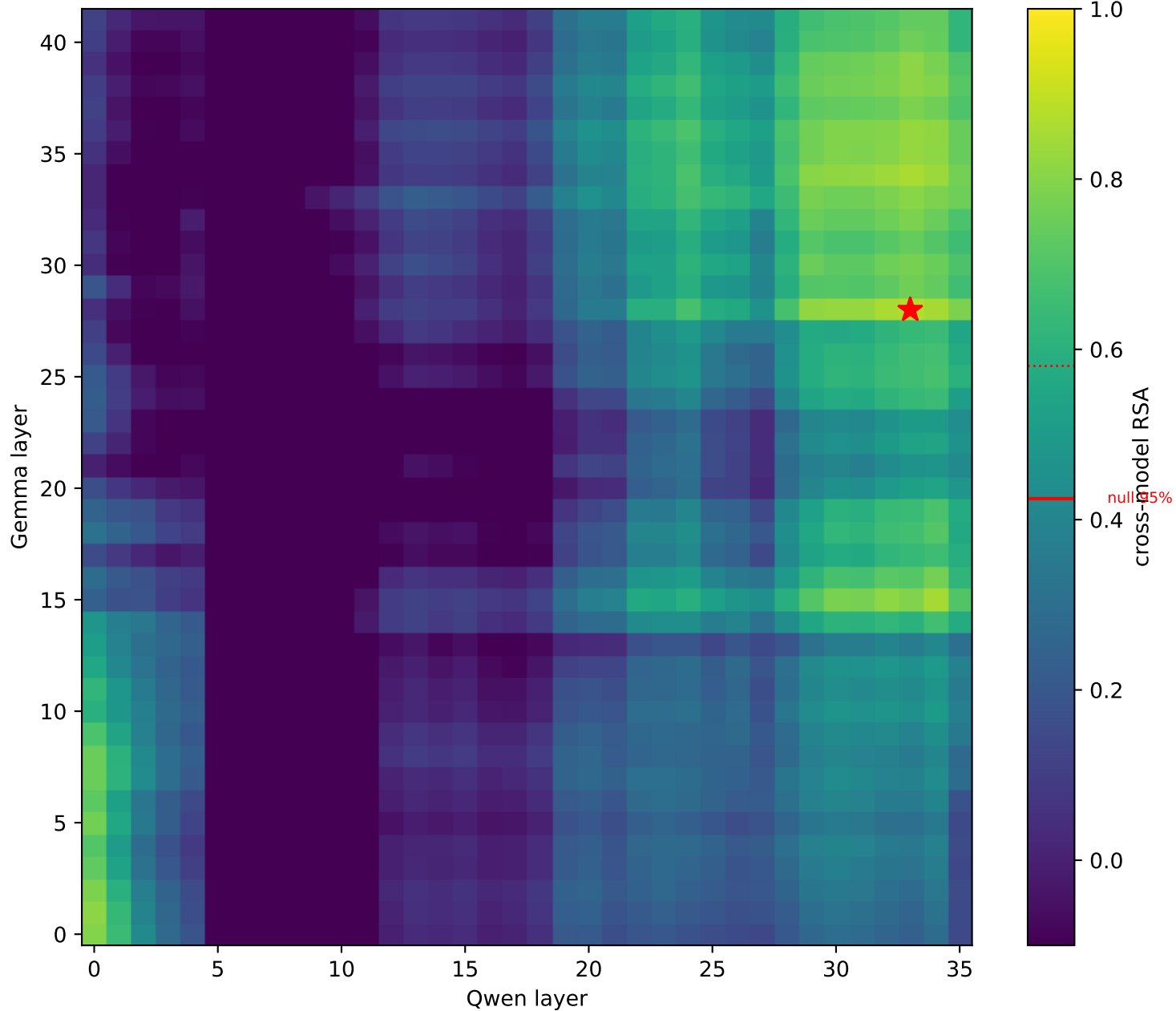
days (n=7): Gemma vs Qwen cross-model RSA (max 0.87; null95=0.42, null99=0.58)
