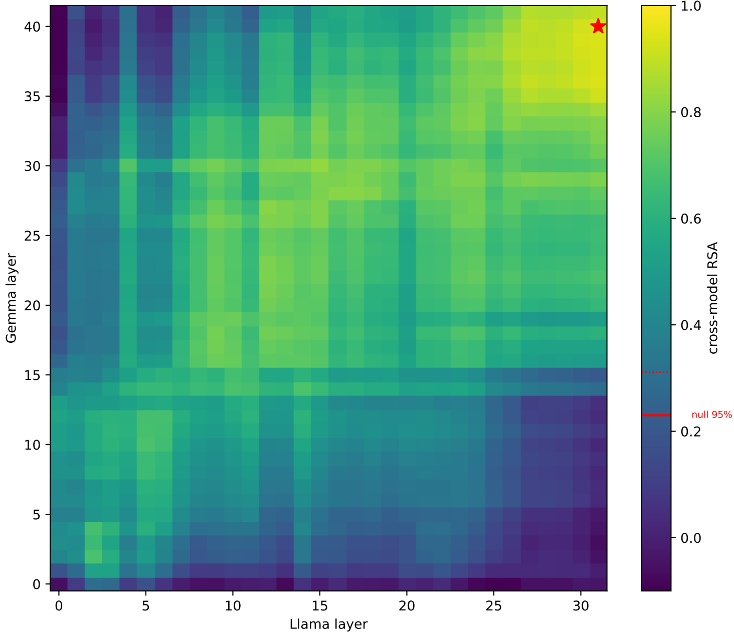
ring (n=16): Gemma vs Llama cross-model RSA (max 0.94; null95=0.23, null99=0.31)
