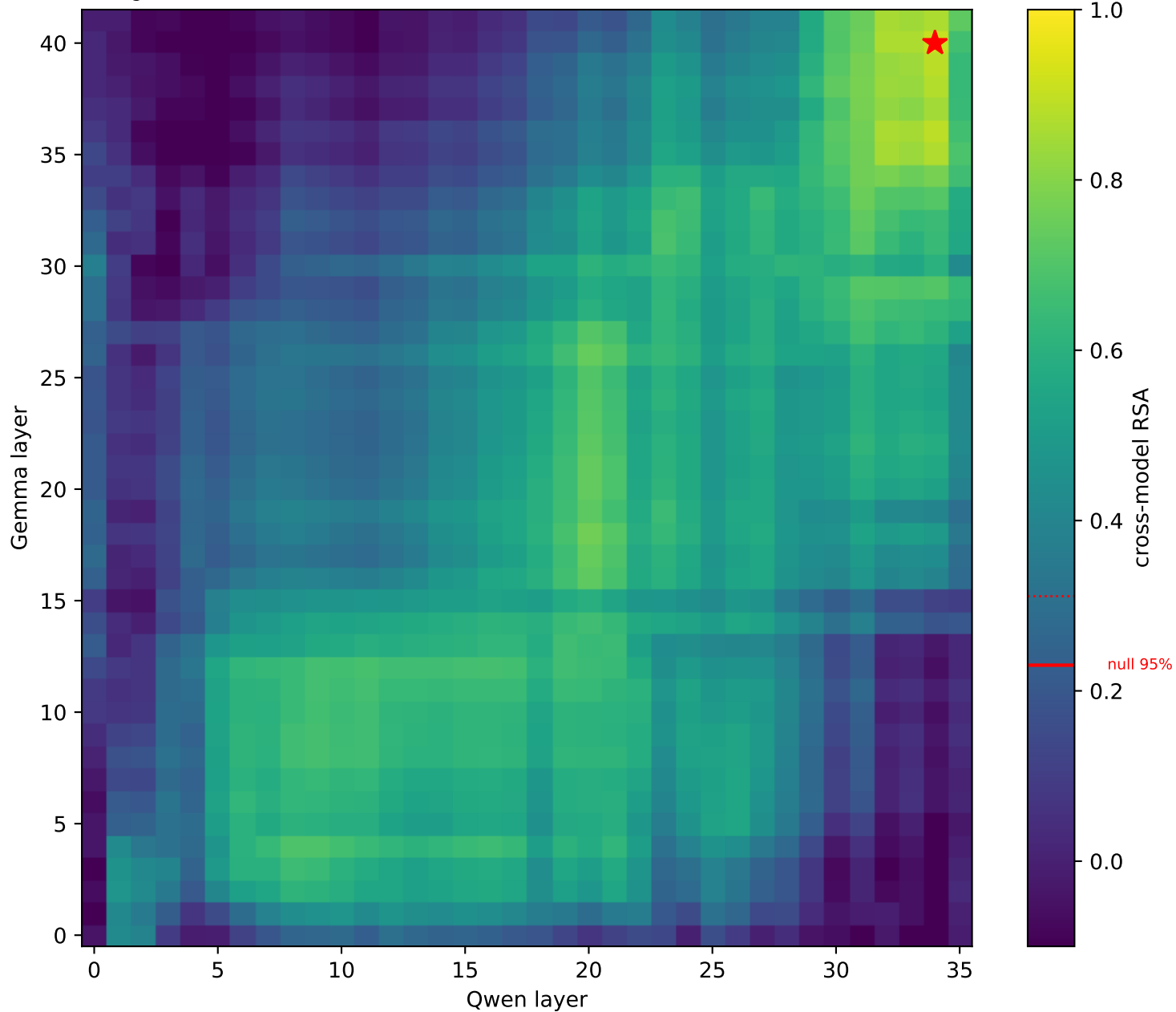
ring (n=16): Gemma vs Qwen cross-model RSA (max 0.91; null95=0.23, null99=0.31)
