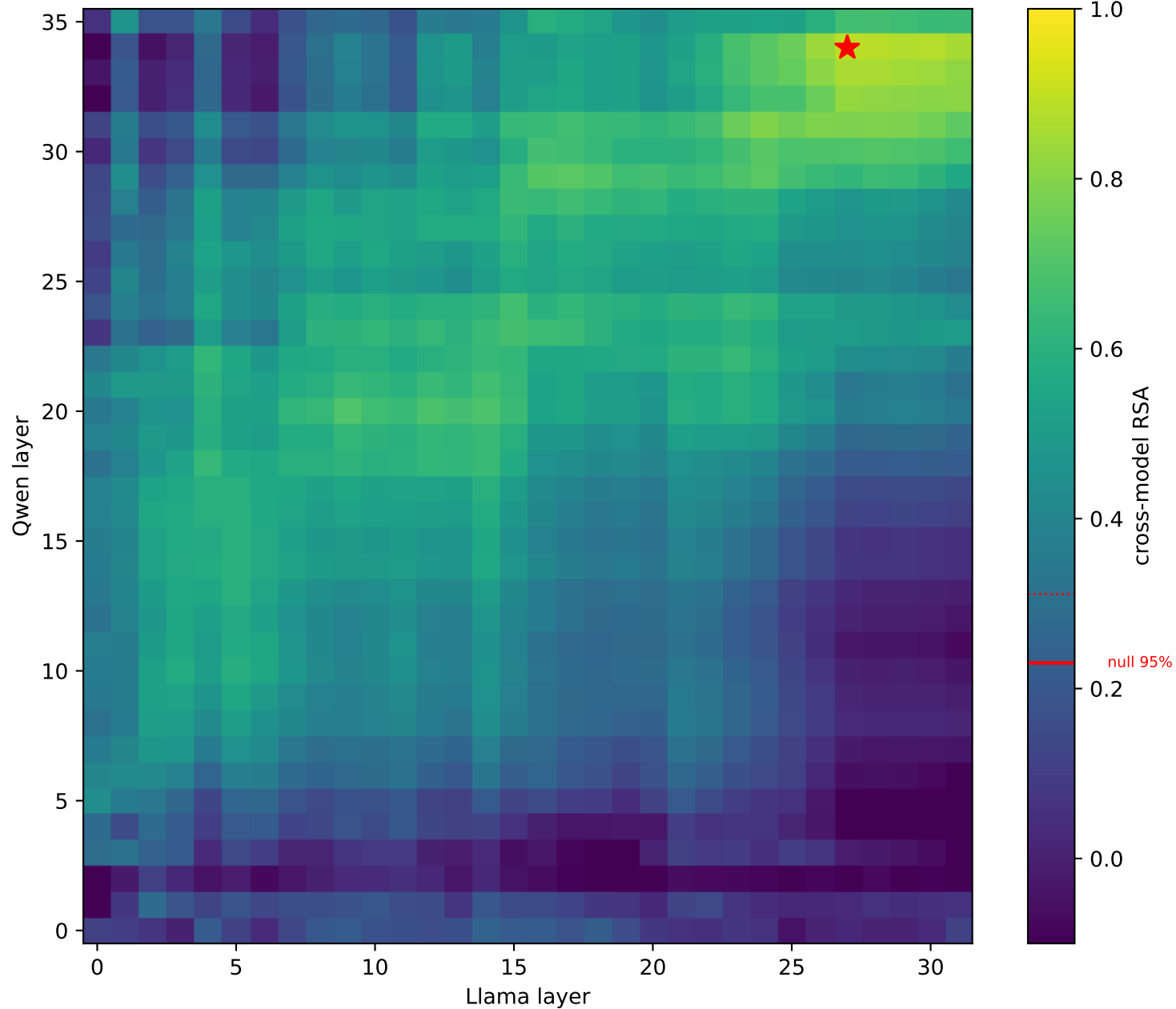
ring (n=16): Qwen vs Llama cross-model RSA (max 0.89; null95=0.23, null99=0.31)
