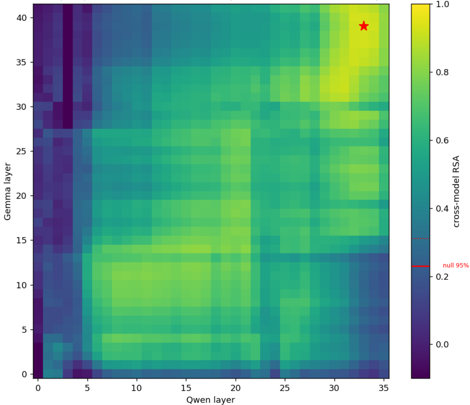
hex (n=16): Gemma vs Qwen cross-model RSA (max 0.93; null95=0.23, null99=0.31)
