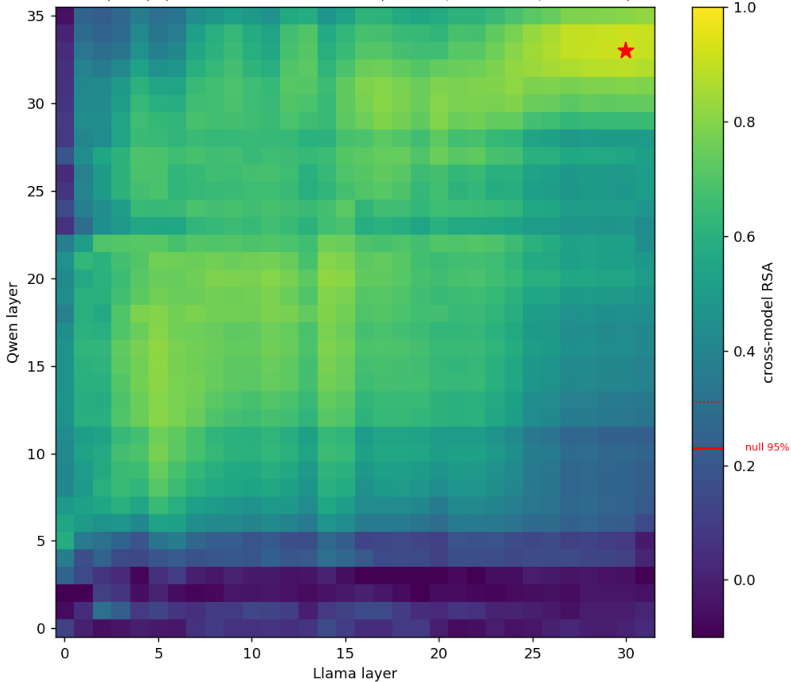
hex (n=16): Qwen vs Llama cross-model RSA (max 0.92; null95=0.23, null99=0.31)
