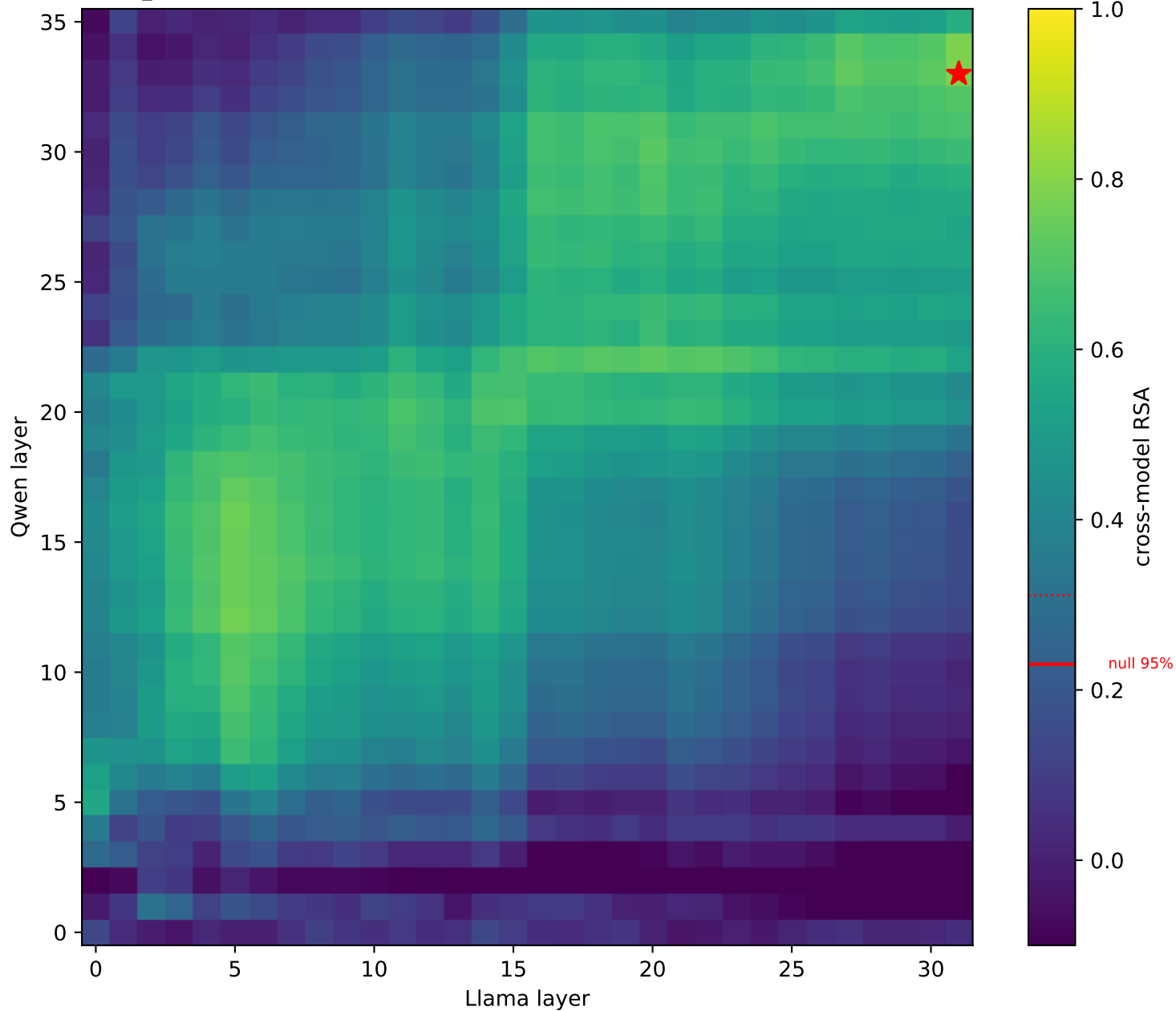
square_grid (n=16): Qwen vs Llama cross-model RSA (max 0.79; null95=0.23, null99=0.31)
