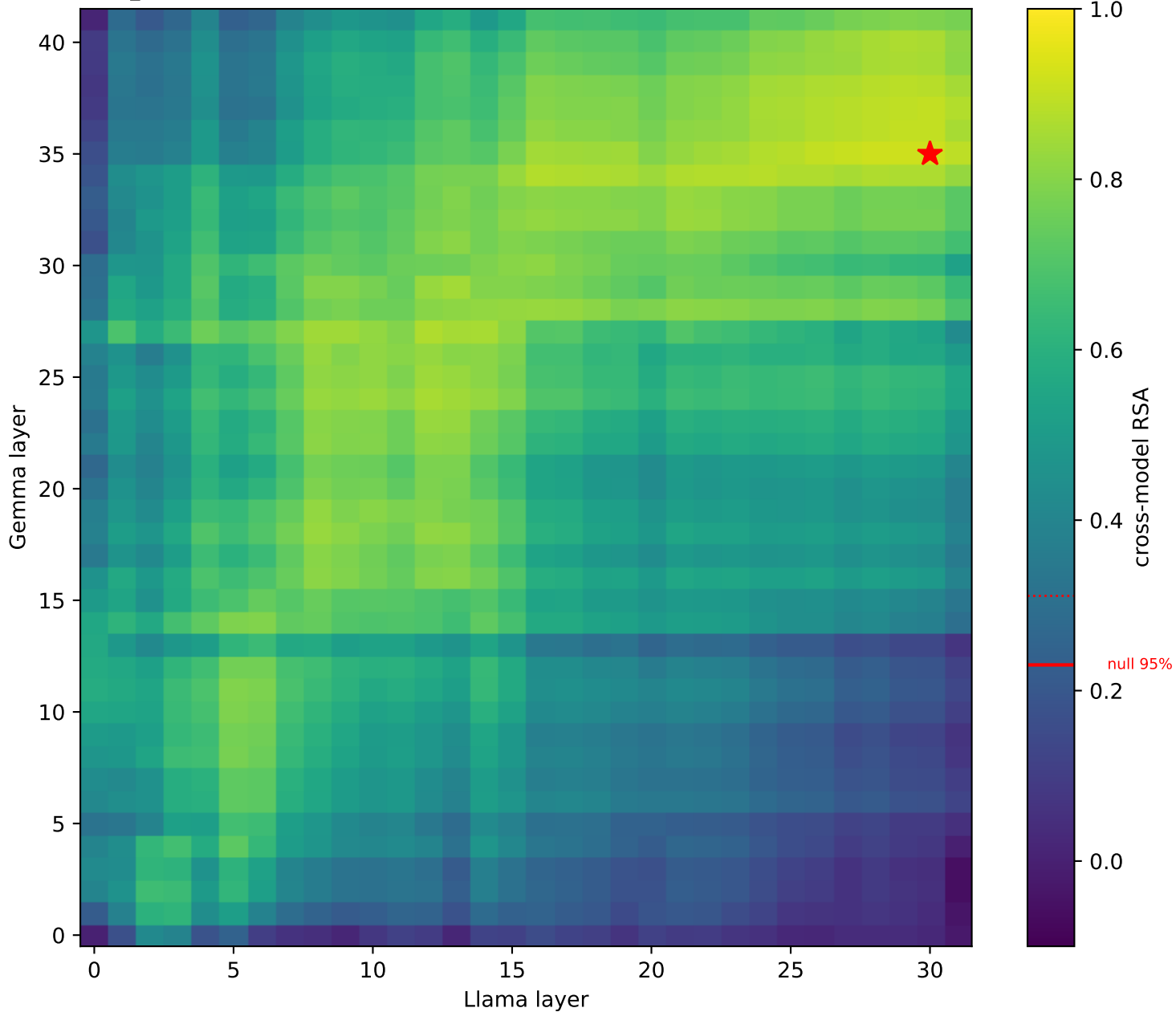
square_grid (n=16): Gemma vs Llama cross-model RSA (max 0.92; null95=0.23, null99=0.31)
