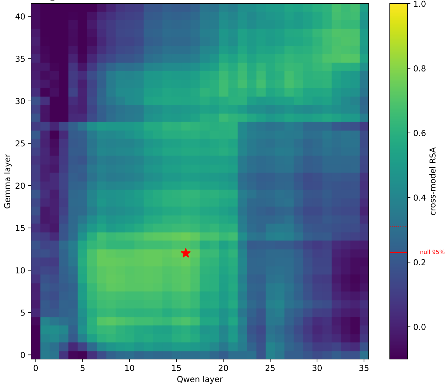
square_grid (n=16): Gemma vs Qwen cross-model RSA (max 0.76; null95=0.23, null99=0.31)
