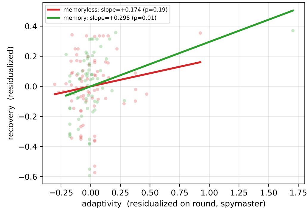
(c) spymaster→guesser partial effect (recovery on adaptivity, round controlled)
