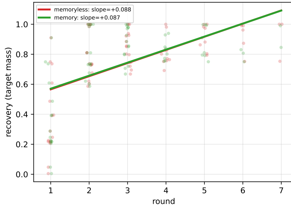
(b) Guesser recovery vs round
