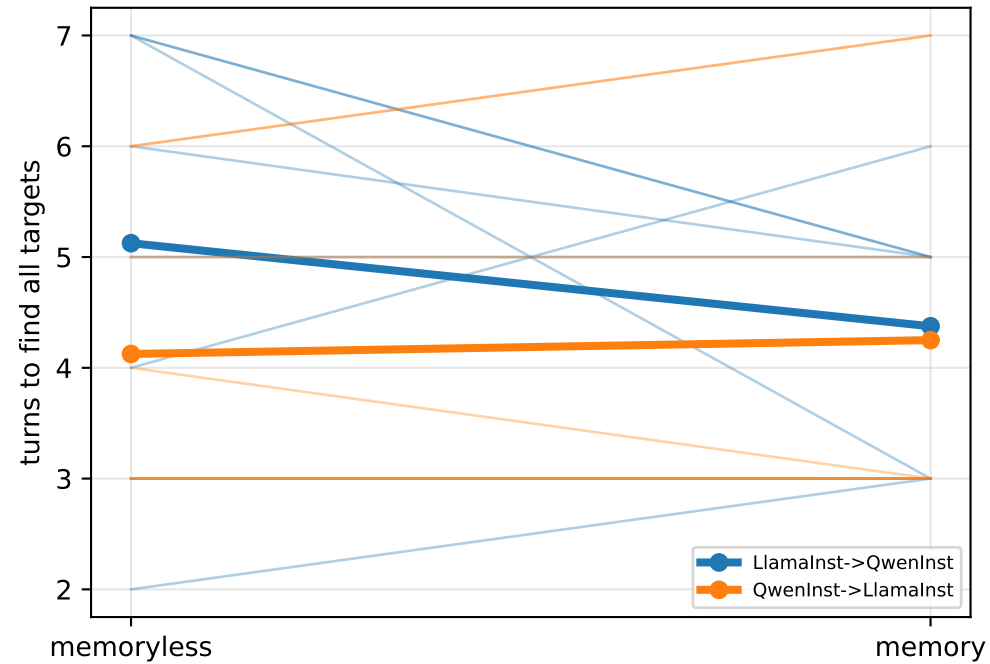
(a) Efficiency: paired per game
