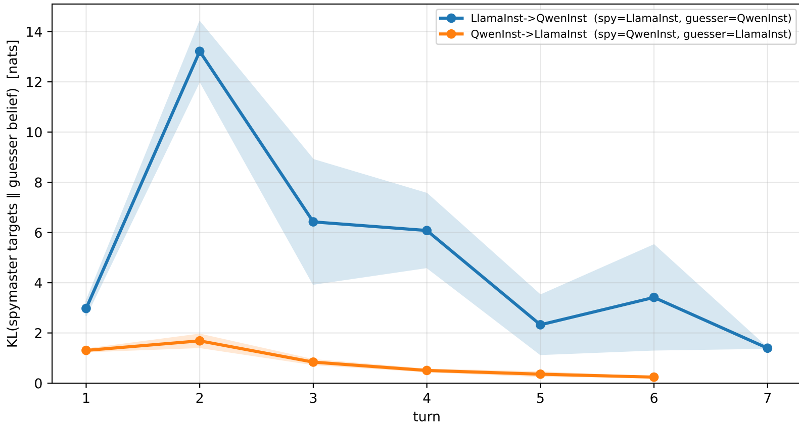
KL between spymaster and guesser over turns (lower = the two minds more aligned; mean over games \pm SE)
