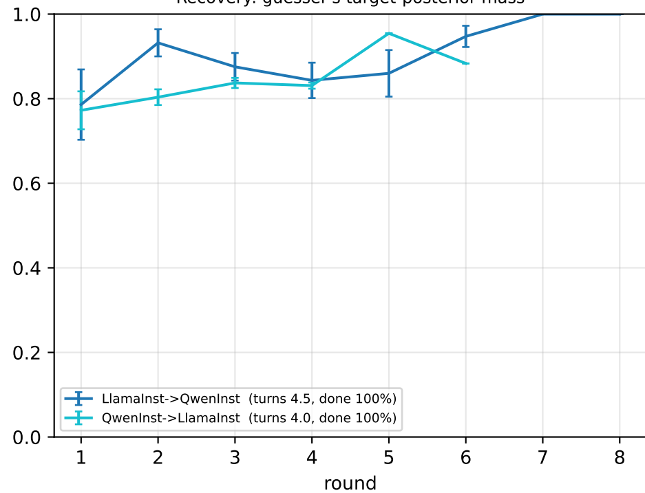
Recovery: guesser's target-posterior mass
