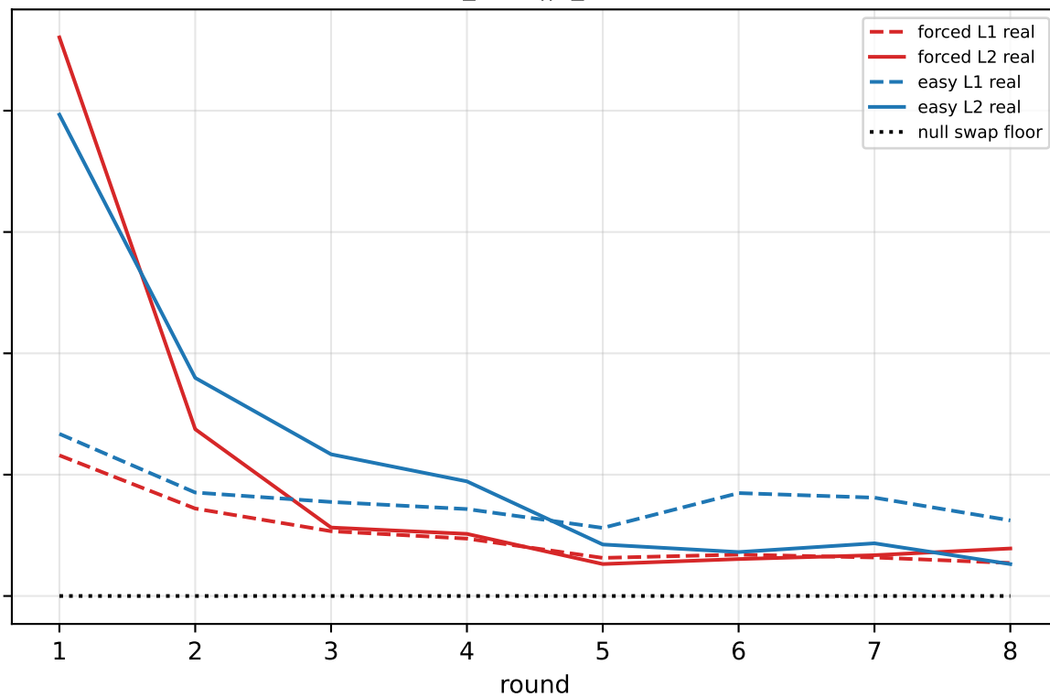
Coupling: KL(B_{\text{swap}}||B_{\text{clean}}) per round
