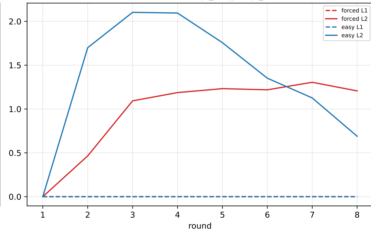
A's adaptivity: KL(\text{clue}|B_{\text{real}}||\text{clue}|B_{\text{naive}})
