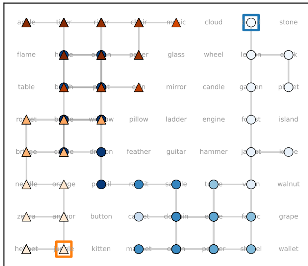
game 7: no-meet (120 r)
