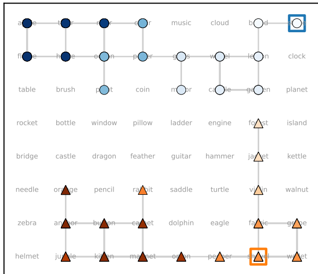
game 5: no-meet (120 r)
