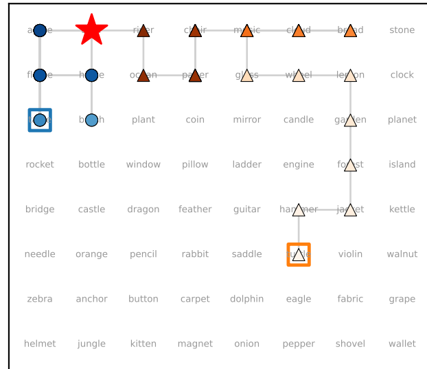
game 3: MET @r38
