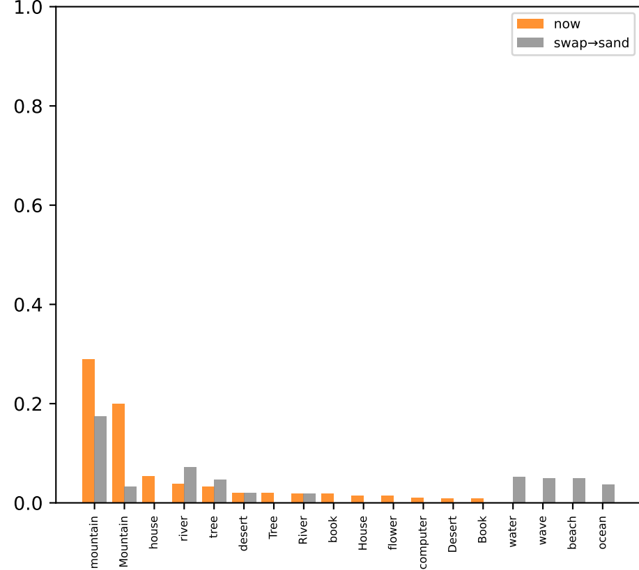
LlamaInst#2: mountain KL=1.13
