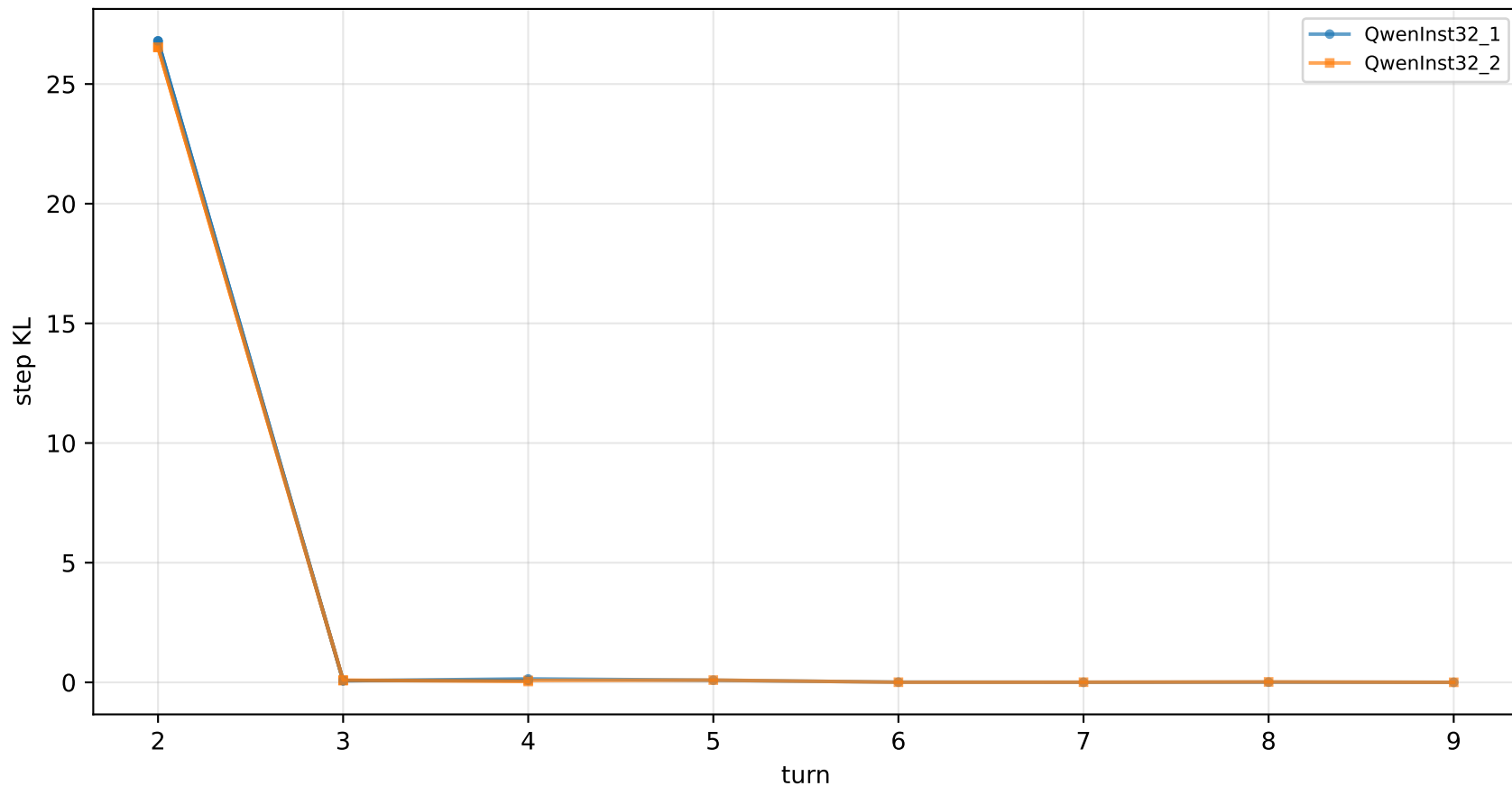
step KL every turn, every game (3 games) — game1open_llm_QwenInst32_1_vs_QwenInst32_2_transcript_stepkl_allturns.pdf
