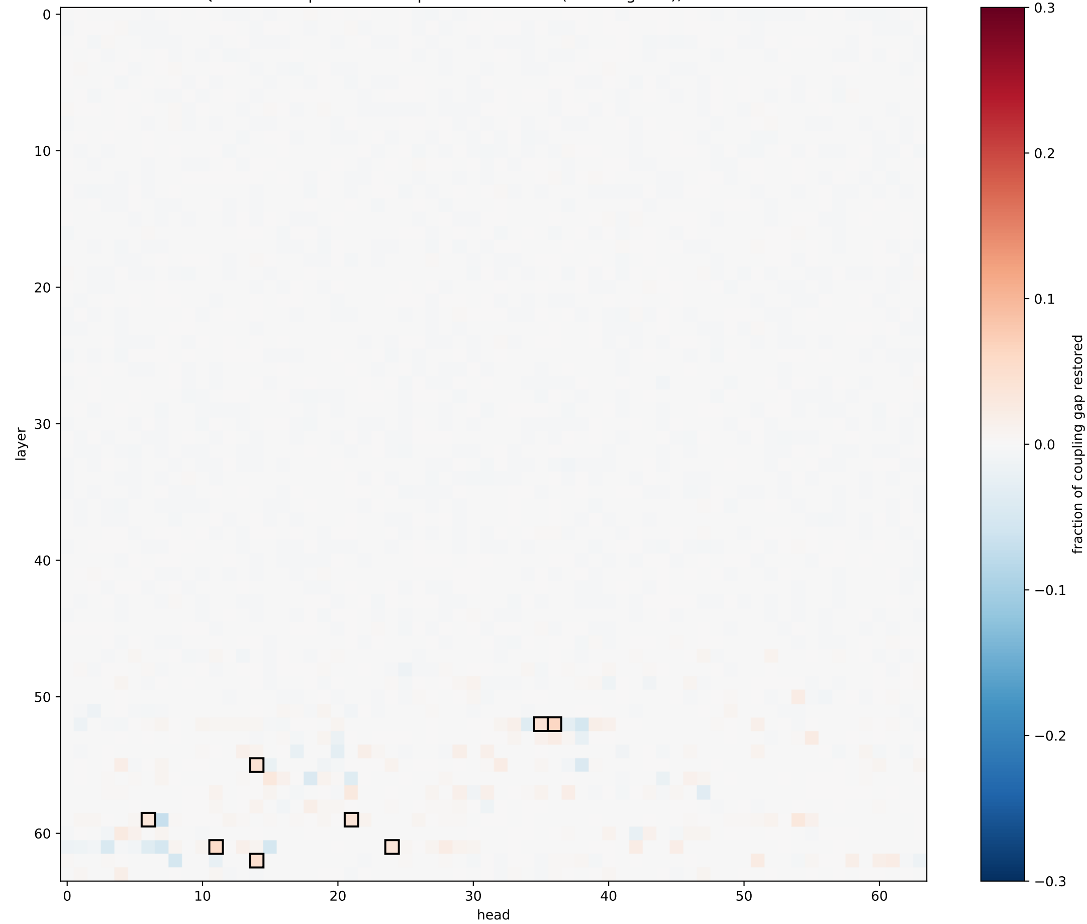
QwenInst32: partner-word patch restoration (real vs ghost), n=24 states
