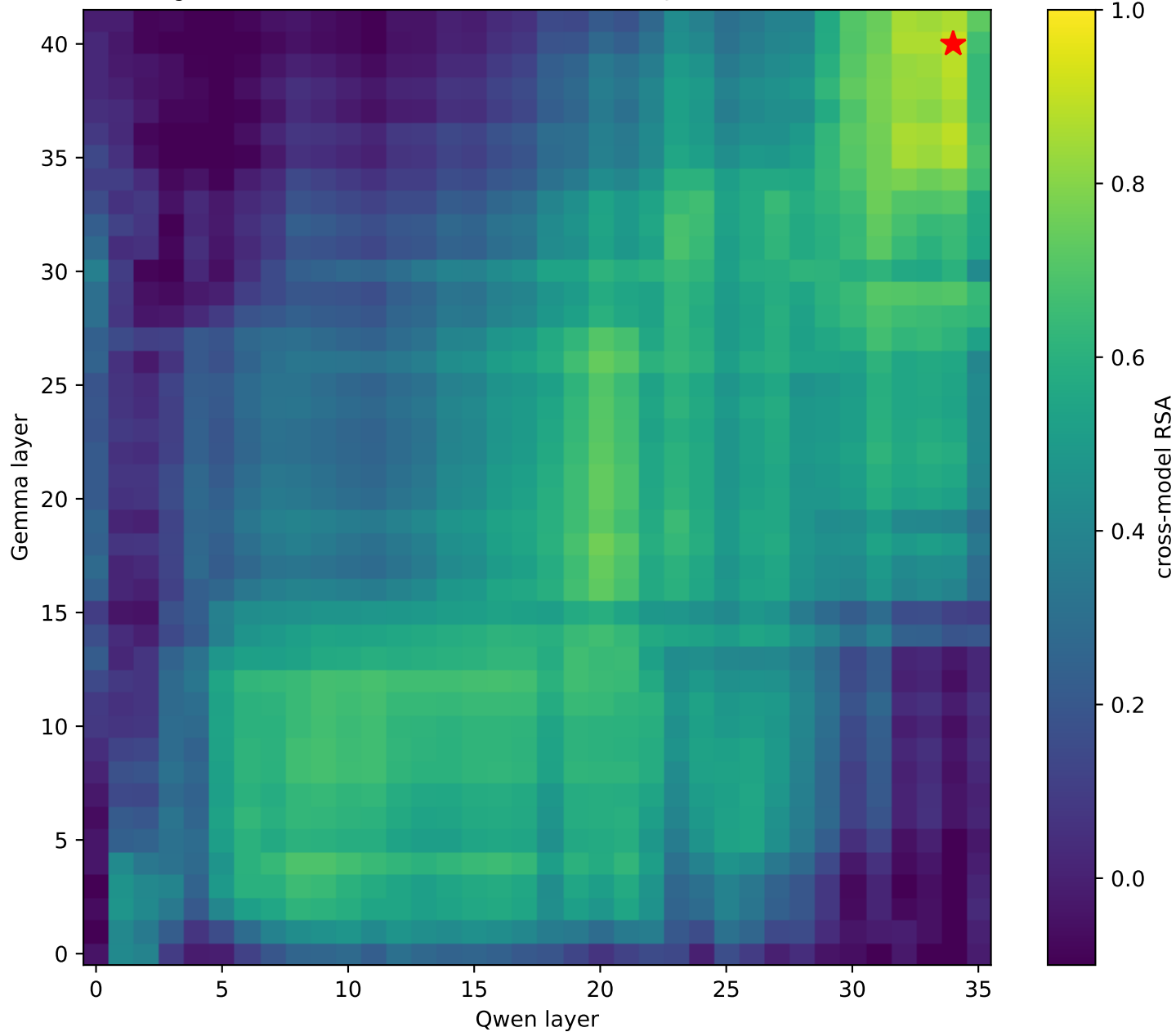
ring: Gemma vs Qwen cross-model RSA (max 0.91 @ Gemma L40 / Qwen L34)
