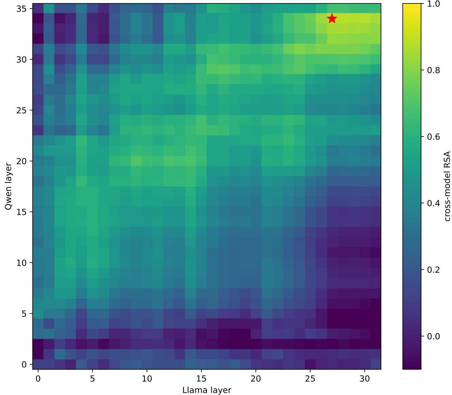
ring: Qwen vs Llama cross-model RSA (max 0.89 @ Qwen L34 / Llama L27)
