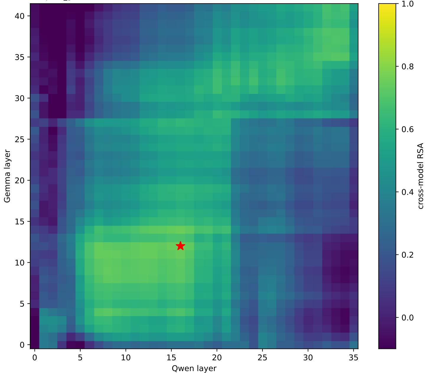
square_grid: Gemma vs Qwen cross-model RSA (max 0.76 @ Gemma L12 / Qwen L16)
