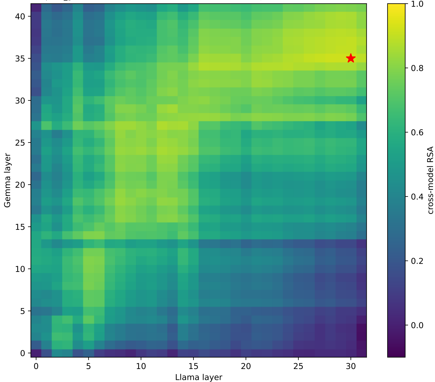
square_grid: Gemma vs Llama cross-model RSA (max 0.92 @ Gemma L35 / Llama L30)
