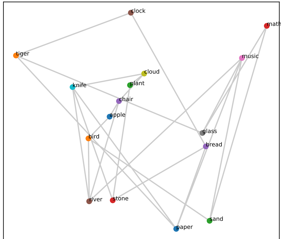
Qwen L14 (RSA=0.19)
