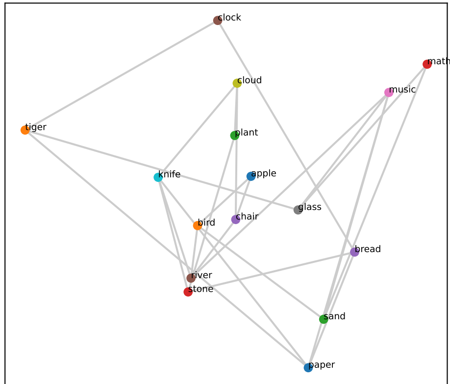
Qwen L9 (RSA=0.10)
