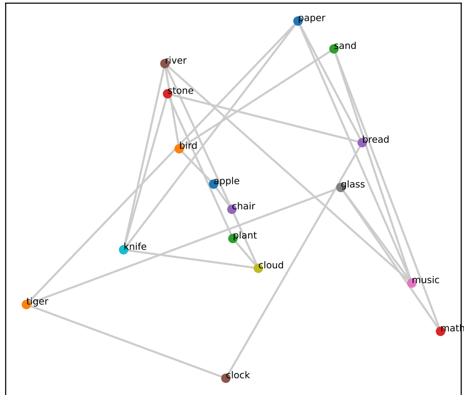
Qwen L15 (RSA=0.18)
