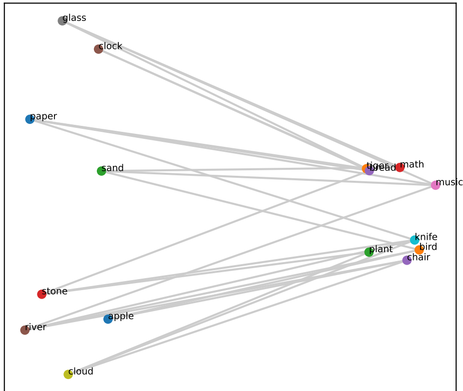
Qwen L33 (RSA=0.17)
