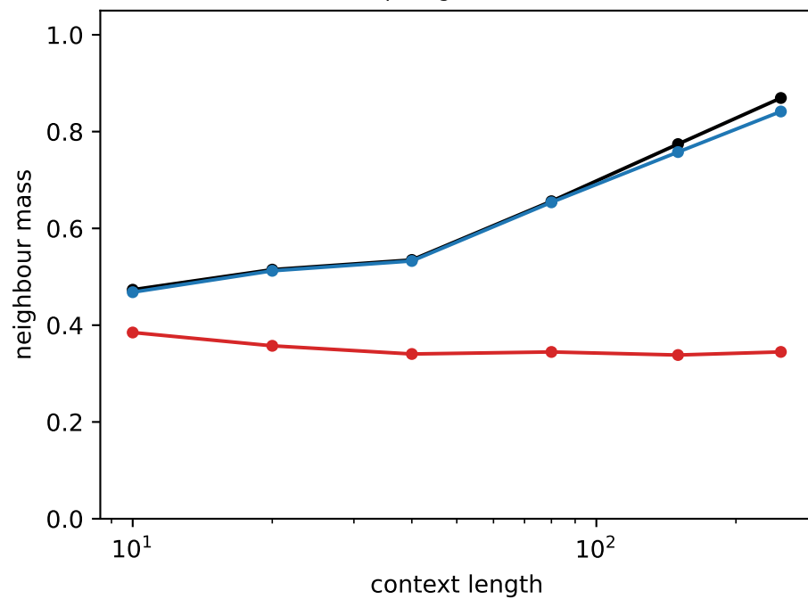
Llama next-step neighbour mass vs context
