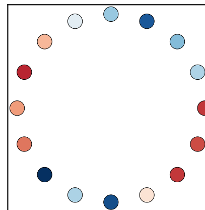
PC2 (9%) \approx checkerboard (parity)
