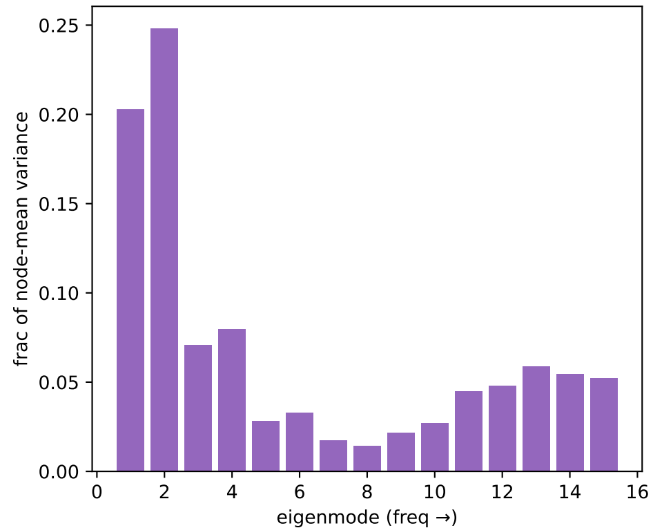
Gemma ring L40: power per Laplacian mode
