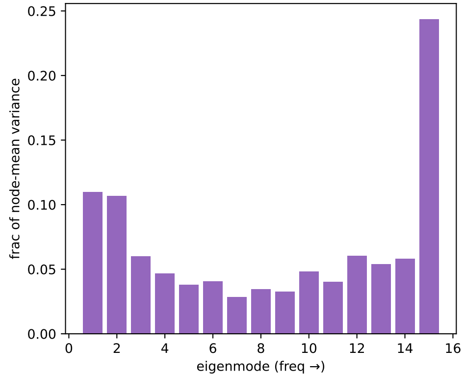
Qwen square_grid L34: power per Laplacian mode
