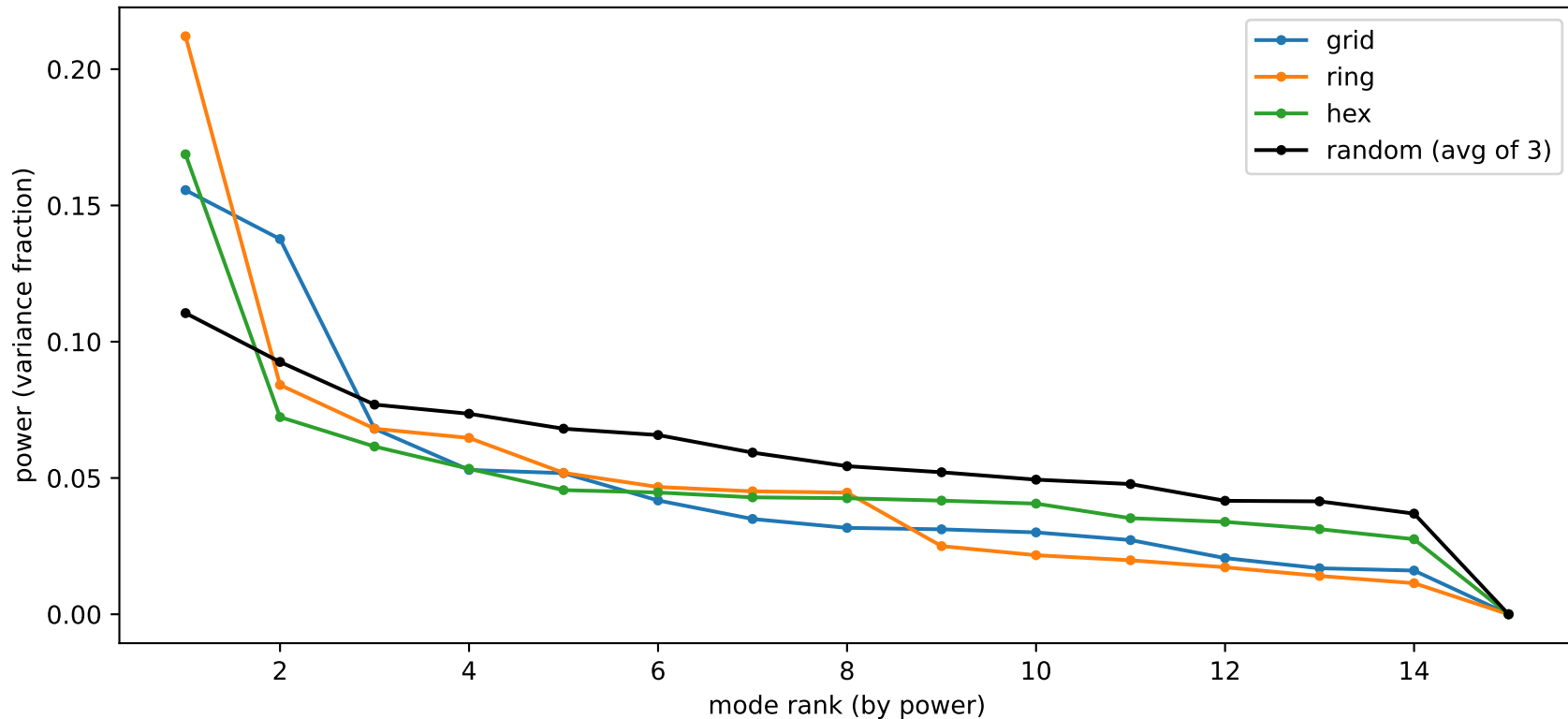
What the model concentrates on, by topology: sorted Laplacian power spectrum geometric graphs spike on a few coarse modes; random is flat/diffuse
