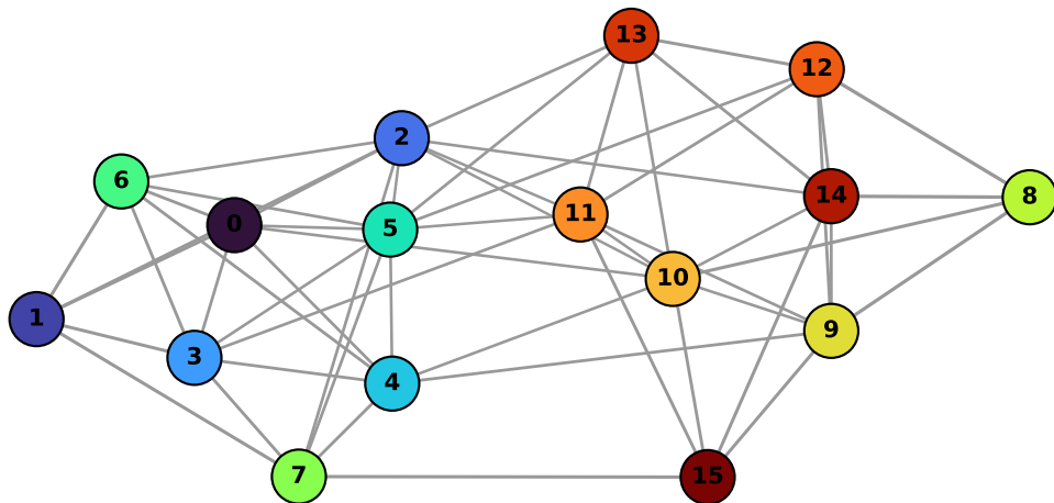
sbm2: the Markov chain 16 states, 54 transitions, mean degree 6.8
