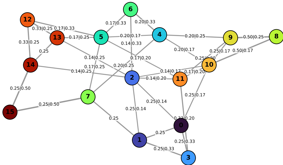
sbm4: the Markov chain 16 states, 33 transitions, mean degree 4.1
