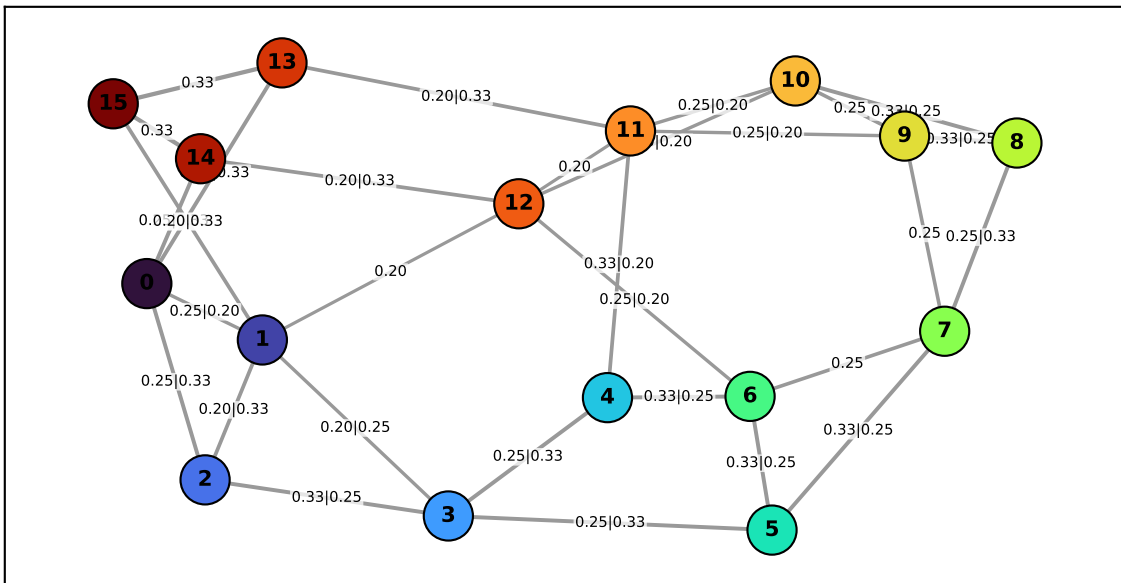
smallworld: the Markov chain 16 states, 30 transitions, mean degree 3.8
