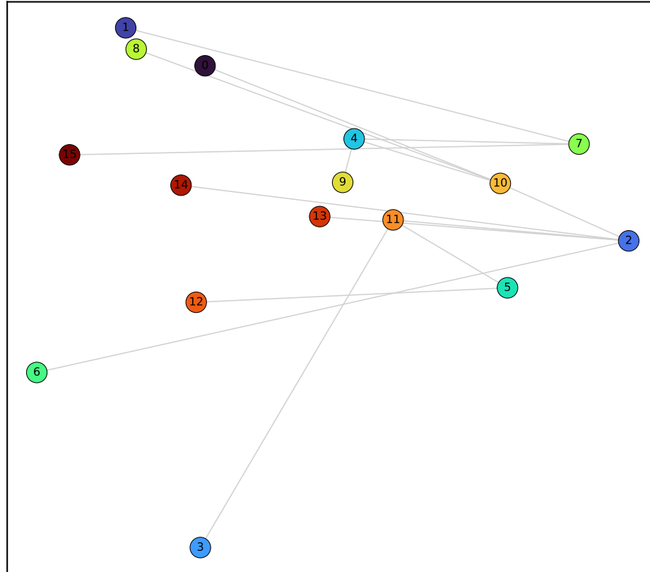
Gemma layer 14/41 (PC var 14.11%)
