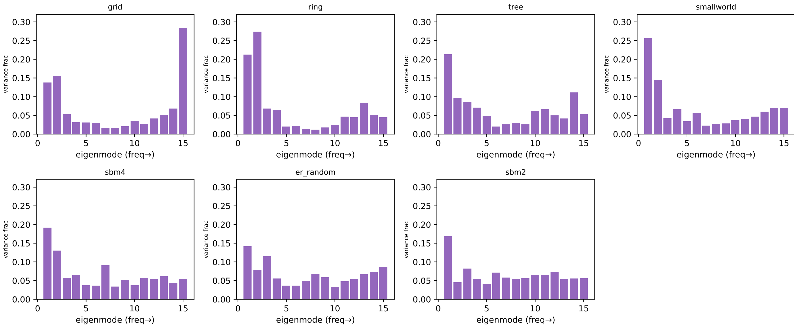
Llama: node-mean variance vs Laplacian eigenmode, per family
