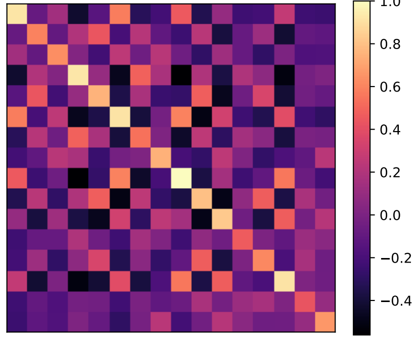
grid: representation Gram G=HcHc^T
