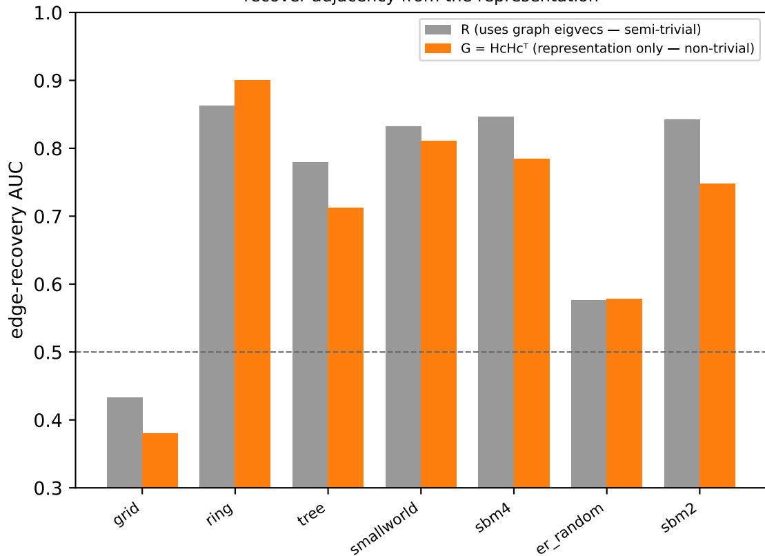
recover adjacency from the representation
