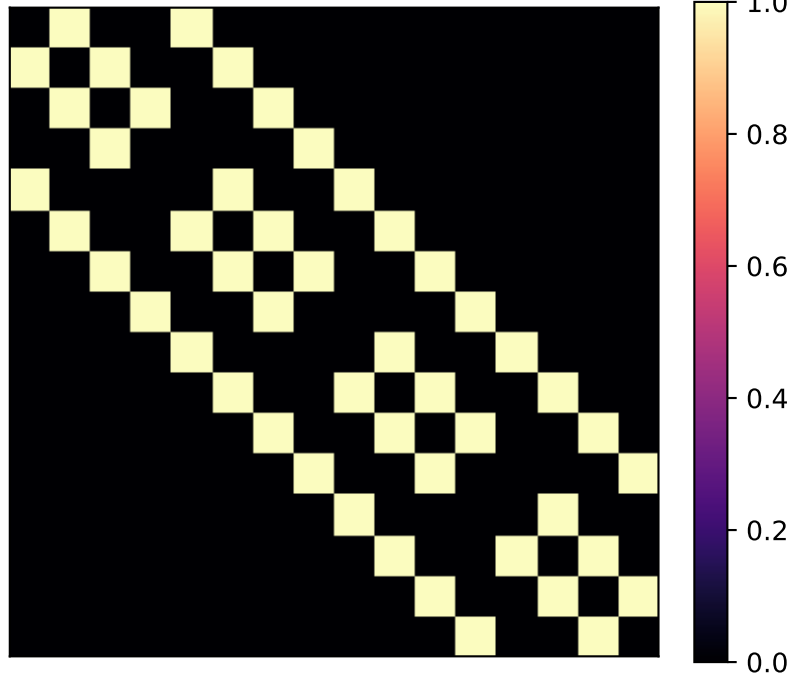
grid: adjacency A
