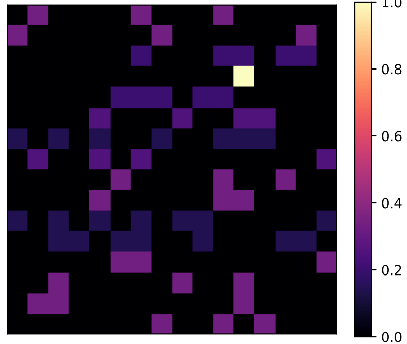
er_random: transition T
