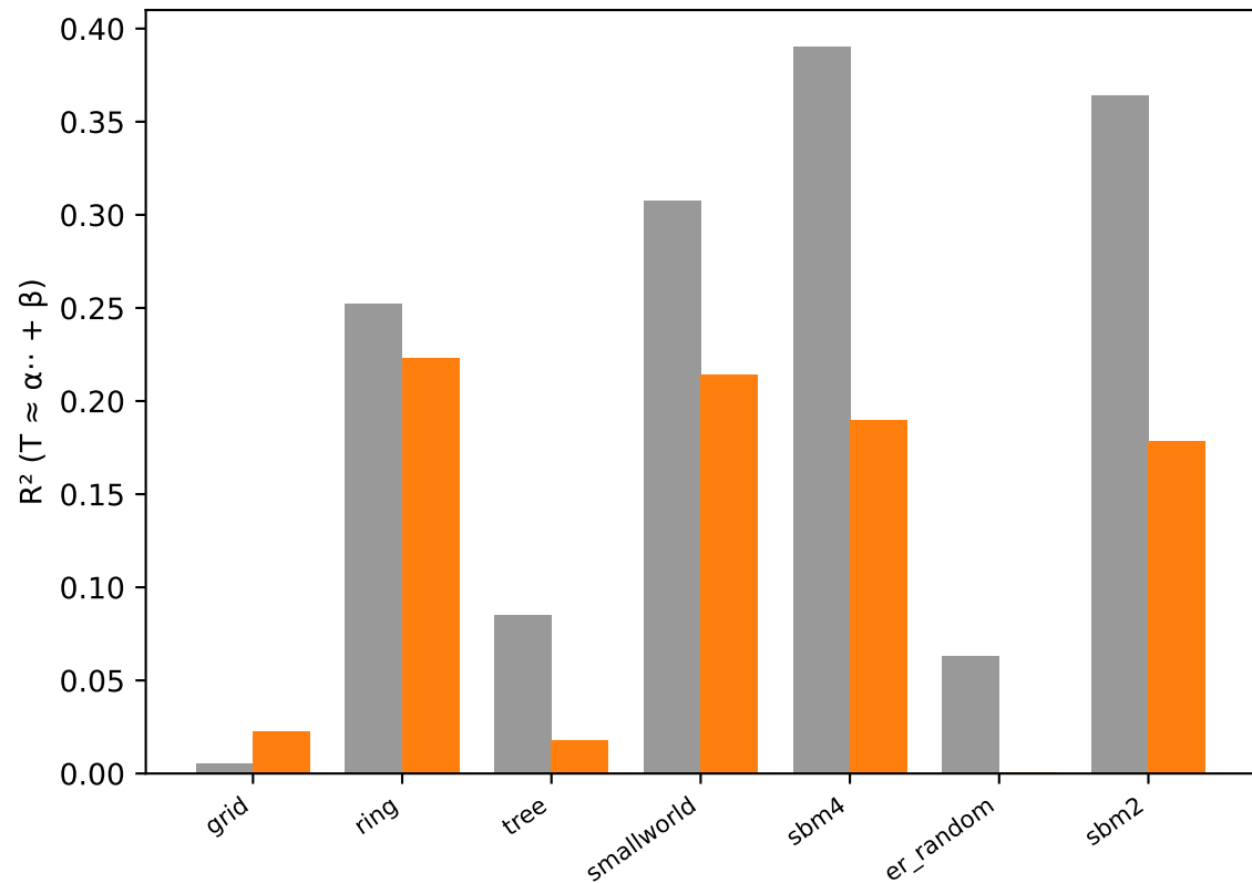
linear fit of transition matrix
