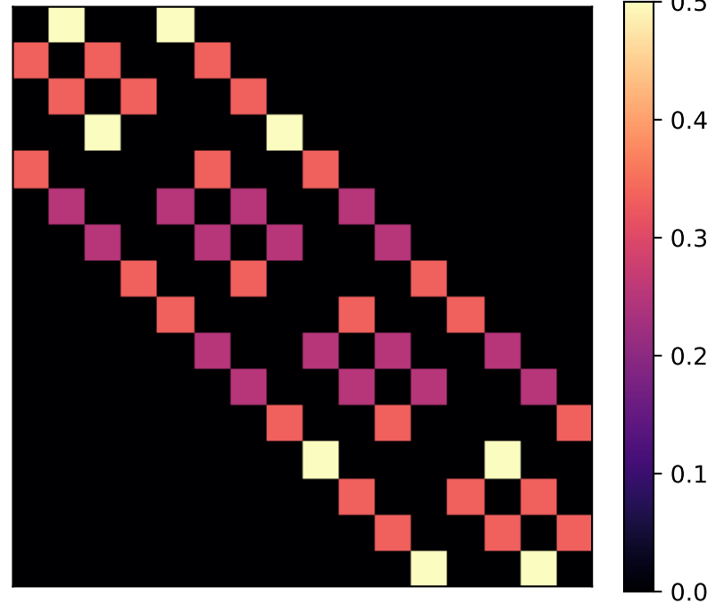
grid: transition T
