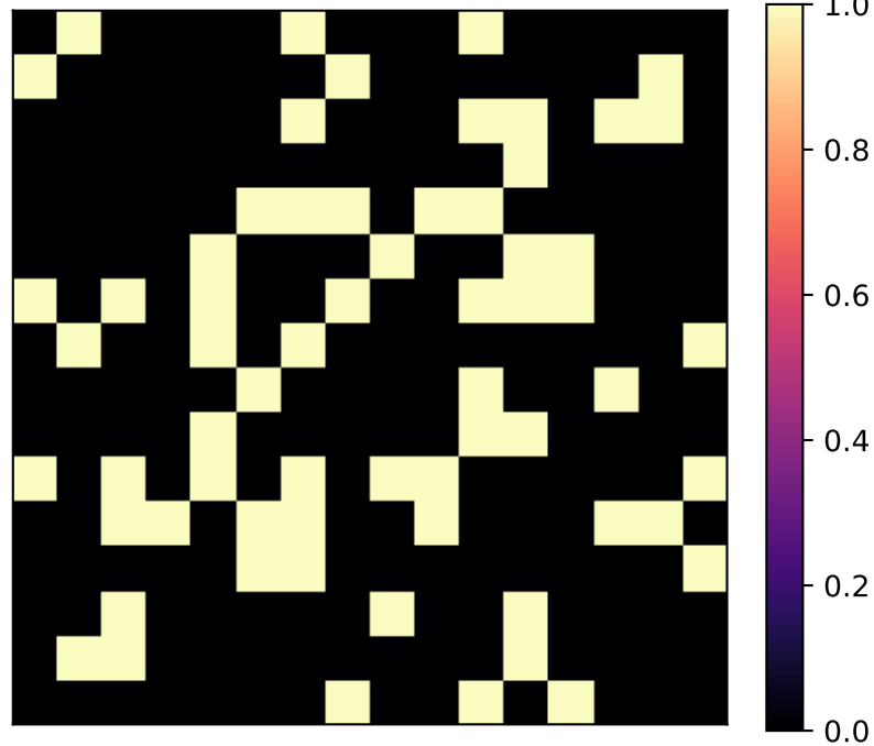
er_random: adjacency A
