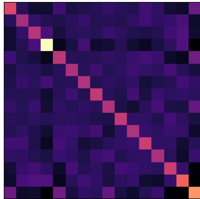
er_random: representation Gram G=HcHc^T
