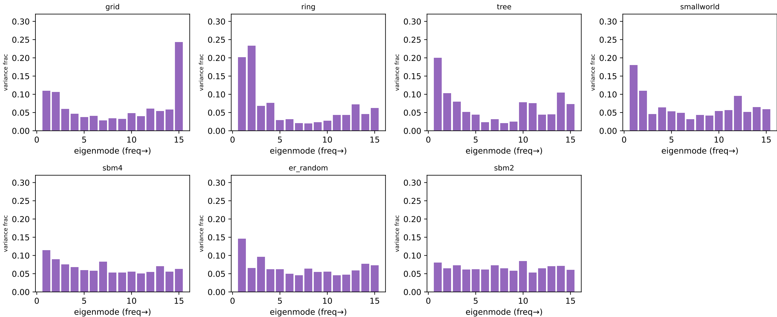
Qwen: node-mean variance vs Laplacian eigenmode, per family
