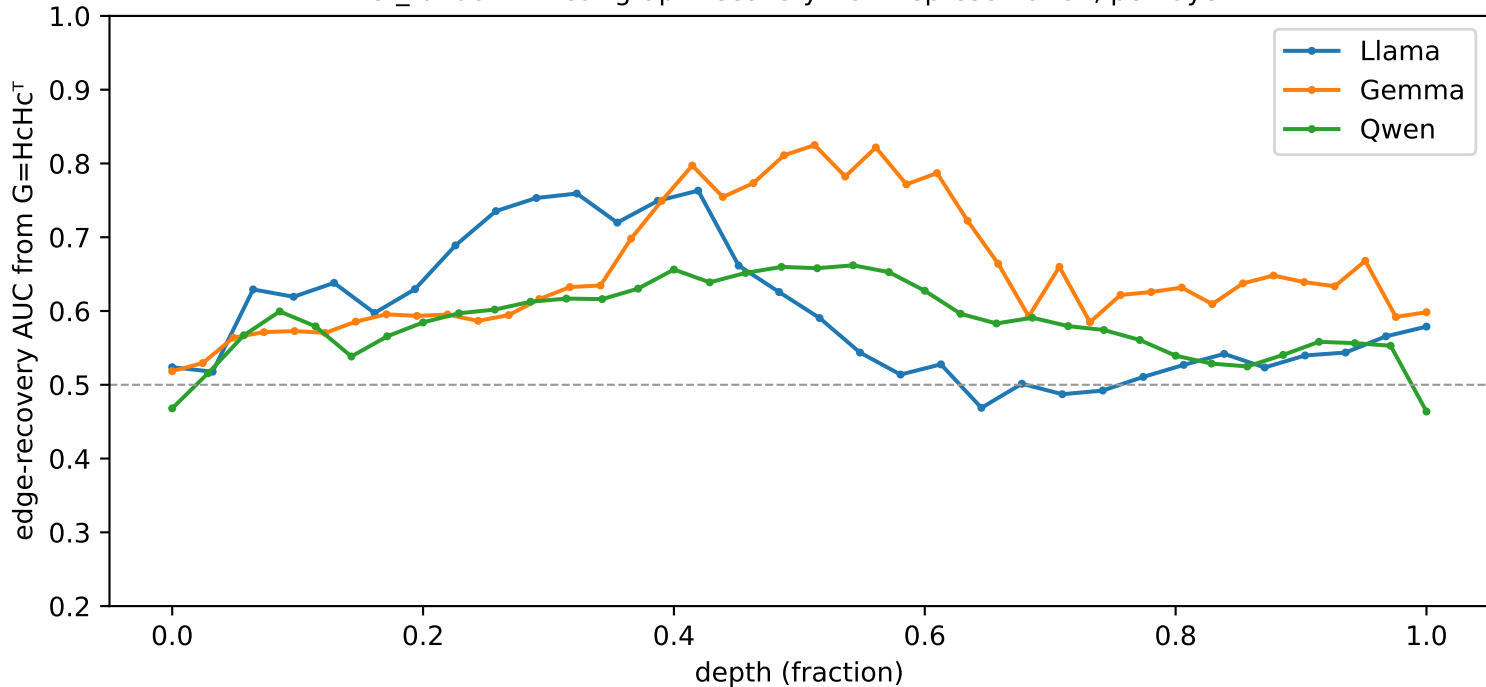
er_random: linear graph-recovery from representation, per layer
