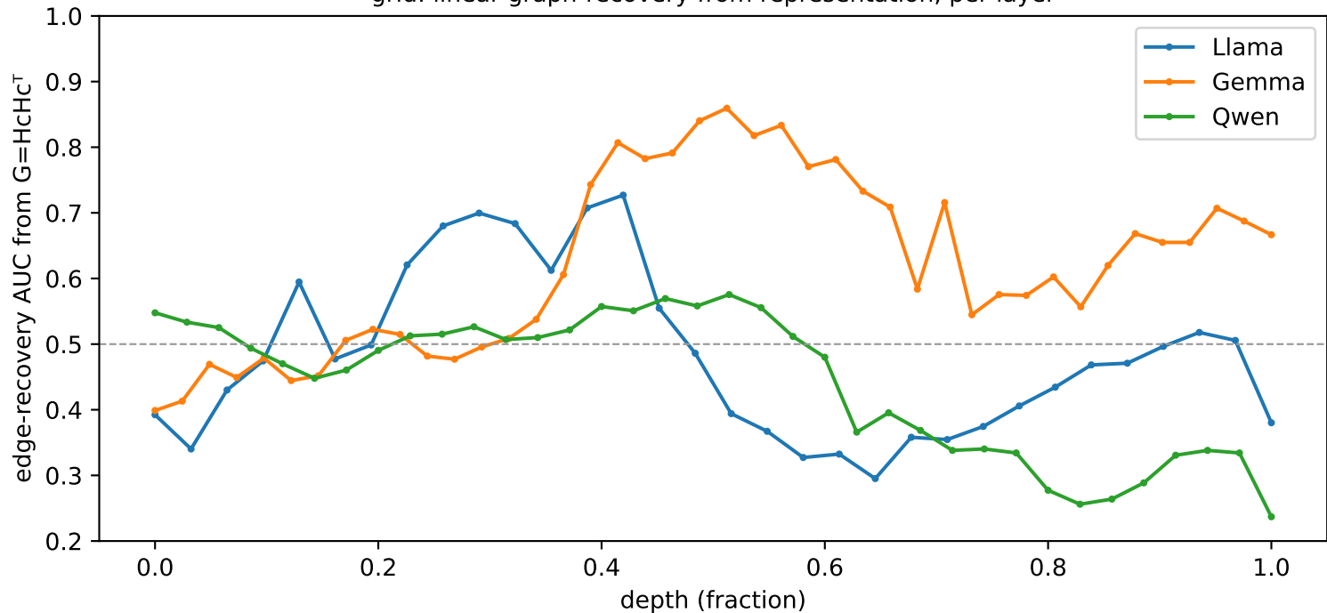
grid: linear graph-recovery from representation, per layer
