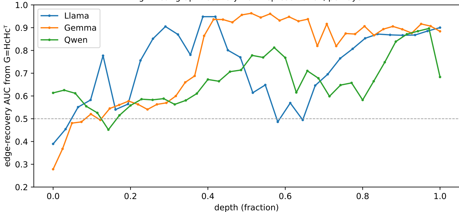
ring: linear graph-recovery from representation, per layer
