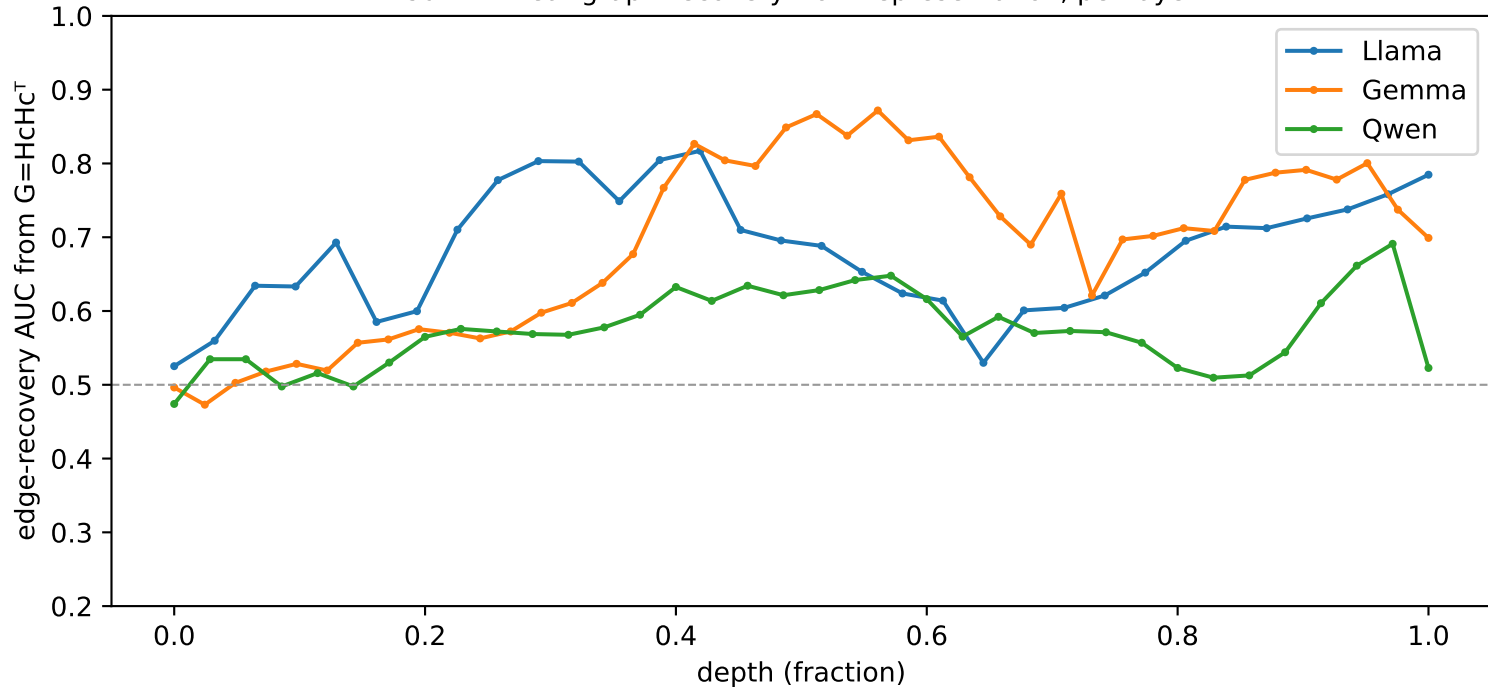
sbm4: linear graph-recovery from representation, per layer
