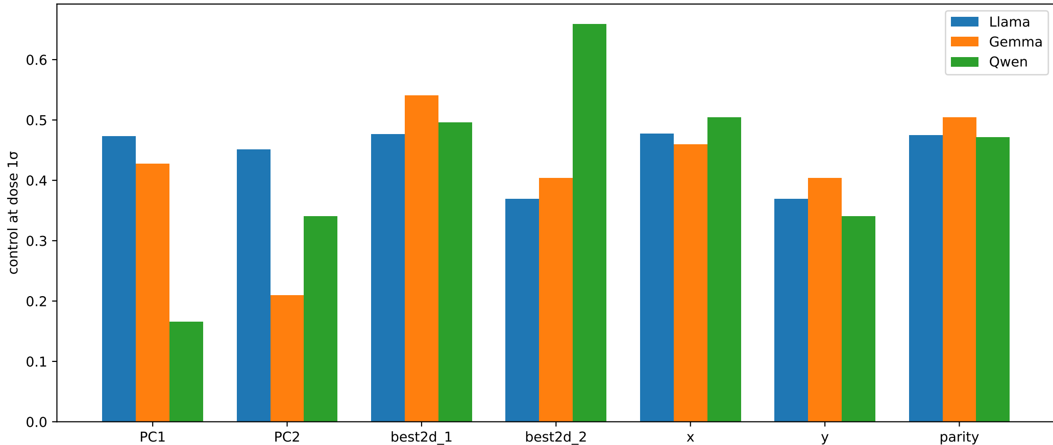
steerability at 1\sigma : data-driven directions vs graph cuts
