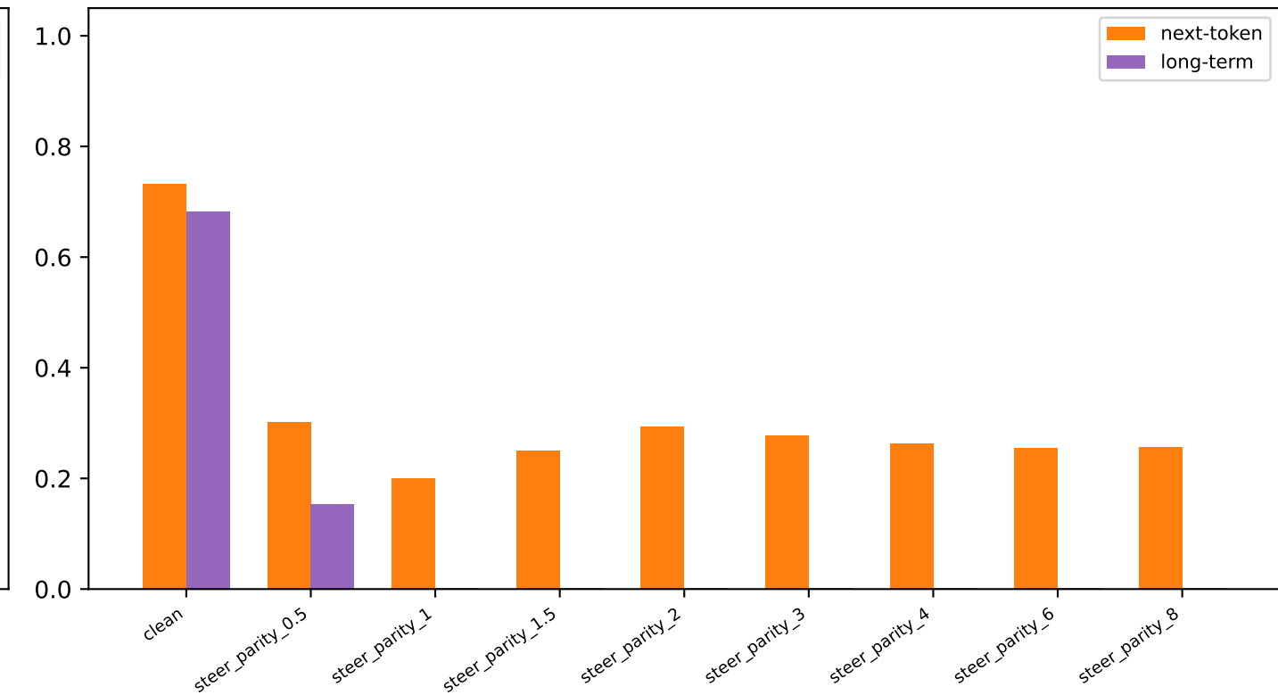
neighbour mass: next-token vs long-term
