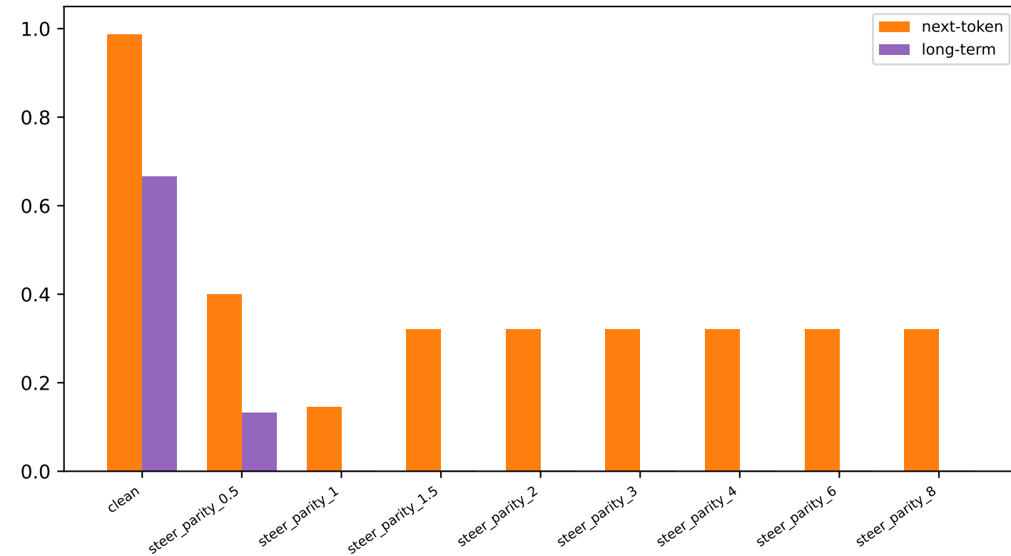
validity: next-token vs long-term
