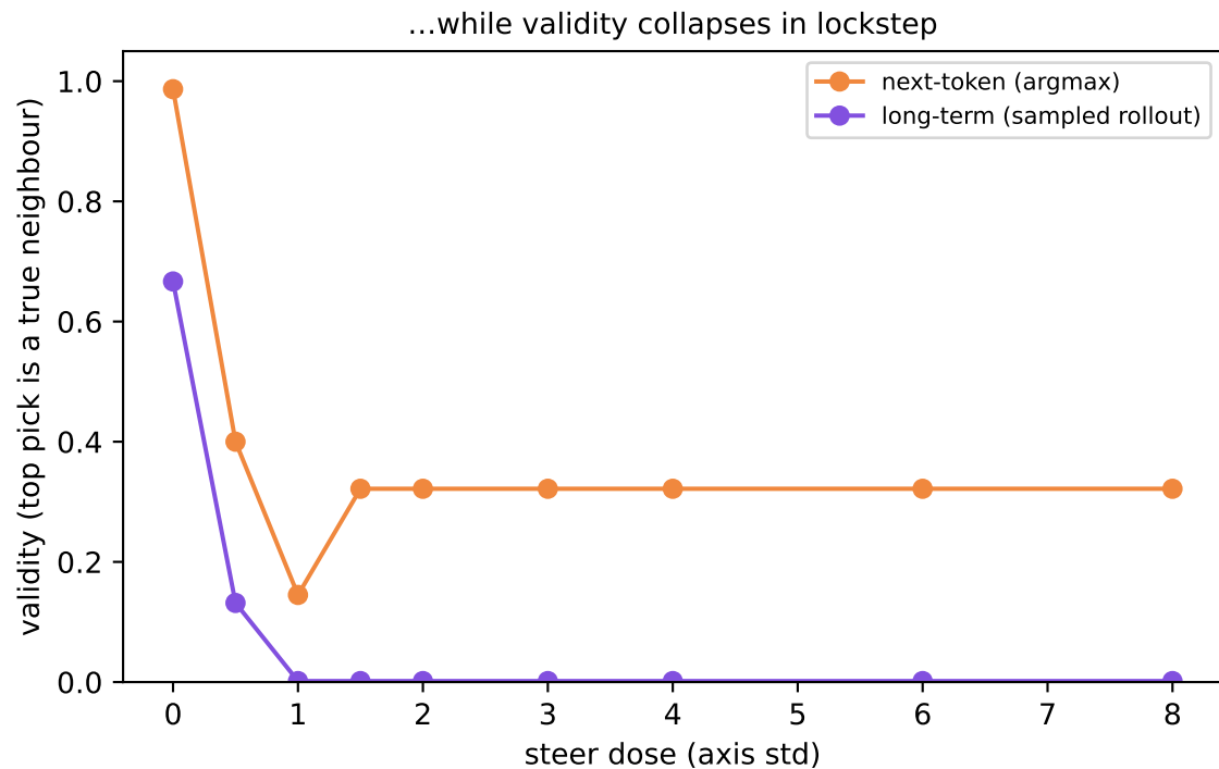
Llama square_grid — steering the parity axis: absolute-sublattice control vs behavioural cost mass = total predicted probability on that node-set (p sums to 1 over the 16 nodes)
