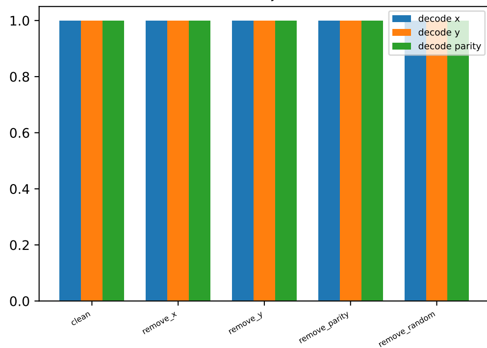
linear decodability after removal
