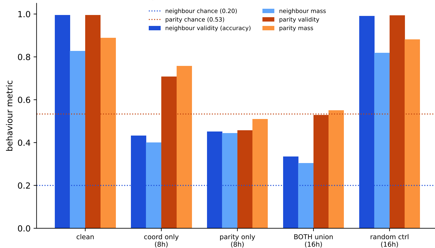
Ablating BOTH circuits vs each alone vs random control
