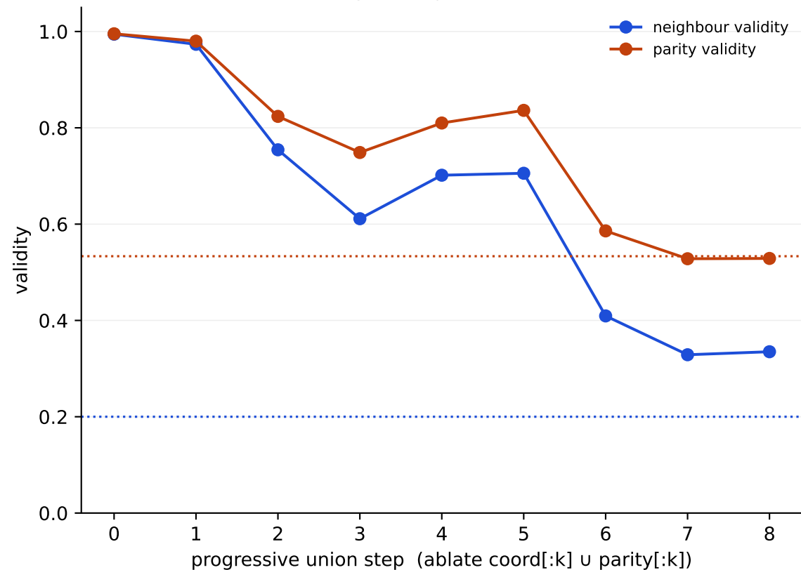
Progressive joint ablation
