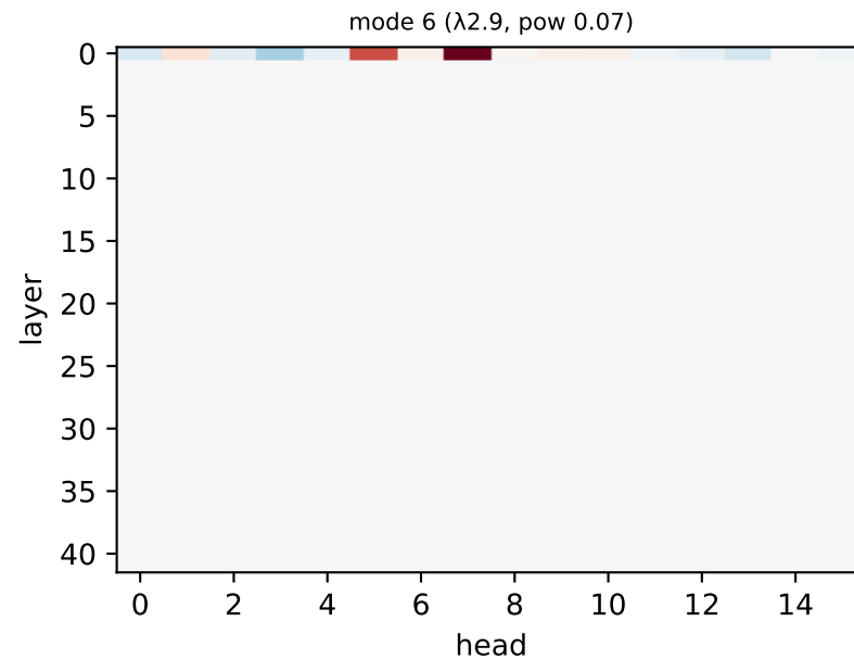
Gemma er_random — single-head damage per eigenmode (red=head builds it)
