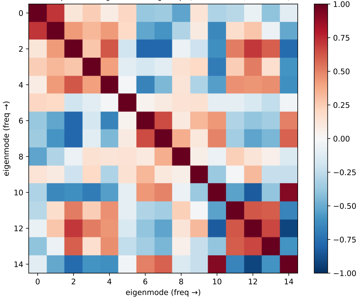
Gemma sbm4 — do eigenmodes share head circuits? corr of per-mode single-head damage maps (1=same heads, 0=different)
