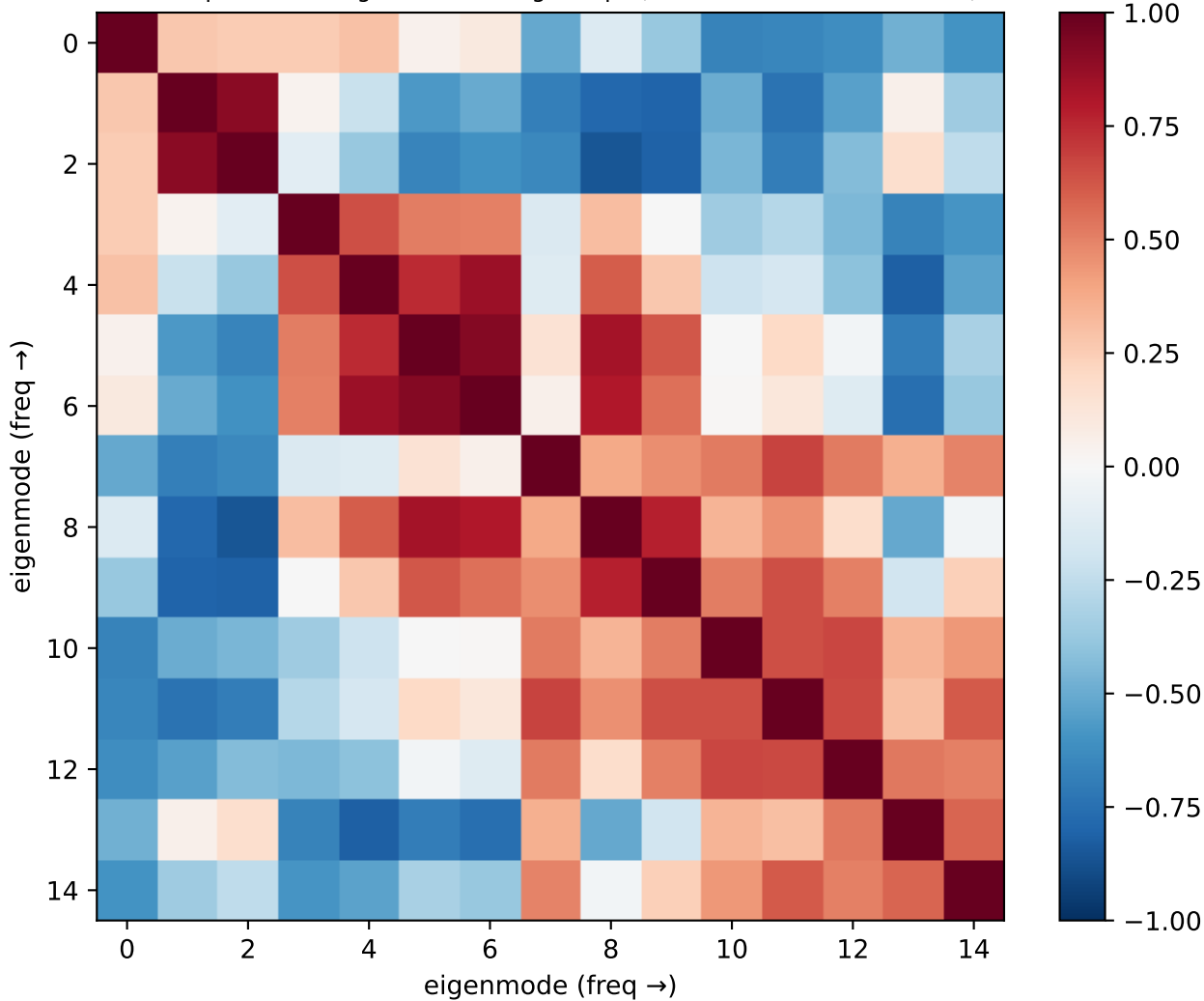
Llama er_random — do eigenmodes share head circuits? corr of per-mode single-head damage maps (1=same heads, 0=different)
