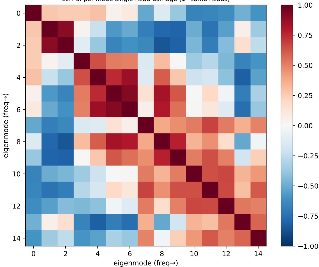
er_random: eigenmode circuit overlap (all 15 modes) corr of per-mode single-head damage (1=same heads)
