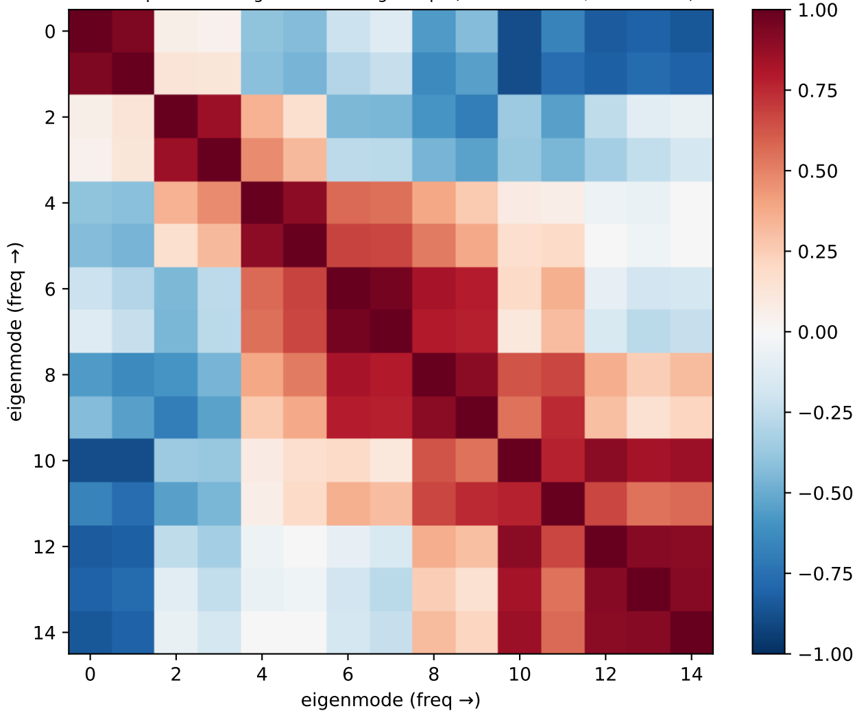
Llama ring — do eigenmodes share head circuits? corr of per-mode single-head damage maps (1=same heads, 0=different)
