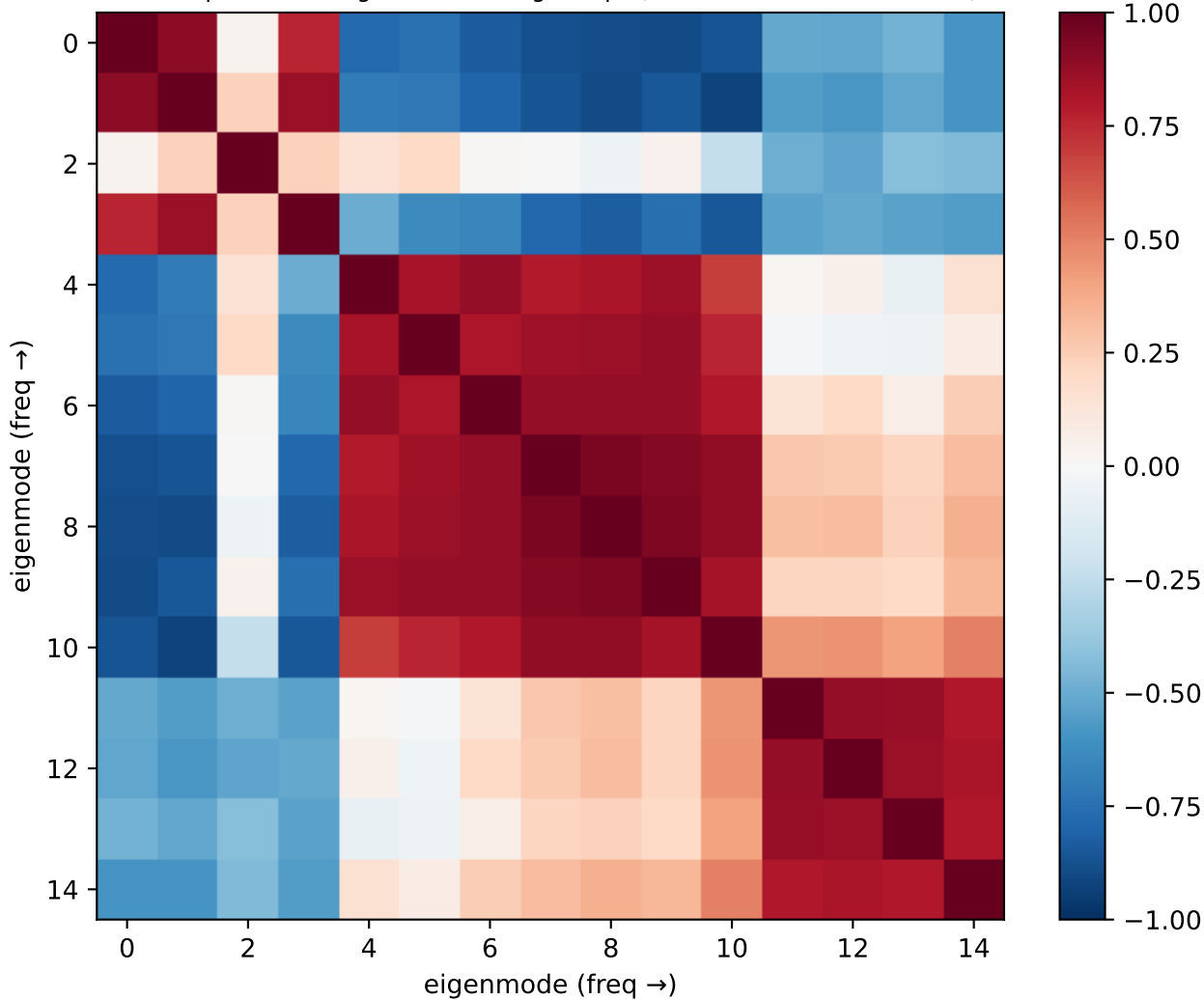
Llama sbm4 — do eigenmodes share head circuits? corr of per-mode single-head damage maps (1=same heads, 0=different)
