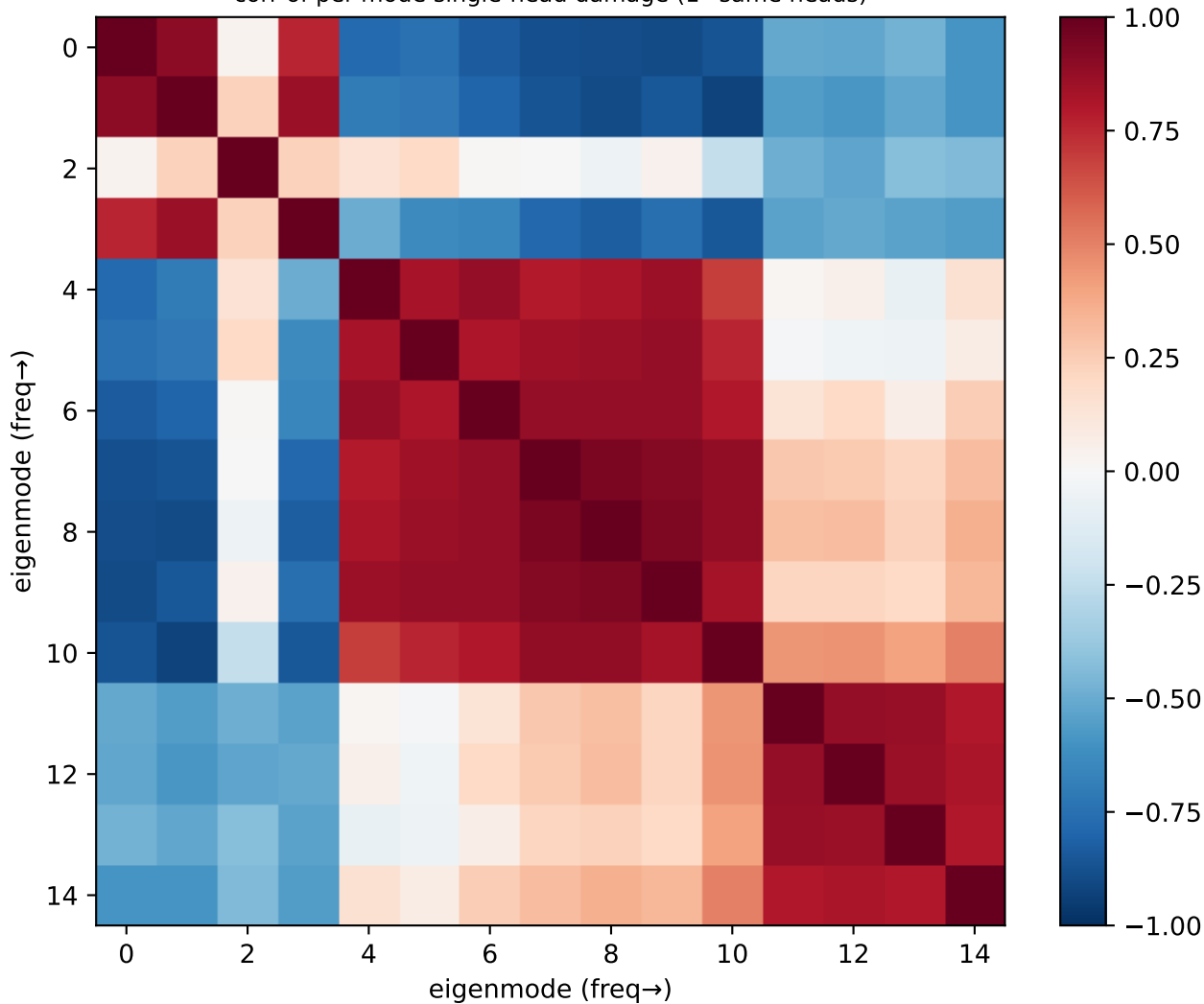
sbm4: eigenmode circuit overlap (all 15 modes) corr of per-mode single-head damage (1=same heads)
