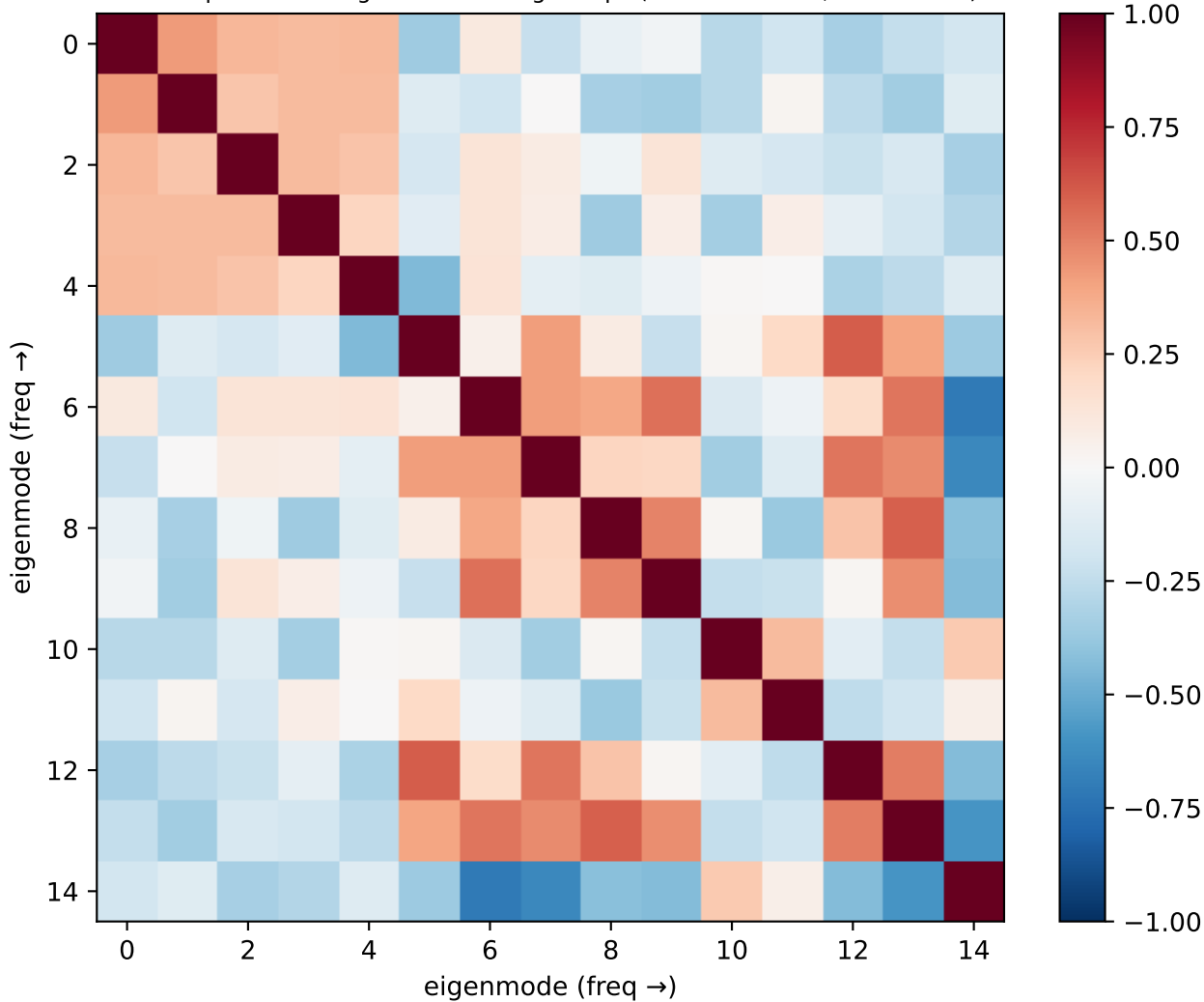
Qwen grid — do eigenmodes share head circuits? corr of per-mode single-head damage maps (1=same heads, 0=different)
