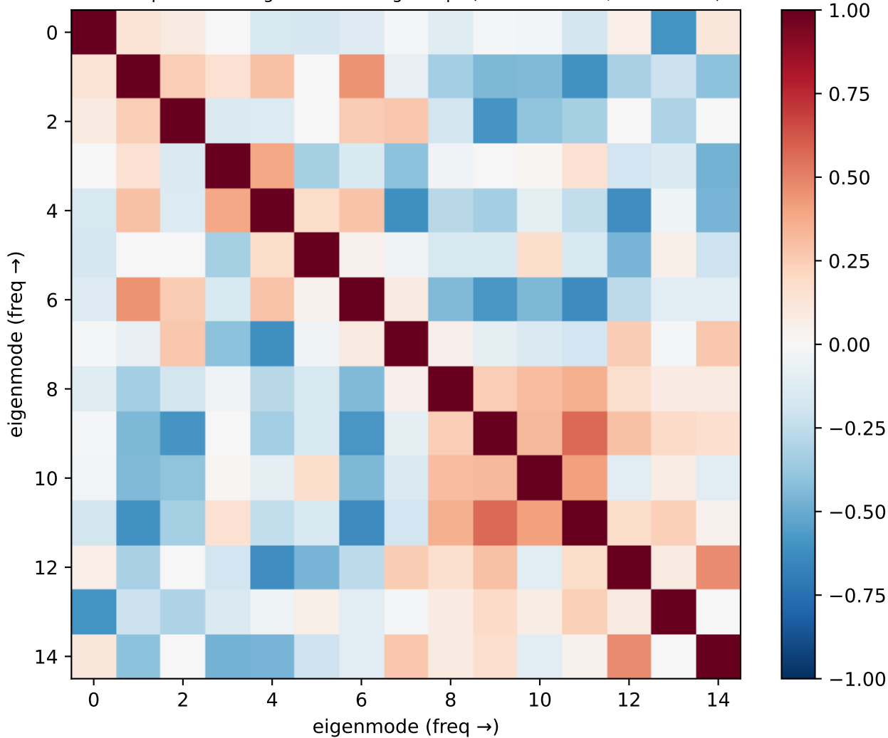
Qwen sbm4 — do eigenmodes share head circuits? corr of per-mode single-head damage maps (1=same heads, 0=different)
