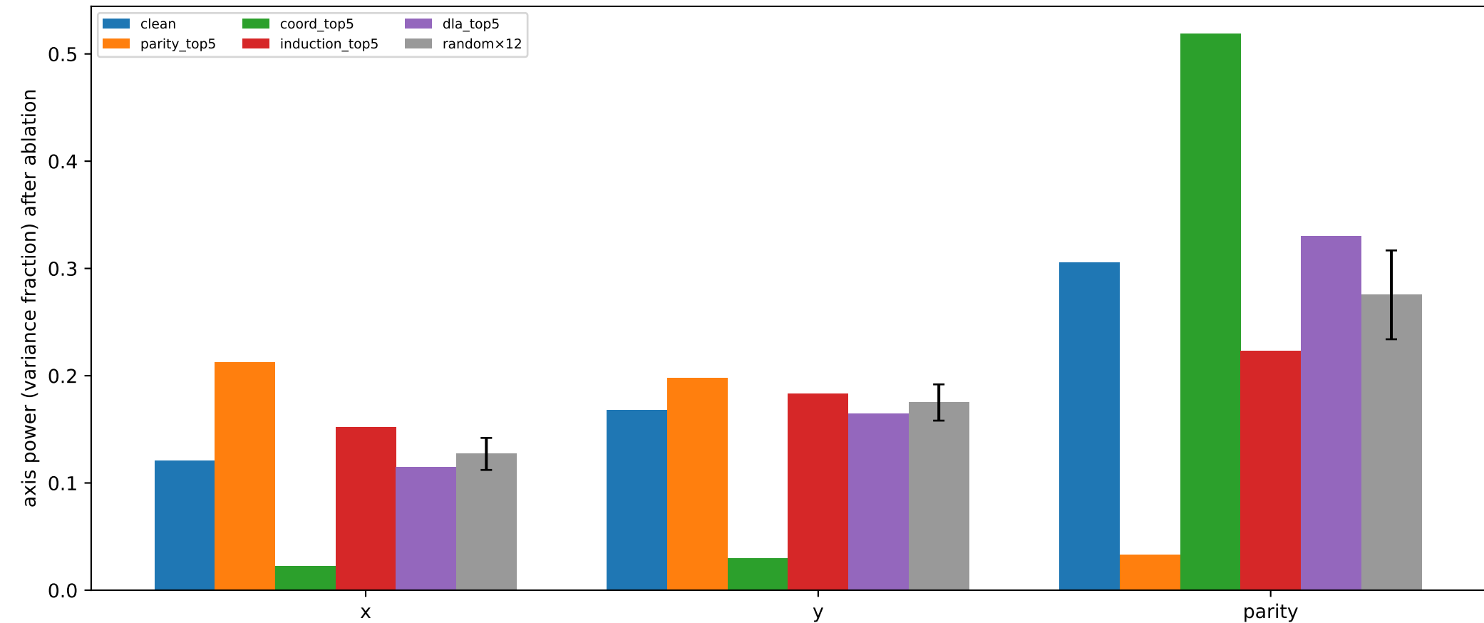
Llama square_grid — group ablation of K=5 heads: which set kills which axis (lower = more damage). clean = leftmost; random = grey control.
