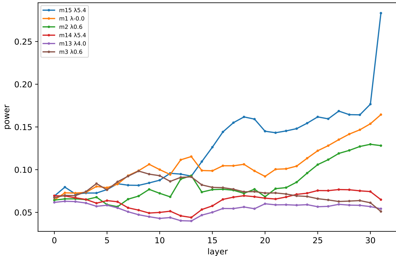
clean power vs layer, per eigenmode (emergence)
