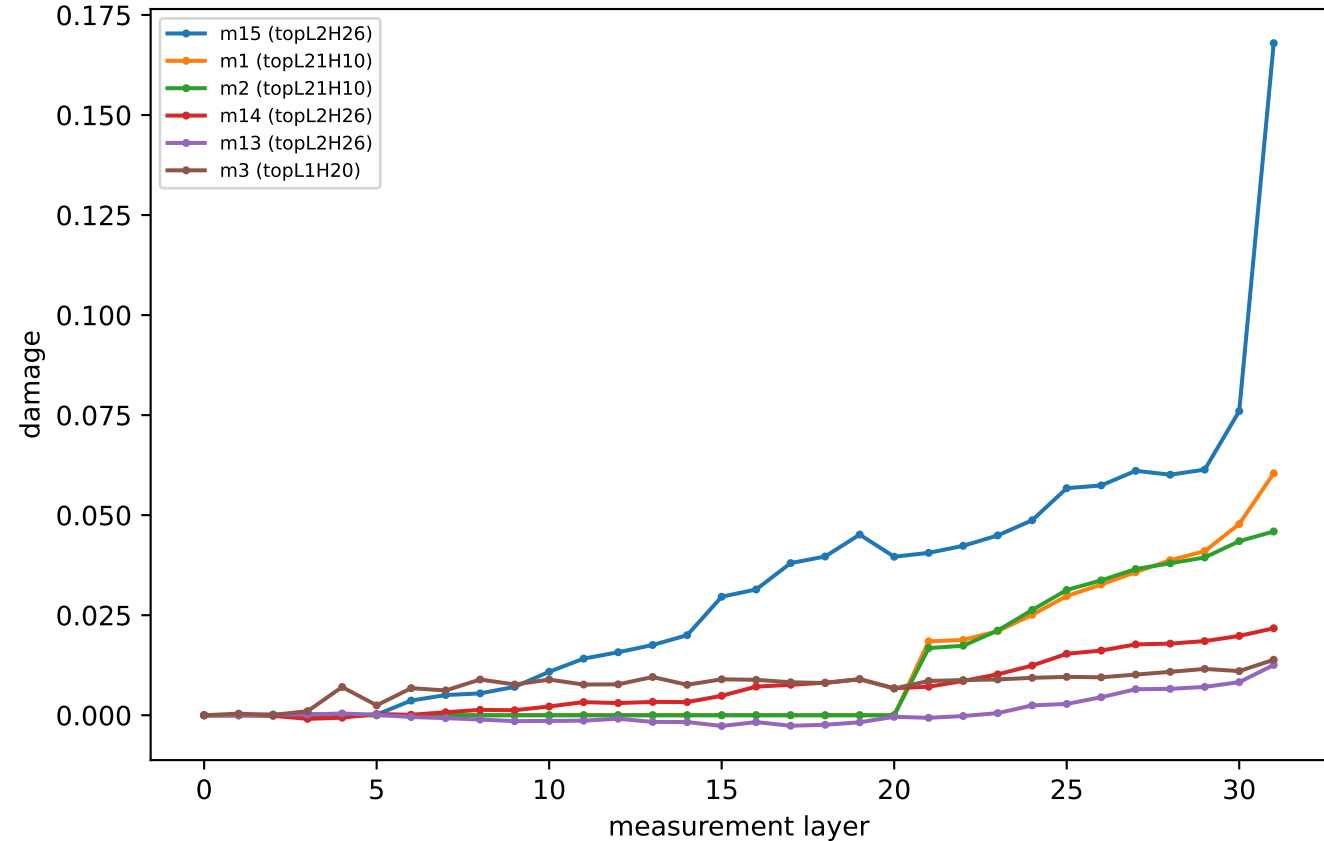
damage vs MEASUREMENT layer for each mode's top head (does it emerge early or late?)
