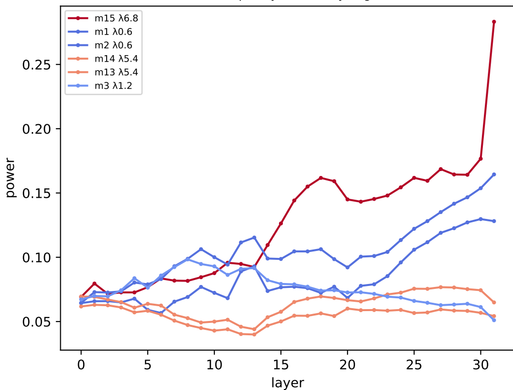
grid: clean power vs layer per eigenmode (colour = frequency; low→early, high→late)
