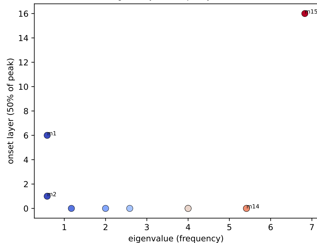
emergence layer vs frequency (r=+0.37)
