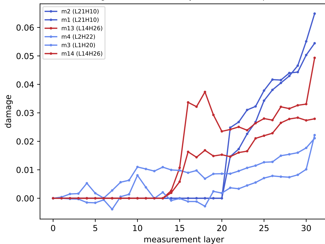
damage vs MEASUREMENT layer, each mode's top head
