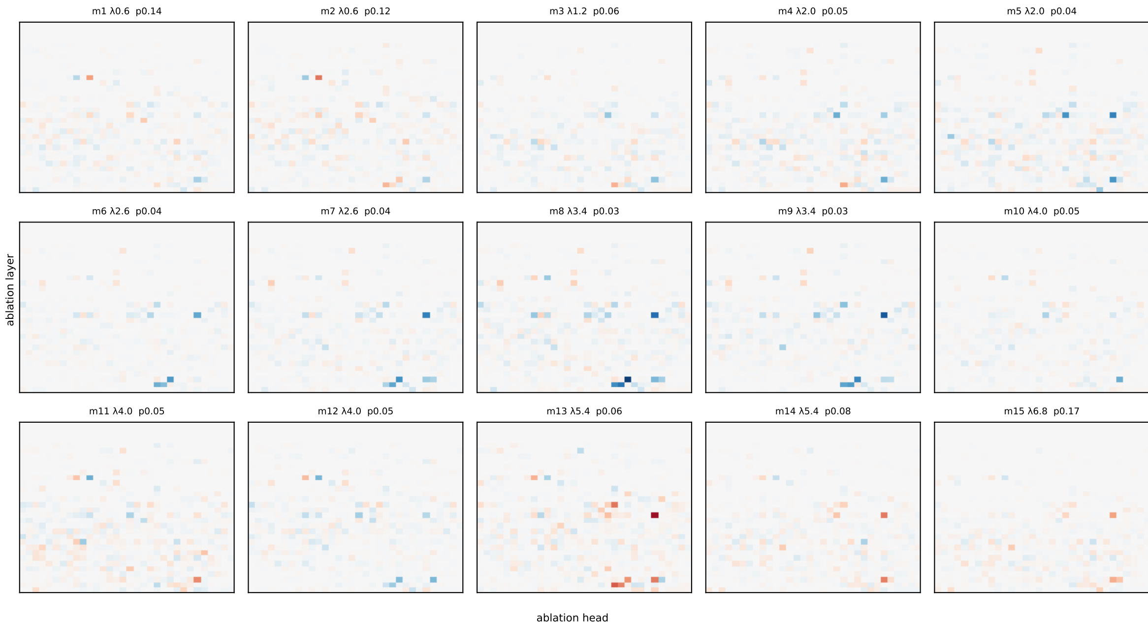
Llama grid — eigenmode damage heatmaps (ablation-layer[y] x head[x]) measured at LAYER 27 red = ablating that head weakens the mode at this layer; per-mode fixed scale
