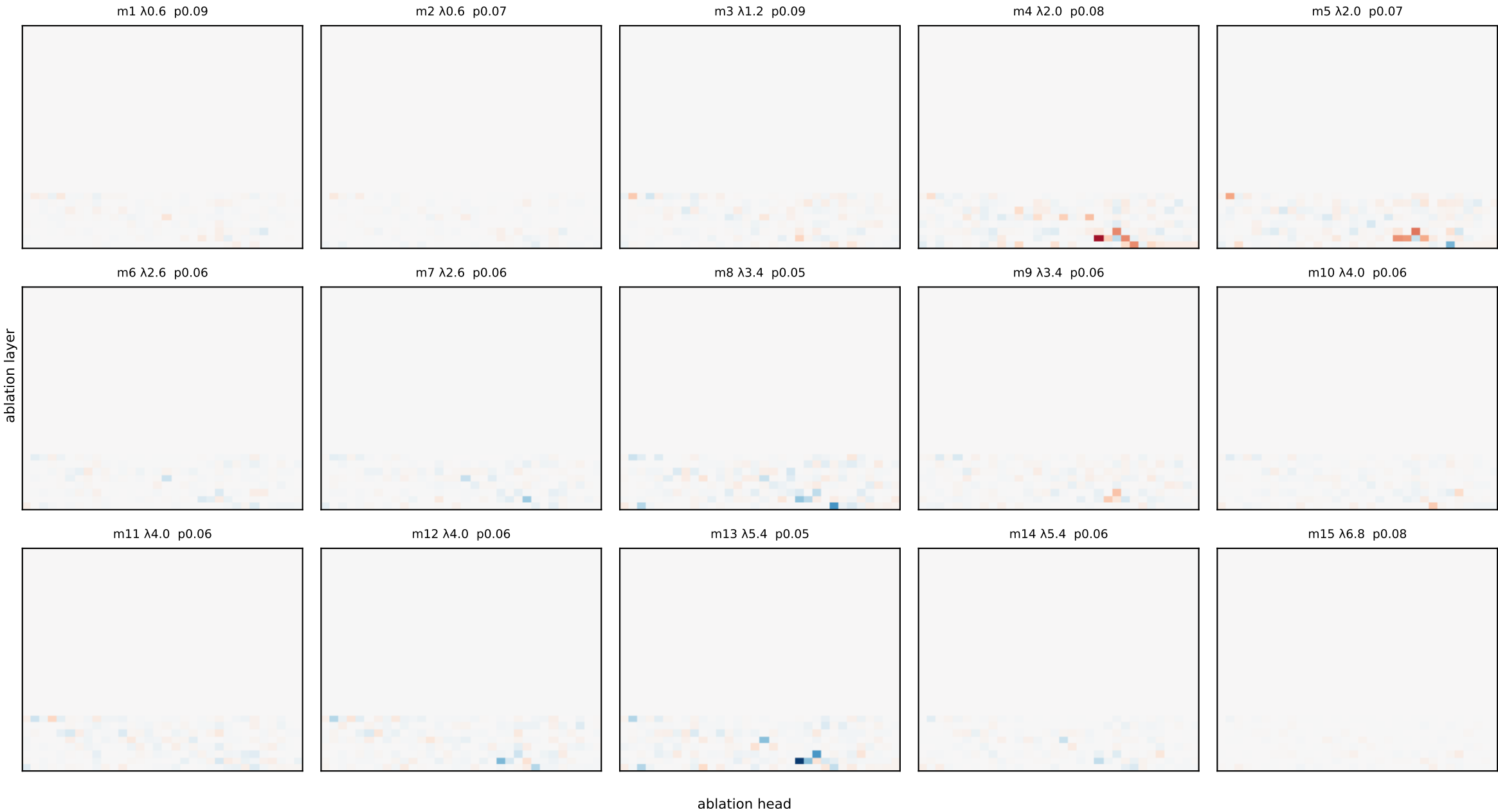
Llama grid — eigenmode damage heatmaps (ablation-layer[y] x head[x]) measured at LAYER 7 red = ablating that head weakens the mode at this layer; per-mode fixed scale
