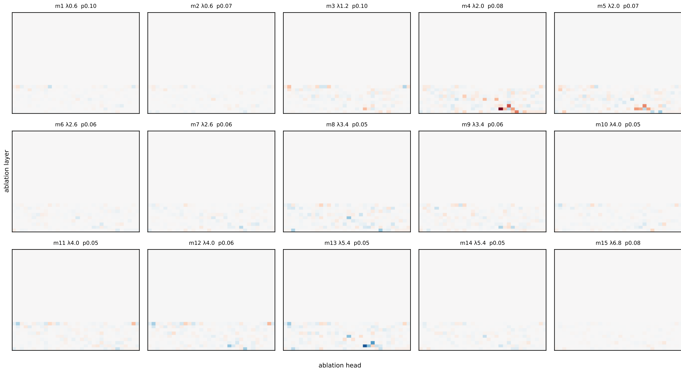
Llama grid — eigenmode damage heatmaps (ablation-layer[y] x head[x]) measured at LAYER 8 red = ablating that head weakens the mode at this layer; per-mode fixed scale
