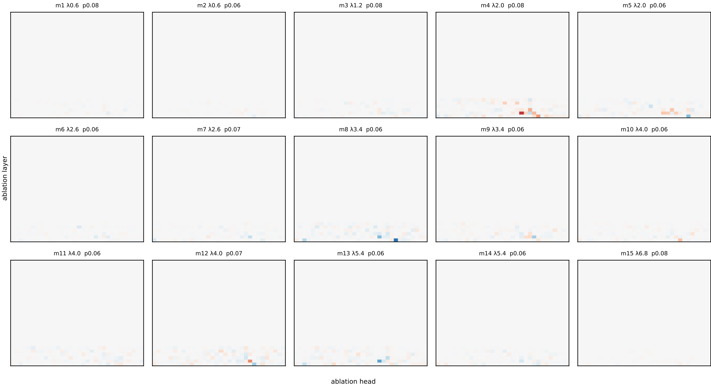
Llama grid — eigenmode damage heatmaps (ablation-layer[y] x head[x]) measured at LAYER 5 red = ablating that head weakens the mode at this layer; per-mode fixed scale
