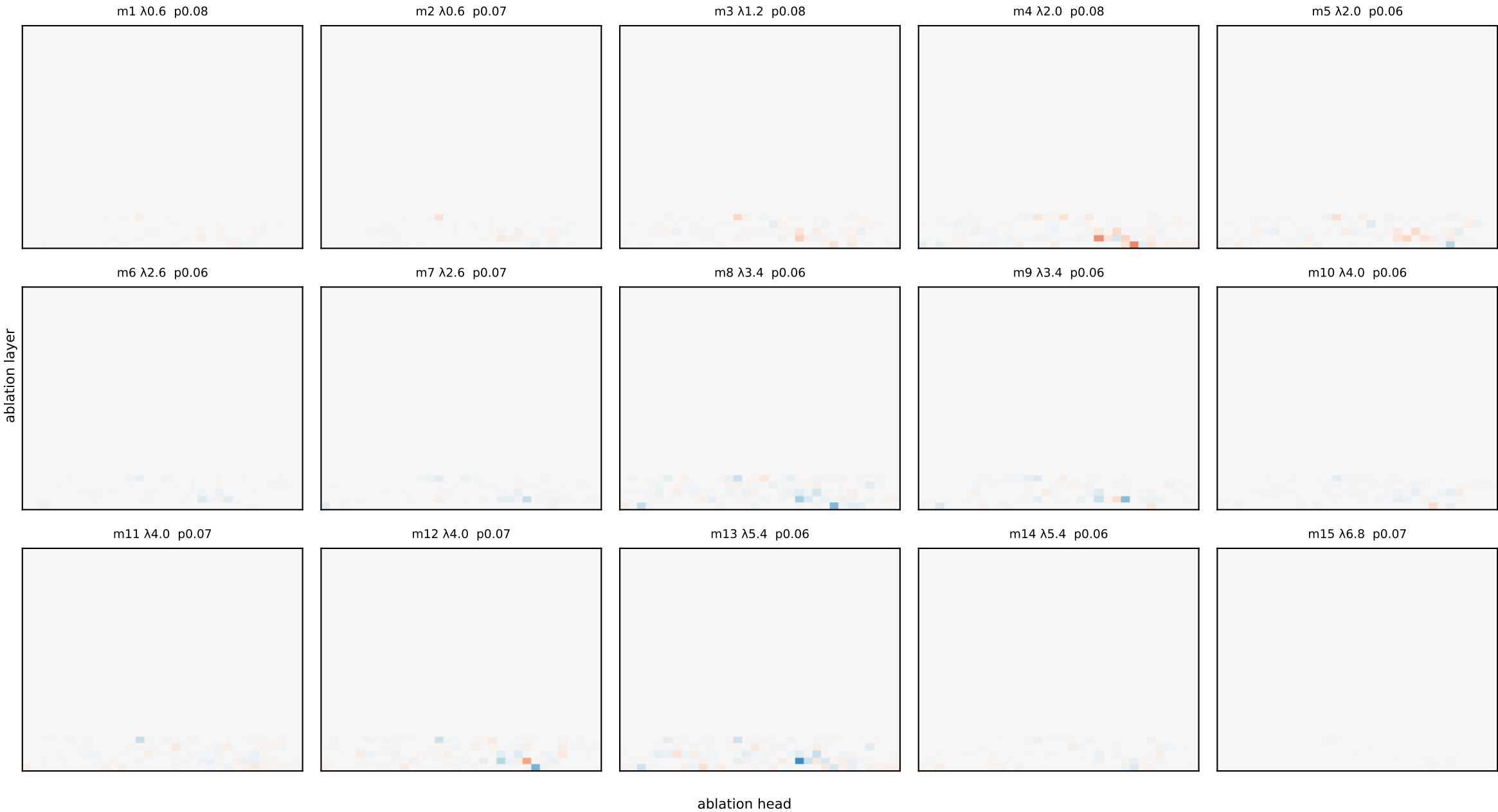
Llama grid — eigenmode damage heatmaps (ablation-layer[y] x head[x]) measured at LAYER 4 red = ablating that head weakens the mode at this layer; per-mode fixed scale
