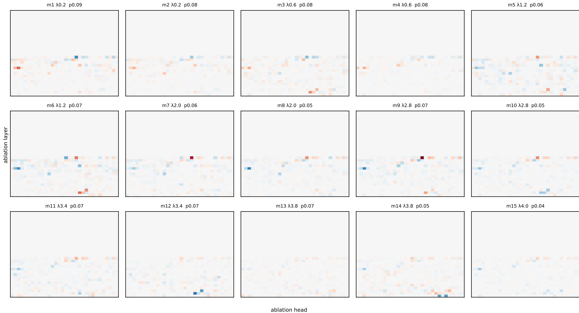
Llama ring — eigenmode damage heatmaps (ablation-layer[y] x head[x]) measured at LAYER 14 red = ablating that head weakens the mode at this layer; per-mode fixed scale
