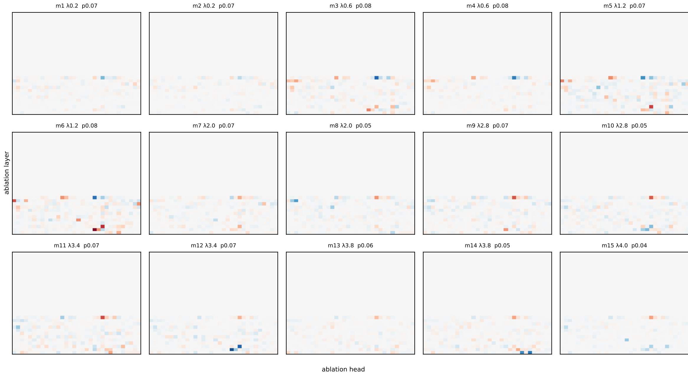
Llama ring — eigenmode damage heatmaps (ablation-layer[y] x head[x]) measured at LAYER 11 red = ablating that head weakens the mode at this layer; per-mode fixed scale
