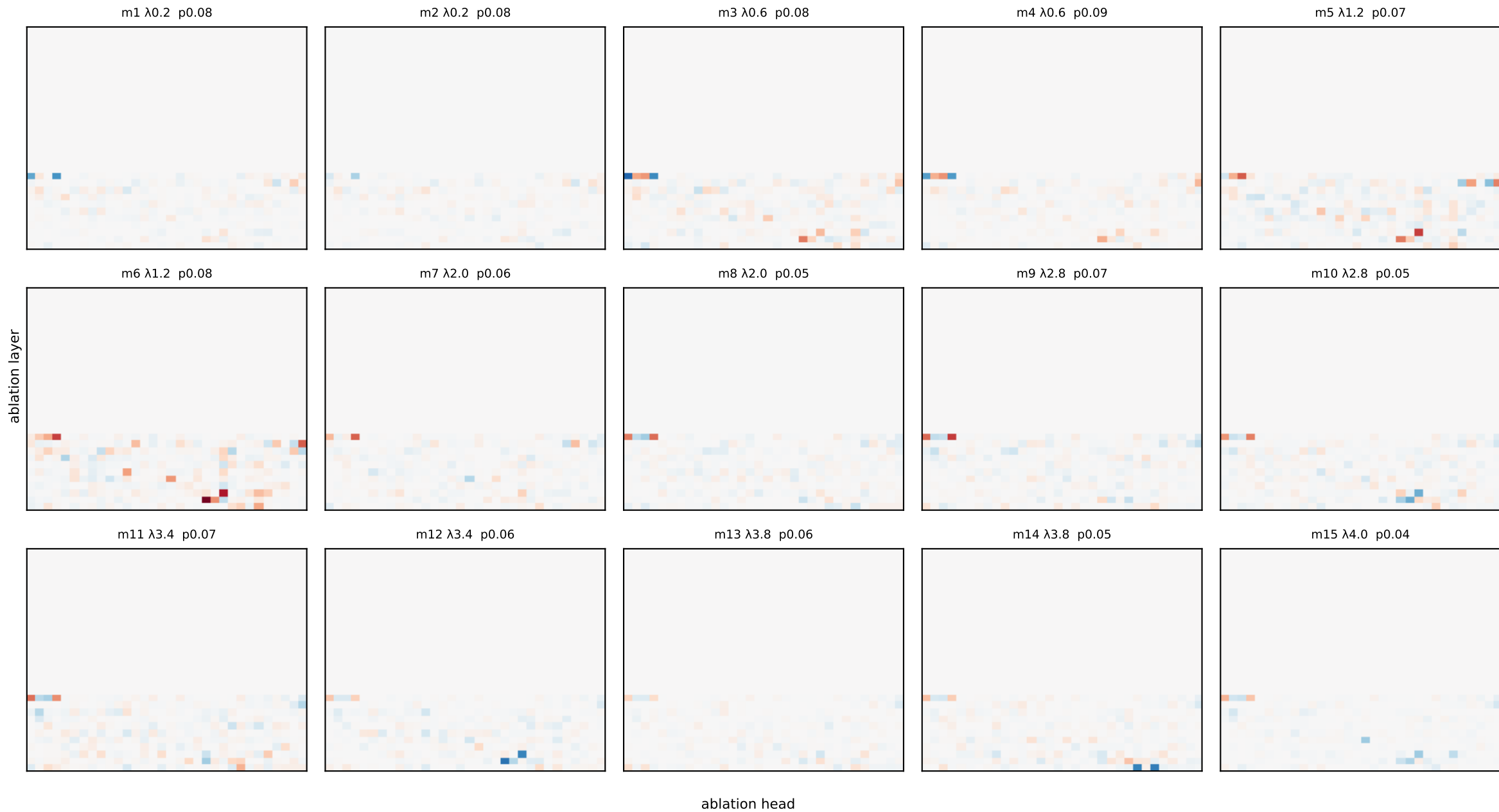
Llama ring — eigenmode damage heatmaps (ablation-layer[y] x head[x]) measured at LAYER 10 red = ablating that head weakens the mode at this layer; per-mode fixed scale
