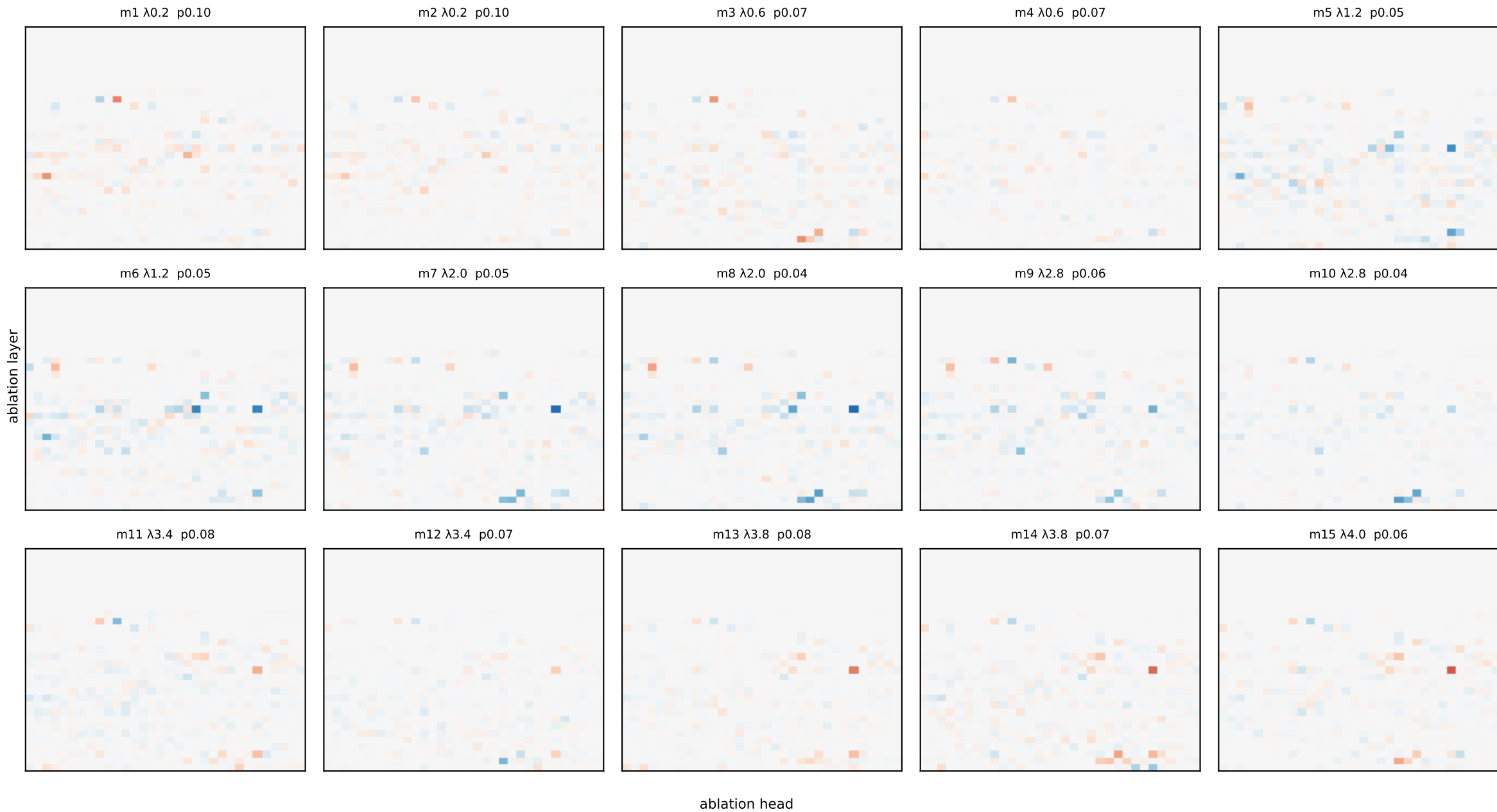
Llama ring — eigenmode damage heatmaps (ablation-layer[y] x head[x]) measured at LAYER 22 red = ablating that head weakens the mode at this layer; per-mode fixed scale
