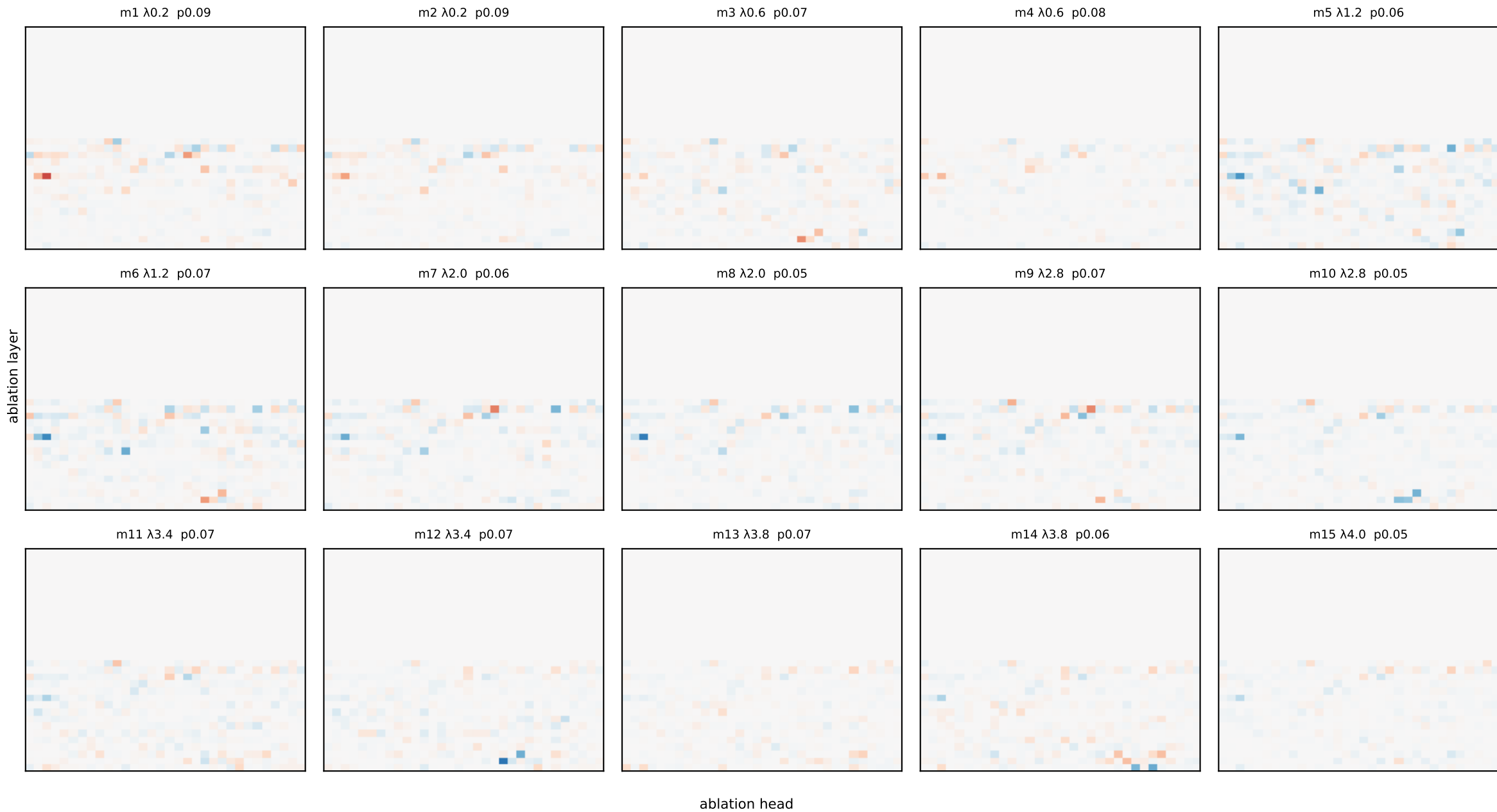
Llama ring — eigenmode damage heatmaps (ablation-layer[y] x head[x]) measured at LAYER 15 red = ablating that head weakens the mode at this layer; per-mode fixed scale
