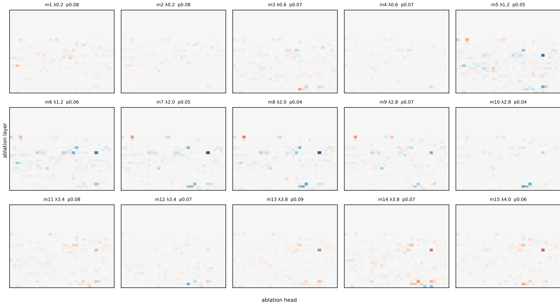
Llama ring — eigenmode damage heatmaps (ablation-layer[y] x head[x]) measured at LAYER 20 red = ablating that head weakens the mode at this layer; per-mode fixed scale
