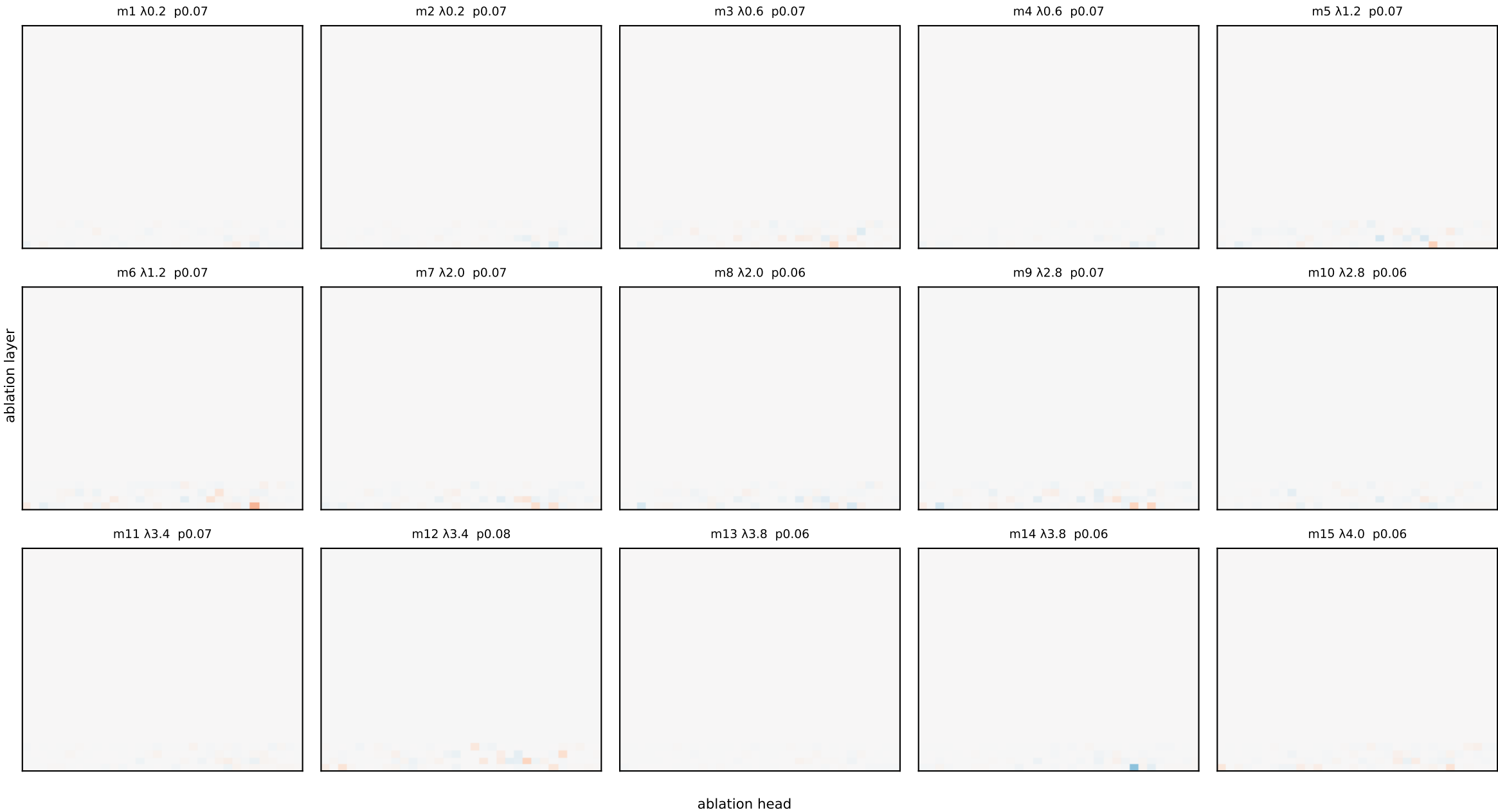
Llama ring — eigenmode damage heatmaps (ablation-layer[y] x head[x]) measured at LAYER 3 red = ablating that head weakens the mode at this layer; per-mode fixed scale
