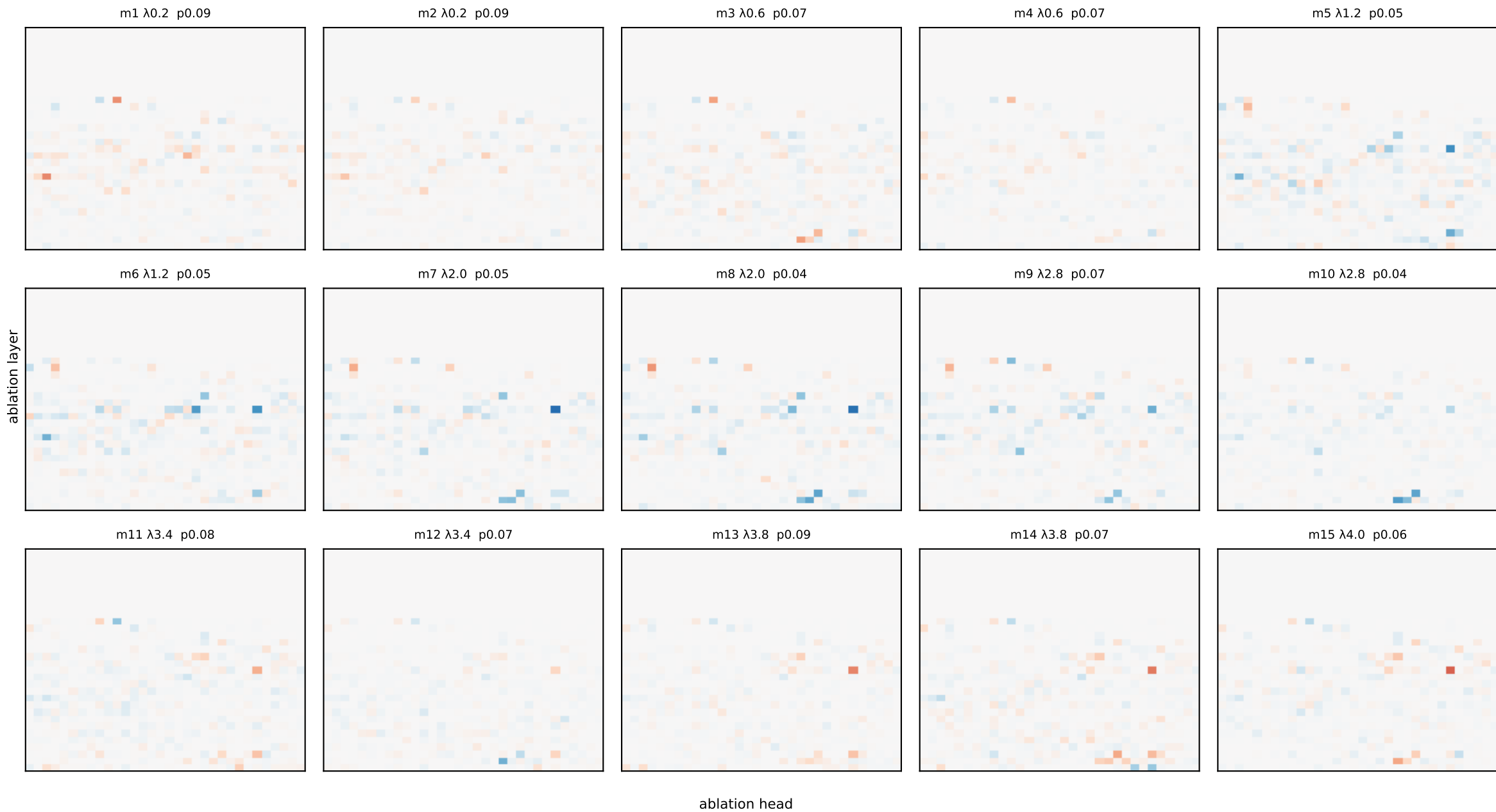
Llama ring — eigenmode damage heatmaps (ablation-layer[y] x head[x]) measured at LAYER 21 red = ablating that head weakens the mode at this layer; per-mode fixed scale
