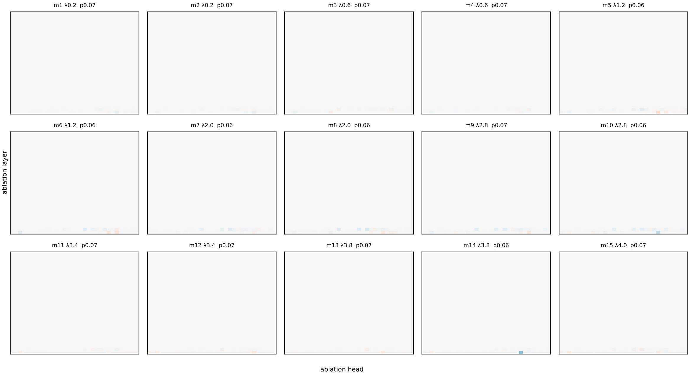
Llama ring — eigenmode damage heatmaps (ablation-layer[y] x head[x]) measured at LAYER 1 red = ablating that head weakens the mode at this layer; per-mode fixed scale
