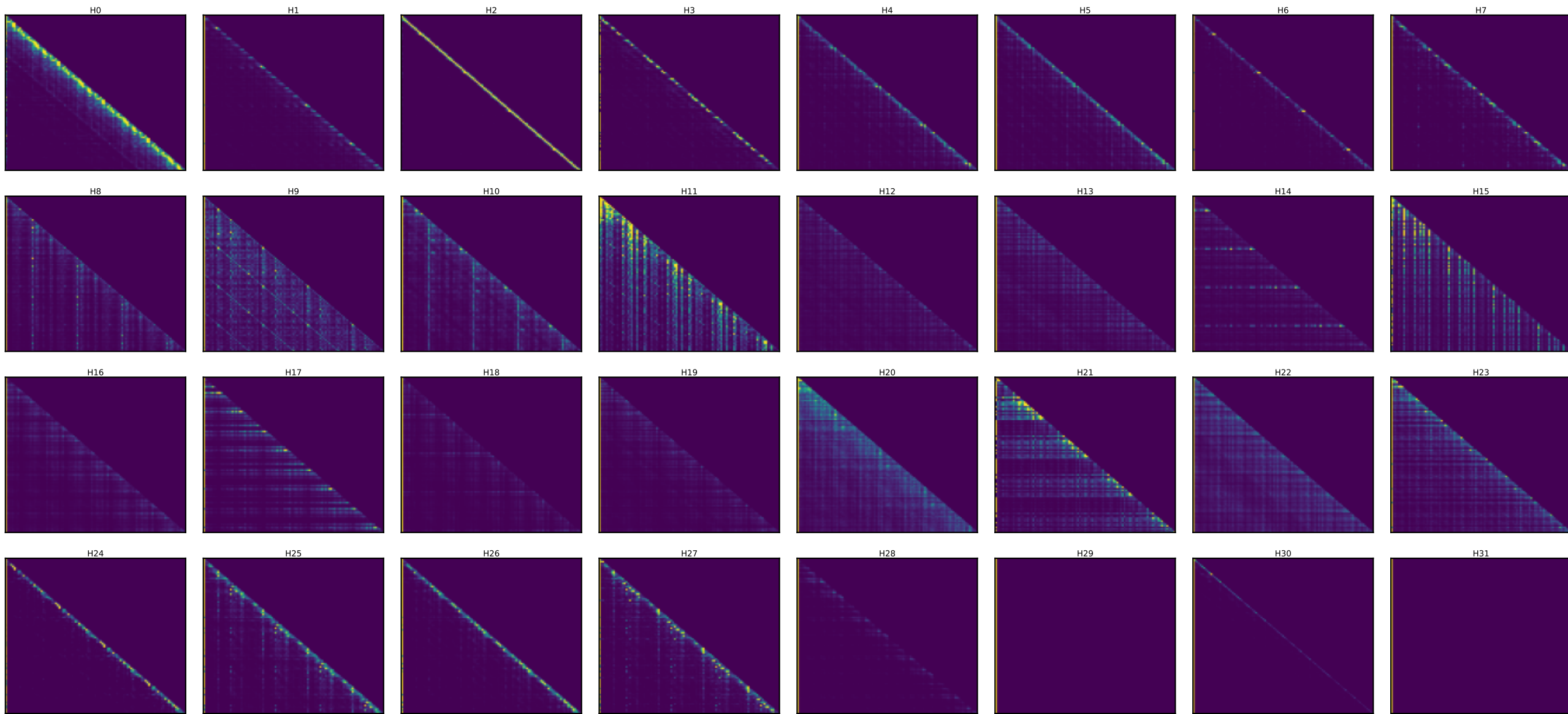
Llama layer 0 — every head's attention [25 random toks x4 + SOS] (induction stripe = diagonal at key=query-25)
