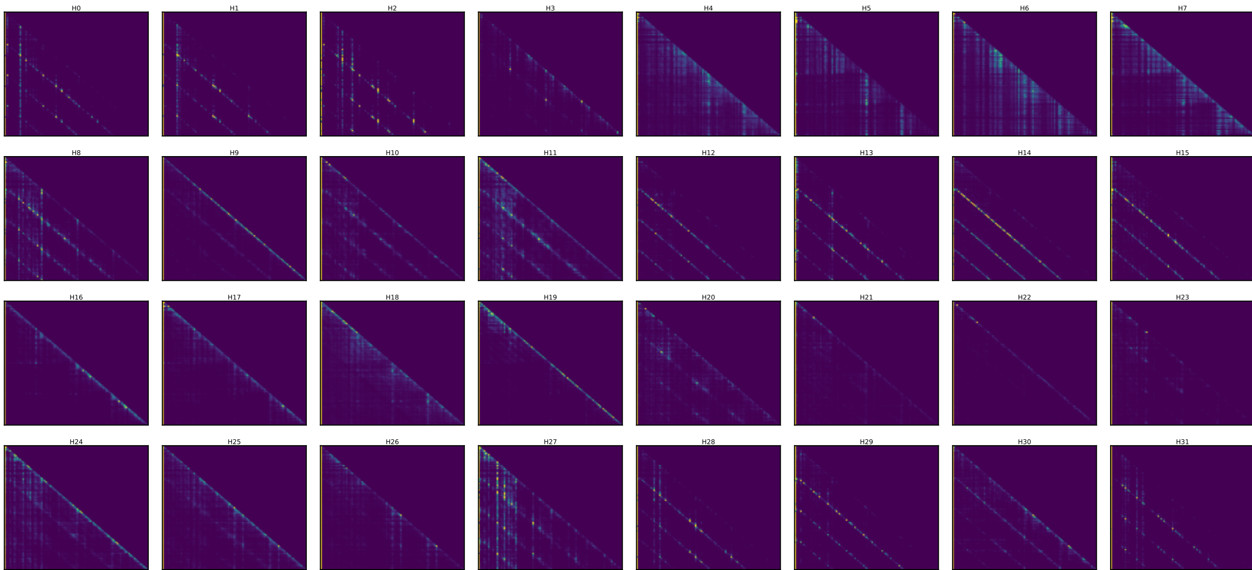
Llama layer 22 — every head's attention [25 random toks x4 + SOS] (induction stripe = diagonal at key=query-25)
