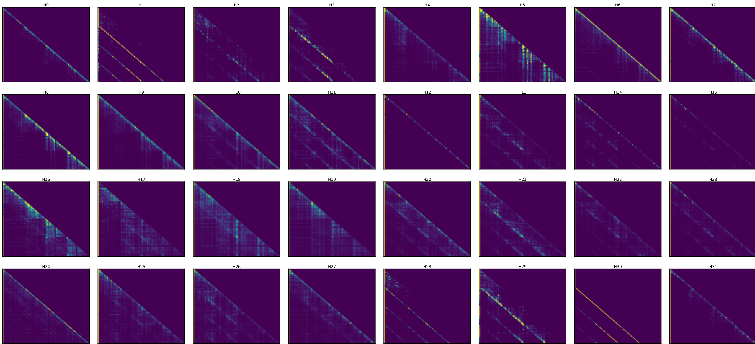
Llama layer 15 — every head's attention [25 random toks x4 + SOS] (induction stripe = diagonal at key=query-25)
