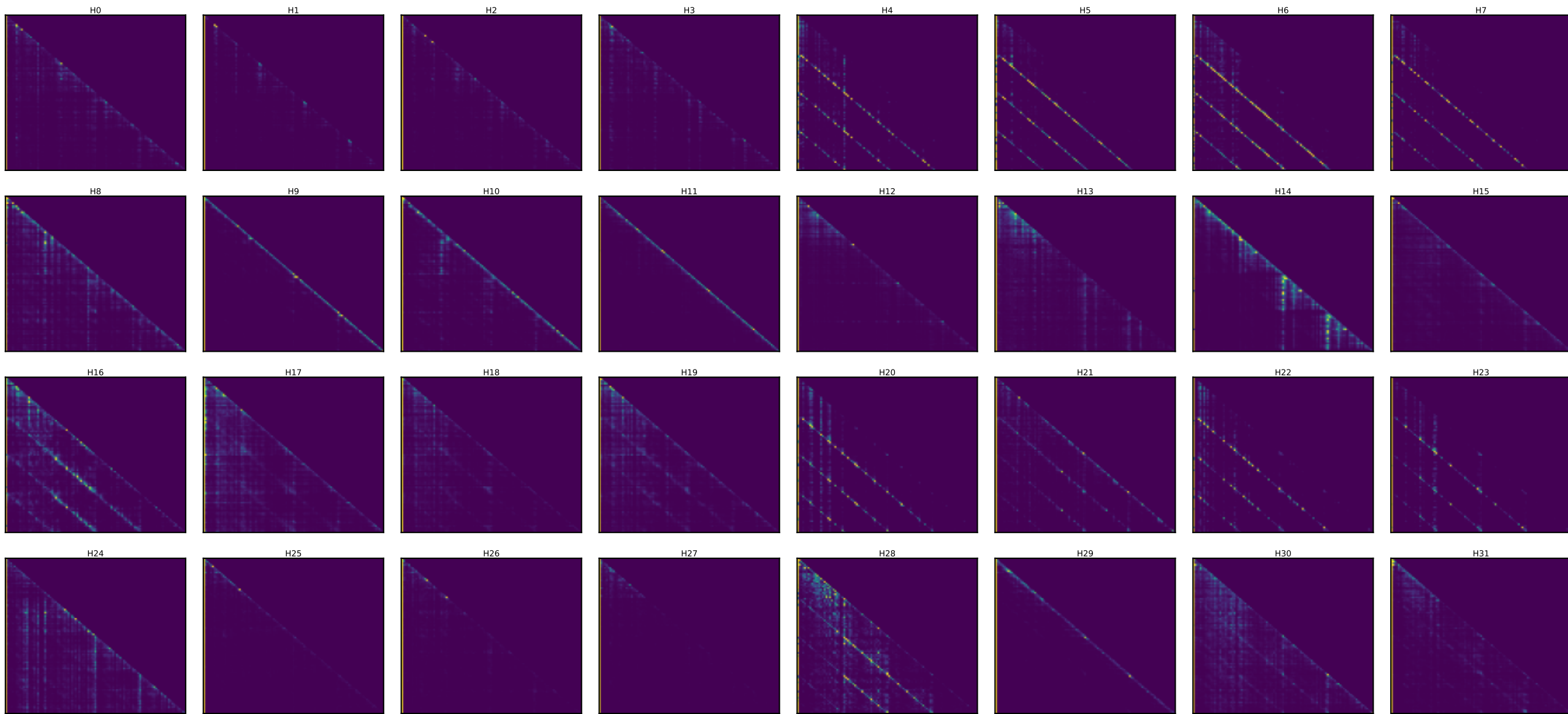
Llama layer 27 — every head's attention [25 random toks x4 + SOS] (induction stripe = diagonal at key=query-25)
