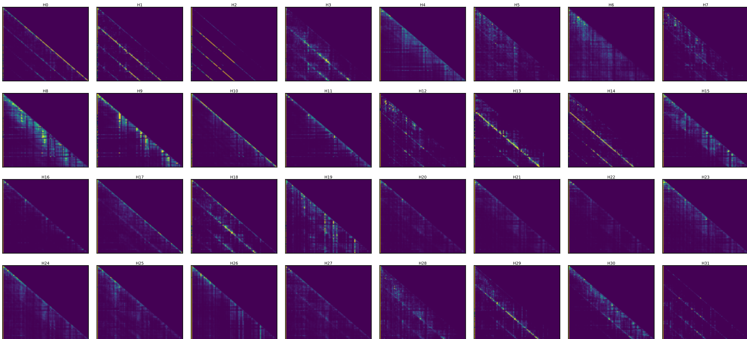
Llama layer 10 — every head's attention [25 random toks x4 + SOS] (induction stripe = diagonal at key=query-25)
