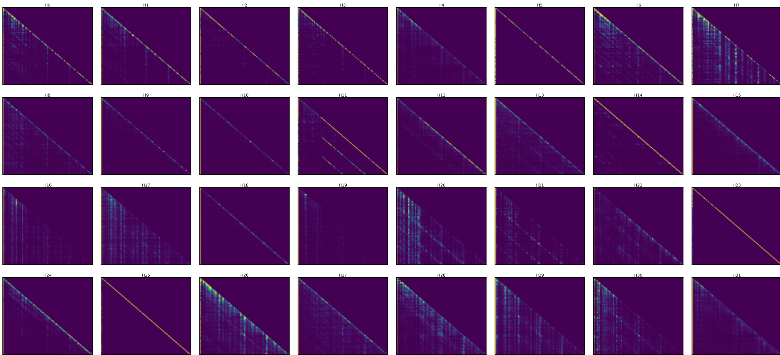
Llama layer 31 — every head's attention [25 random toks x4 + SOS] (induction stripe = diagonal at key=query-25)
