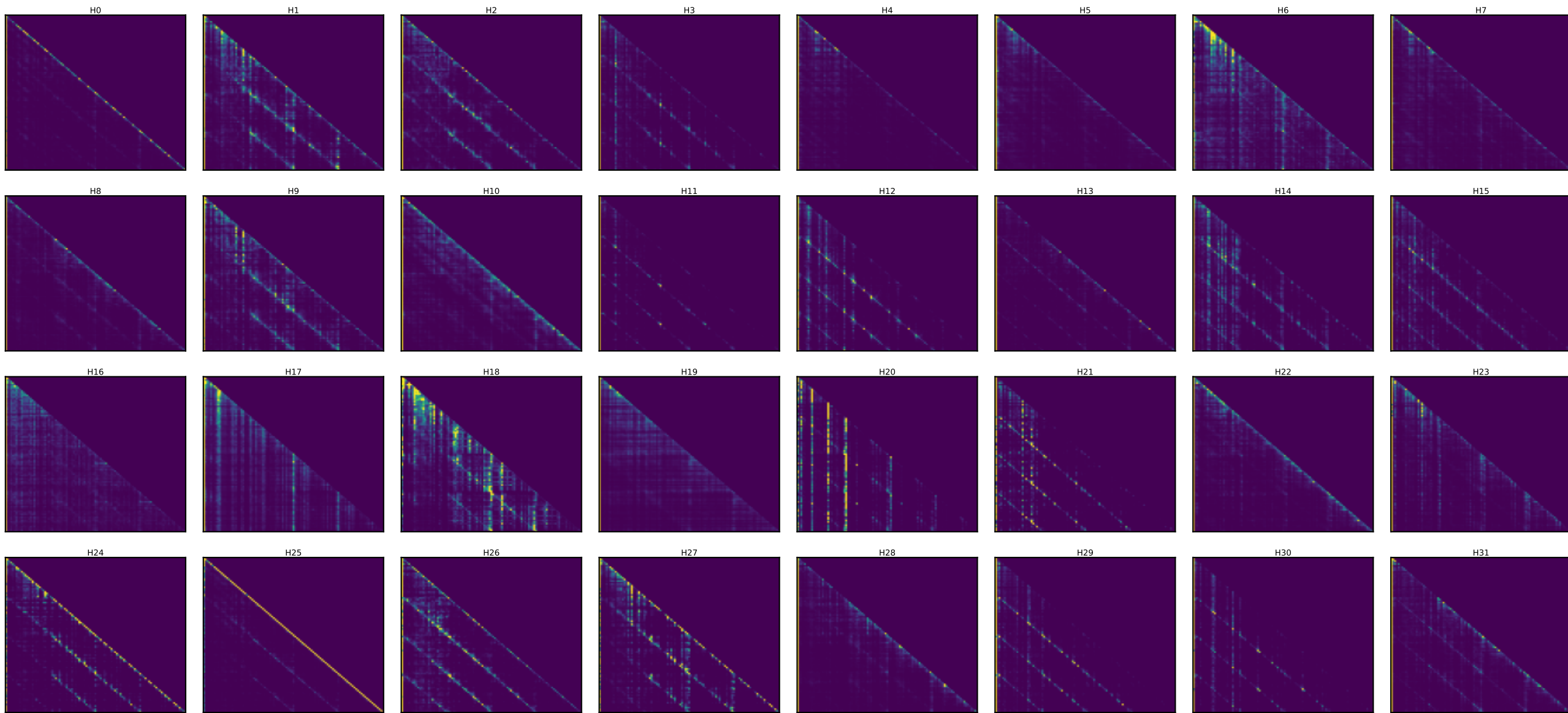
Llama layer 30 — every head's attention [25 random toks x4 + SOS] (induction stripe = diagonal at key=query-25)
