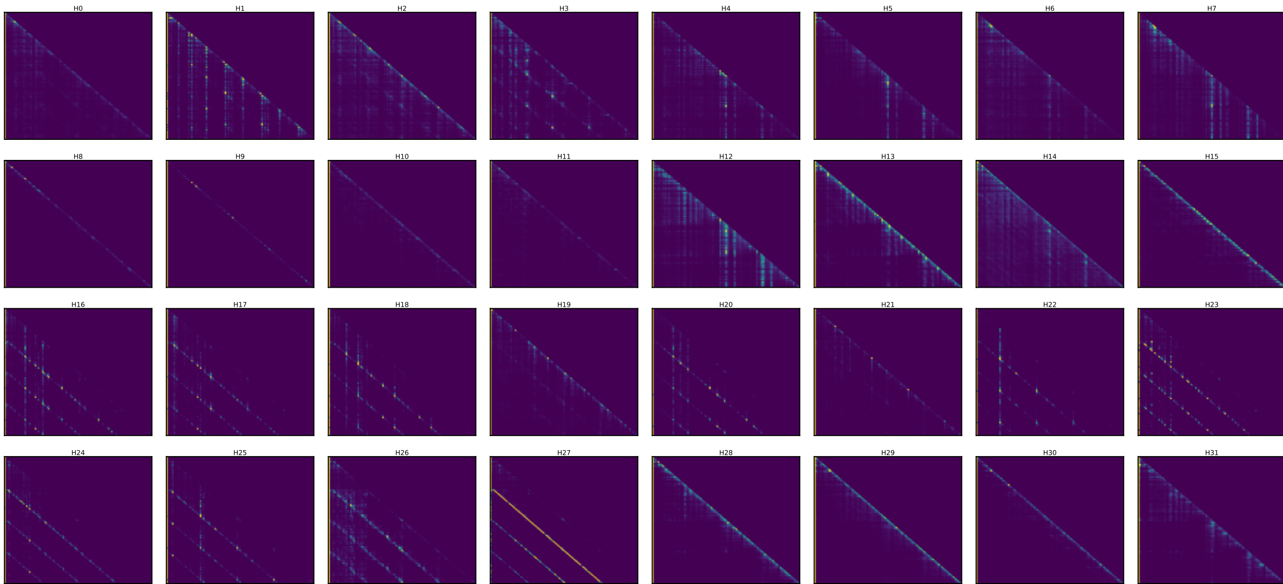
Llama layer 24 — every head's attention [25 random toks x4 + SOS] (induction stripe = diagonal at key=query-25)
