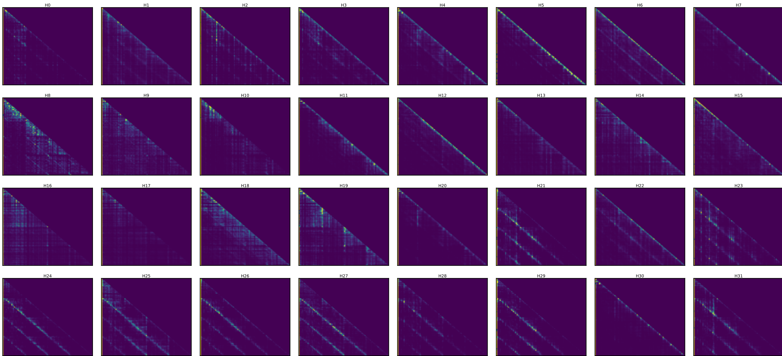
Llama layer 17 — every head's attention [25 random toks x4 + SOS] (induction stripe = diagonal at key=query-25)
