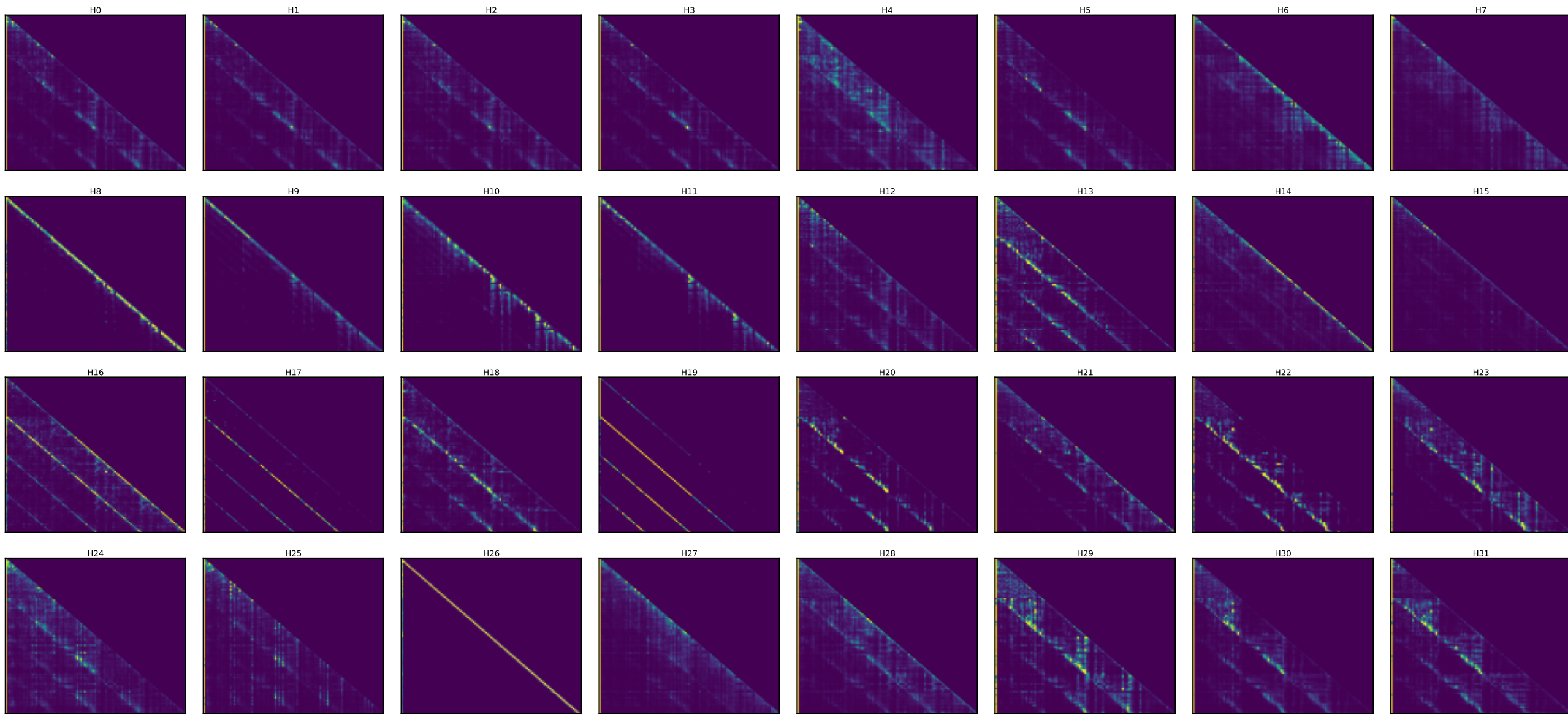
Llama layer 14 — every head's attention [25 random toks x4 + SOS] (induction stripe = diagonal at key=query-25)
