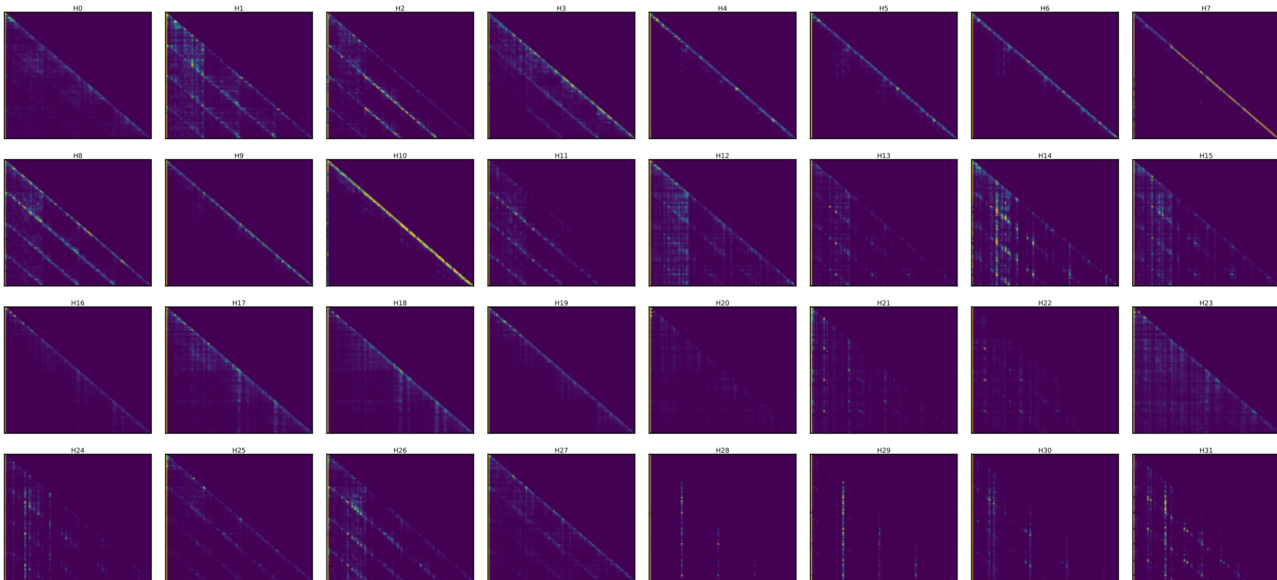
Llama layer 21 — every head's attention [25 random toks x4 + SOS] (induction stripe = diagonal at key=query-25)
