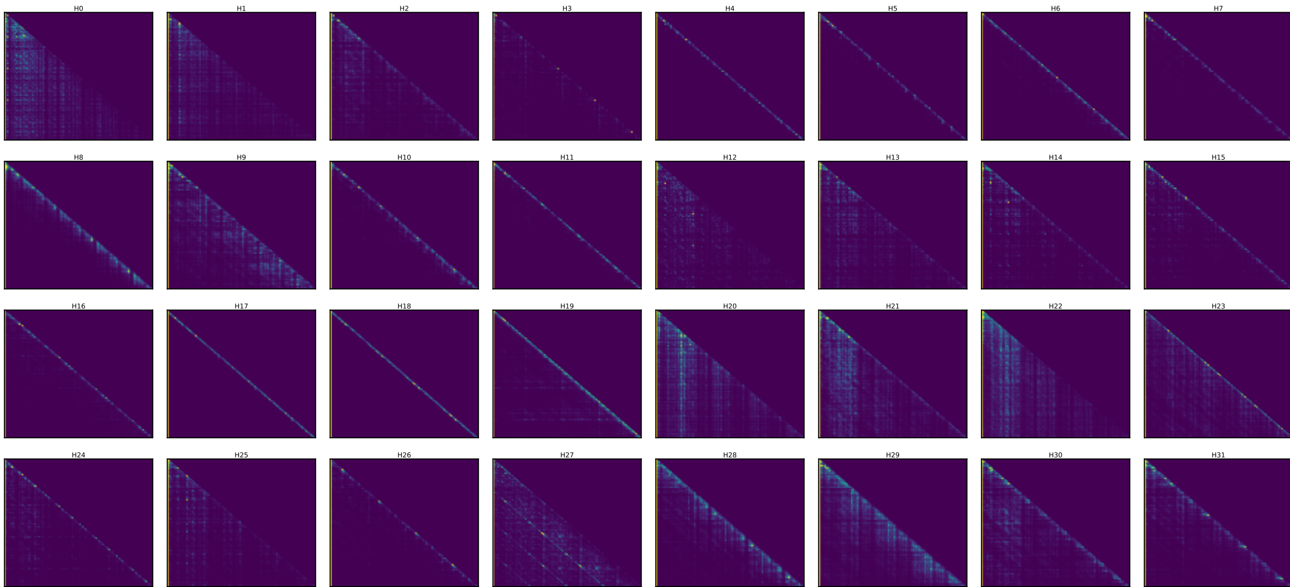
Llama layer 3 — every head's attention [25 random toks x4 + SOS] (induction stripe = diagonal at key=query-25)
