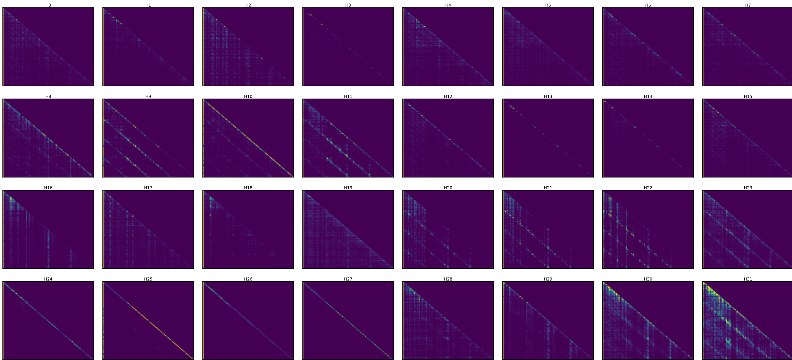
Llama layer 29 — every head's attention [25 random toks x4 + SOS] (induction stripe = diagonal at key=query-25)
