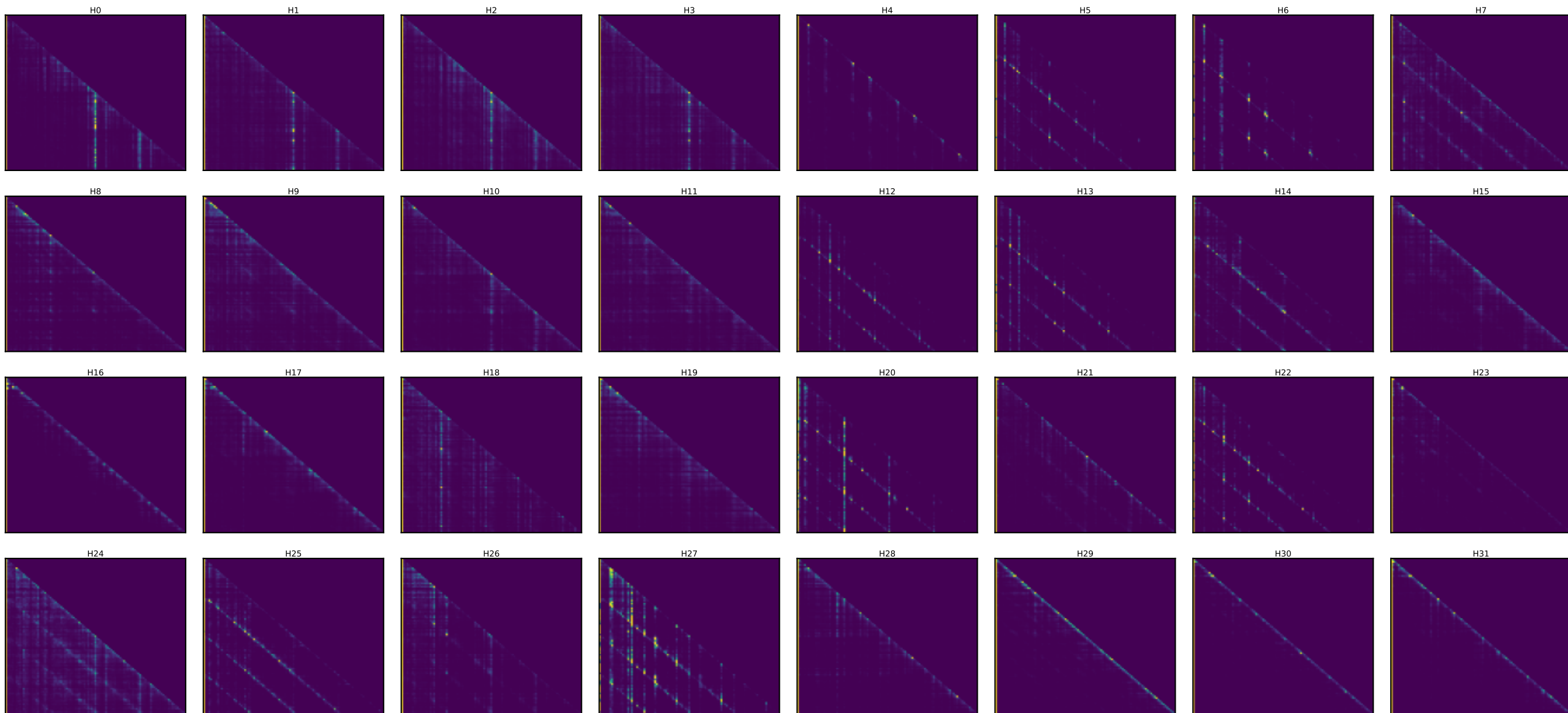
Llama layer 23 — every head's attention [25 random toks x4 + SOS] (induction stripe = diagonal at key=query-25)
