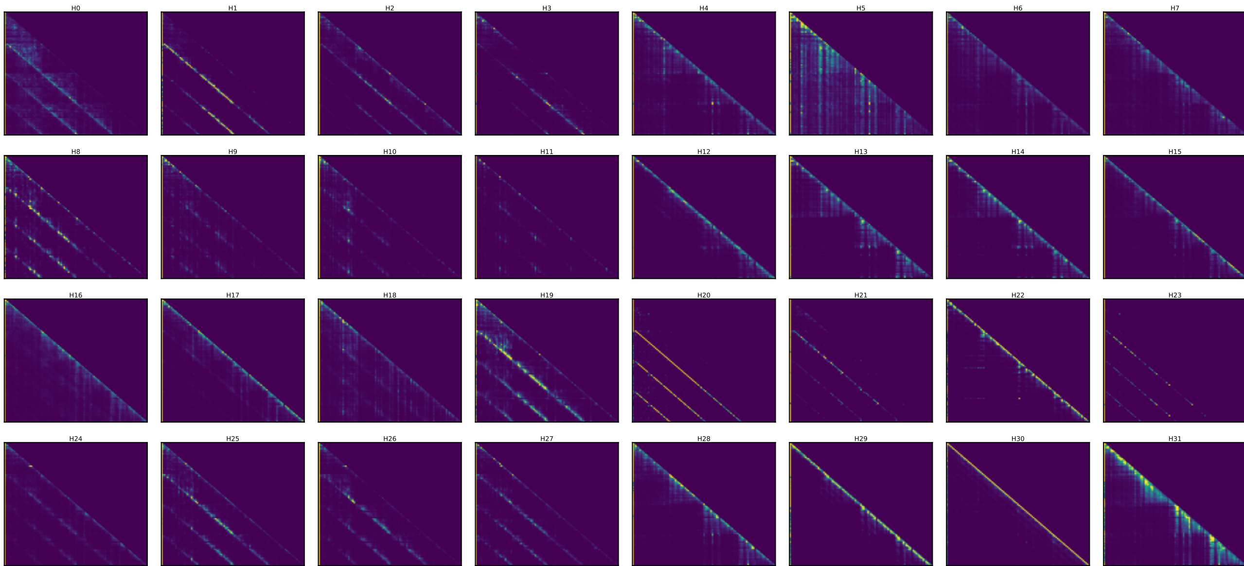
Llama layer 16 — every head's attention [25 random toks x4 + SOS] (induction stripe = diagonal at key=query-25)
