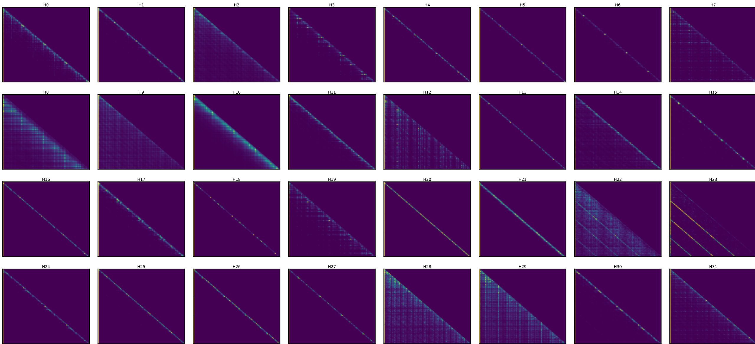
Llama layer 1 — every head's attention [25 random toks x4 + SOS] (induction stripe = diagonal at key=query-25)
