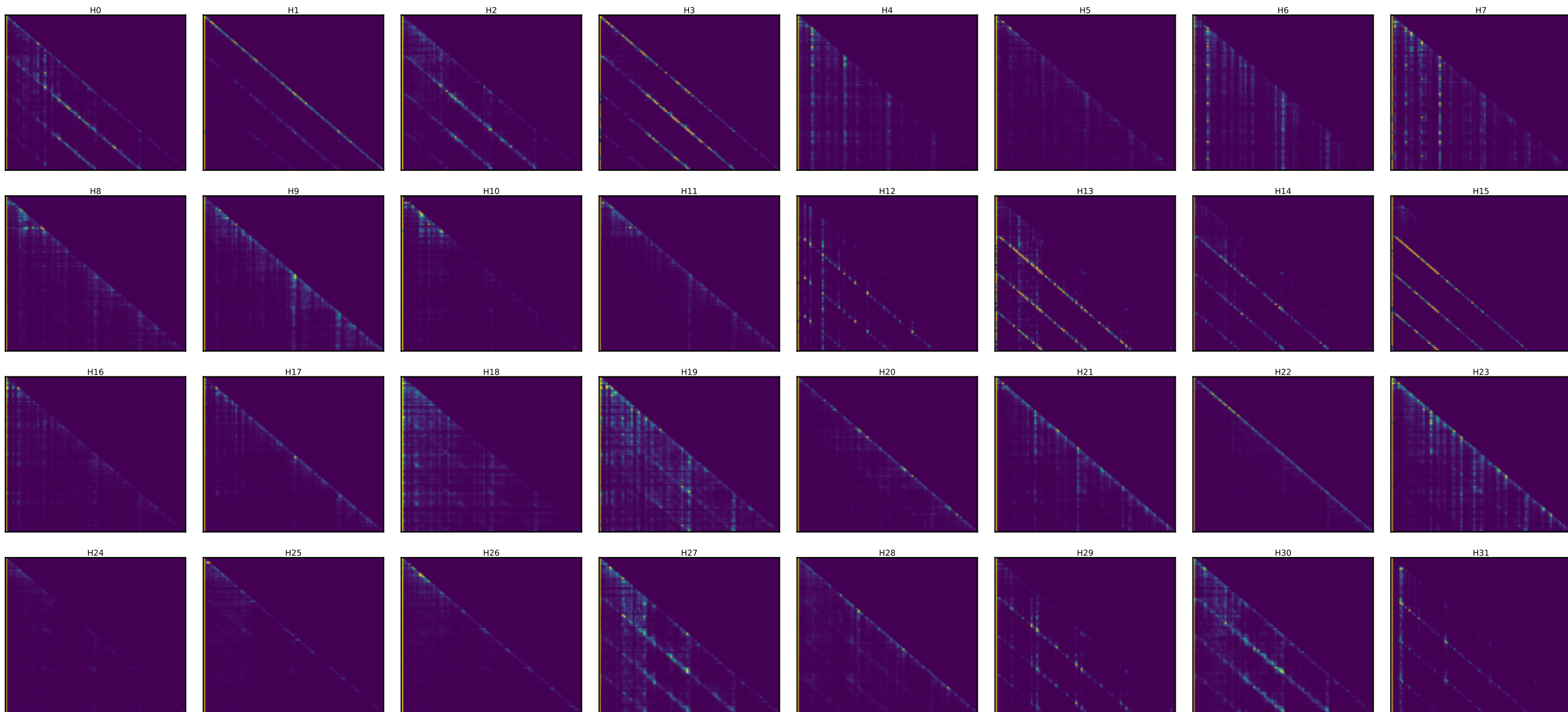
Llama layer 26 — every head's attention [25 random toks x4 + SOS] (induction stripe = diagonal at key=query-25)
