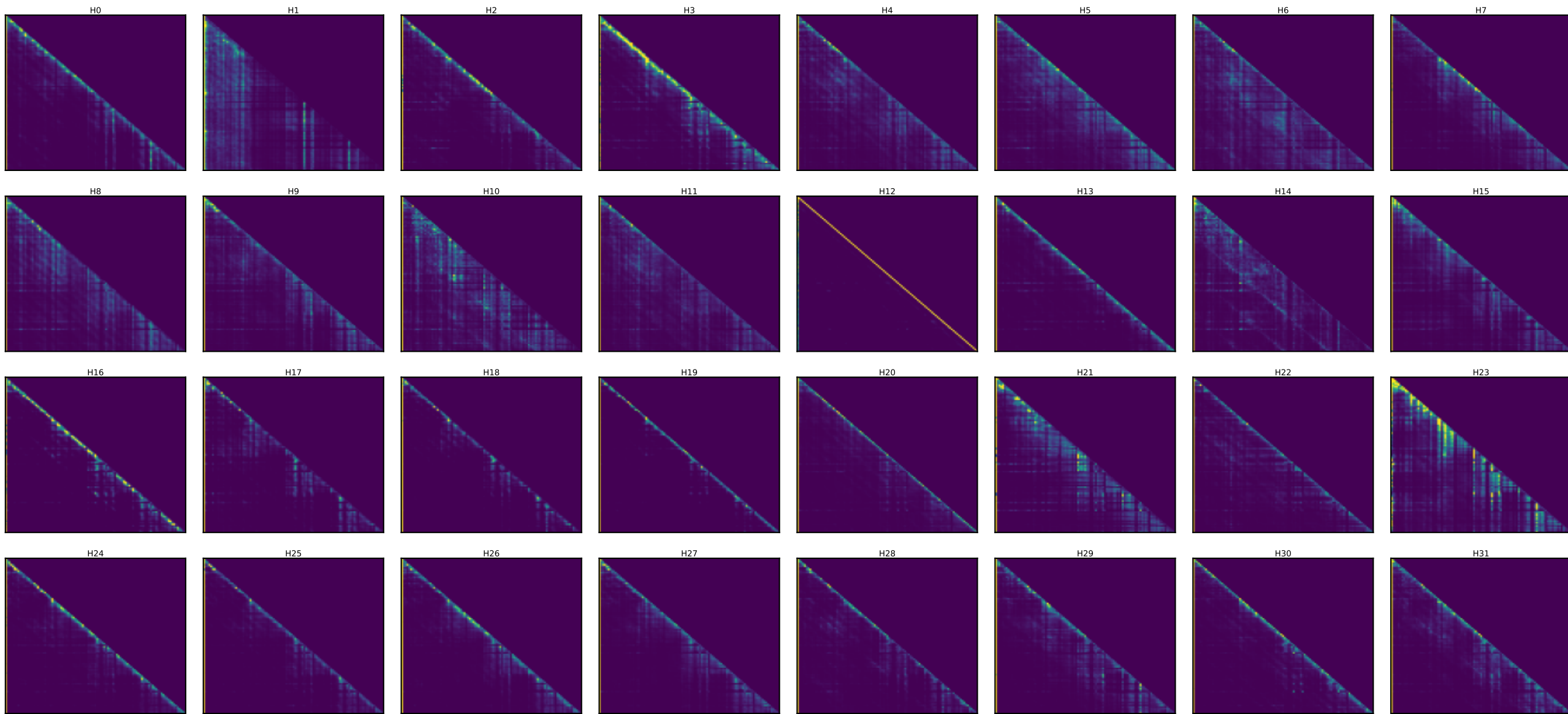
Llama layer 12 — every head's attention [25 random toks x4 + SOS] (induction stripe = diagonal at key=query-25)
