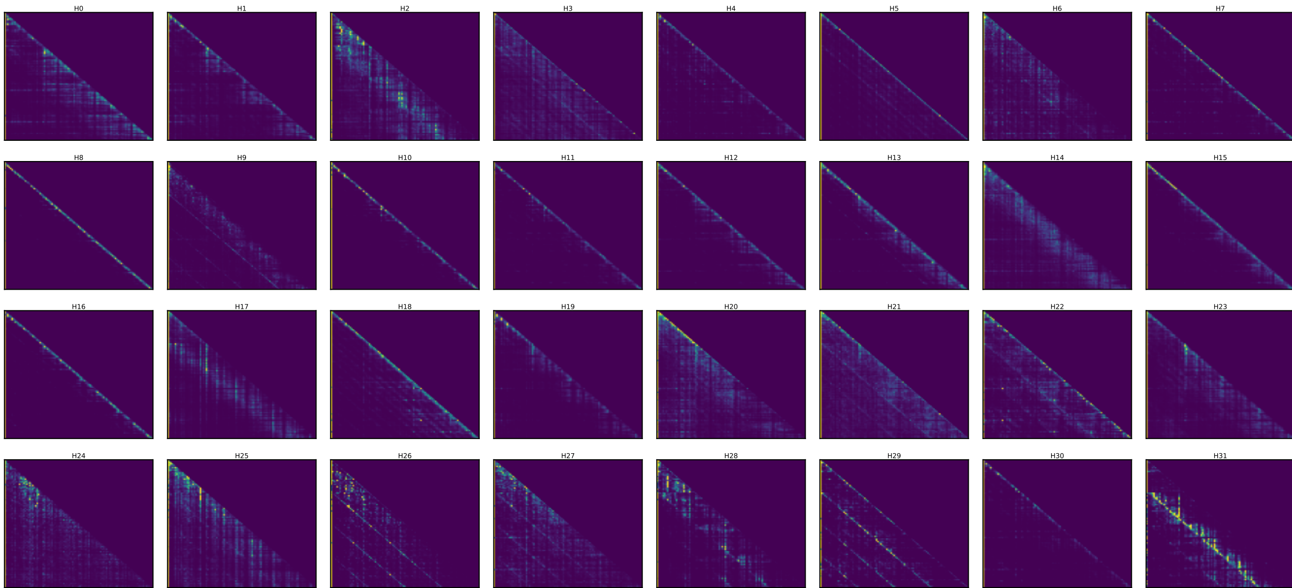
Llama layer 6 — every head's attention [25 random toks x4 + SOS] (induction stripe = diagonal at key=query-25)
