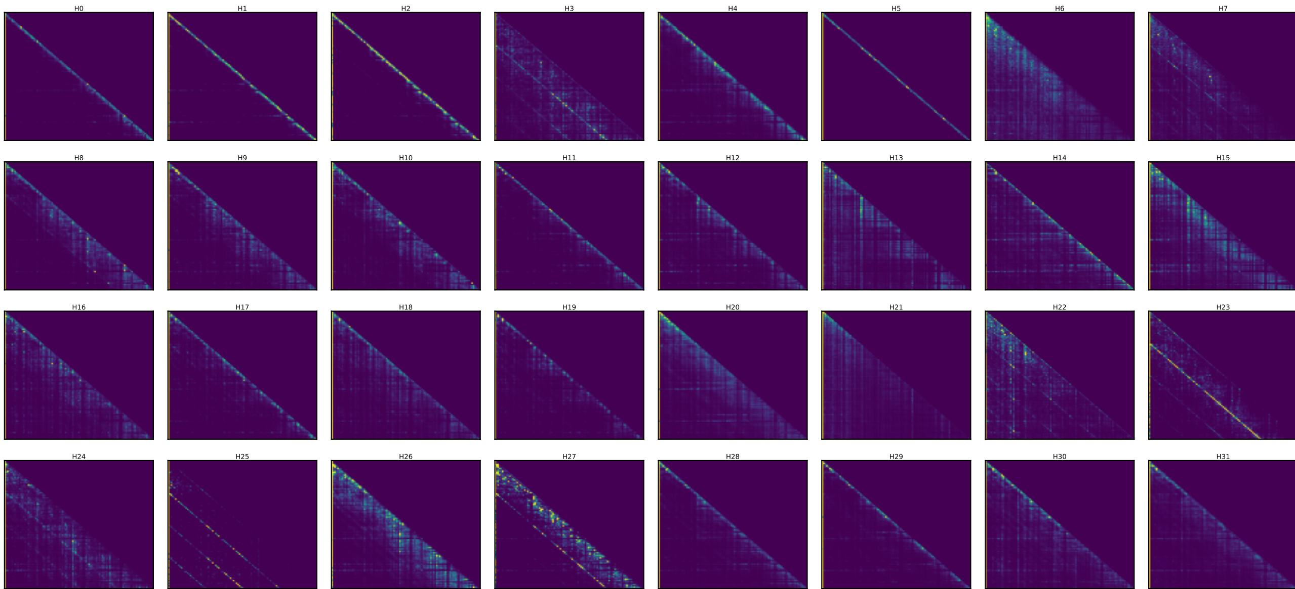
Llama layer 7 — every head's attention [25 random toks x4 + SOS] (induction stripe = diagonal at key=query-25)
