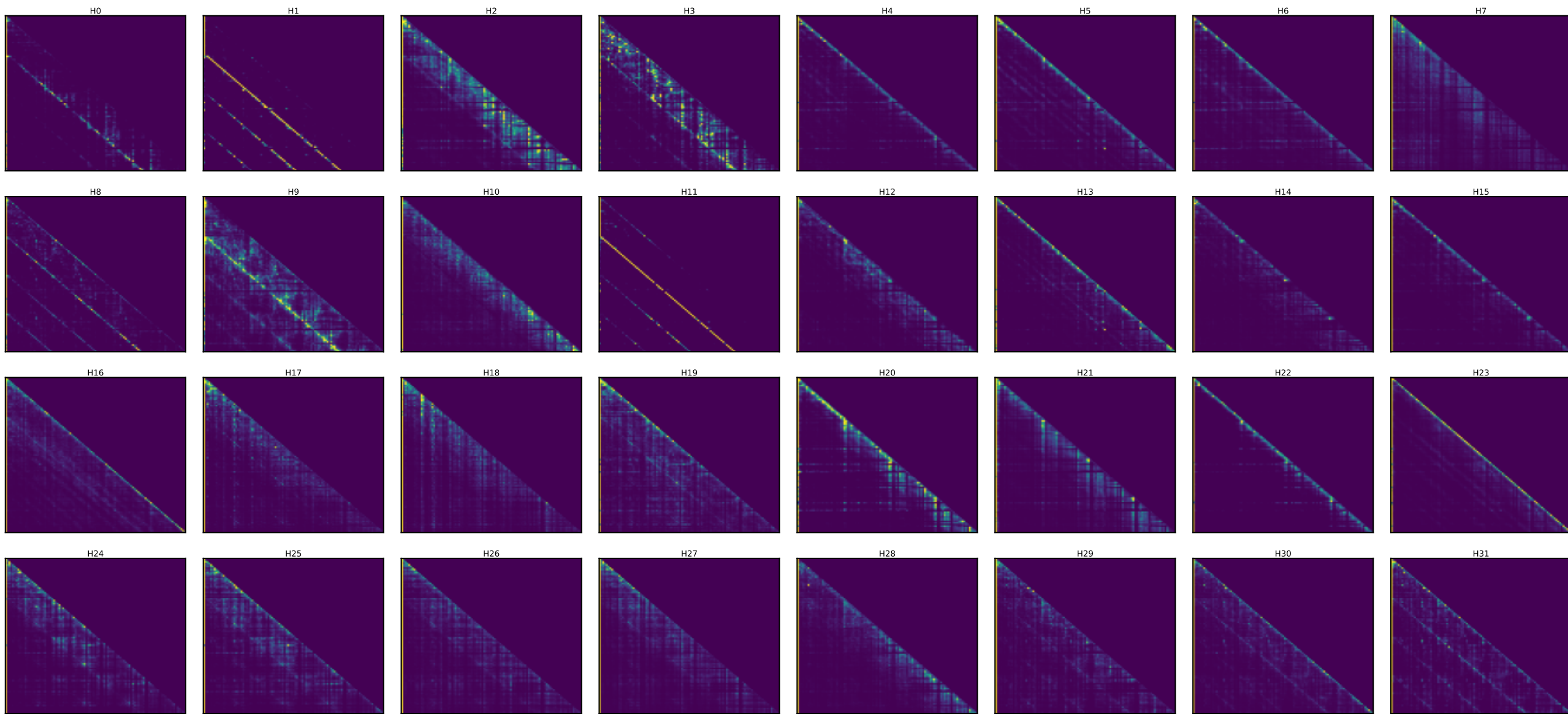
Llama layer 8 — every head's attention [25 random toks x4 + SOS] (induction stripe = diagonal at key=query-25)
