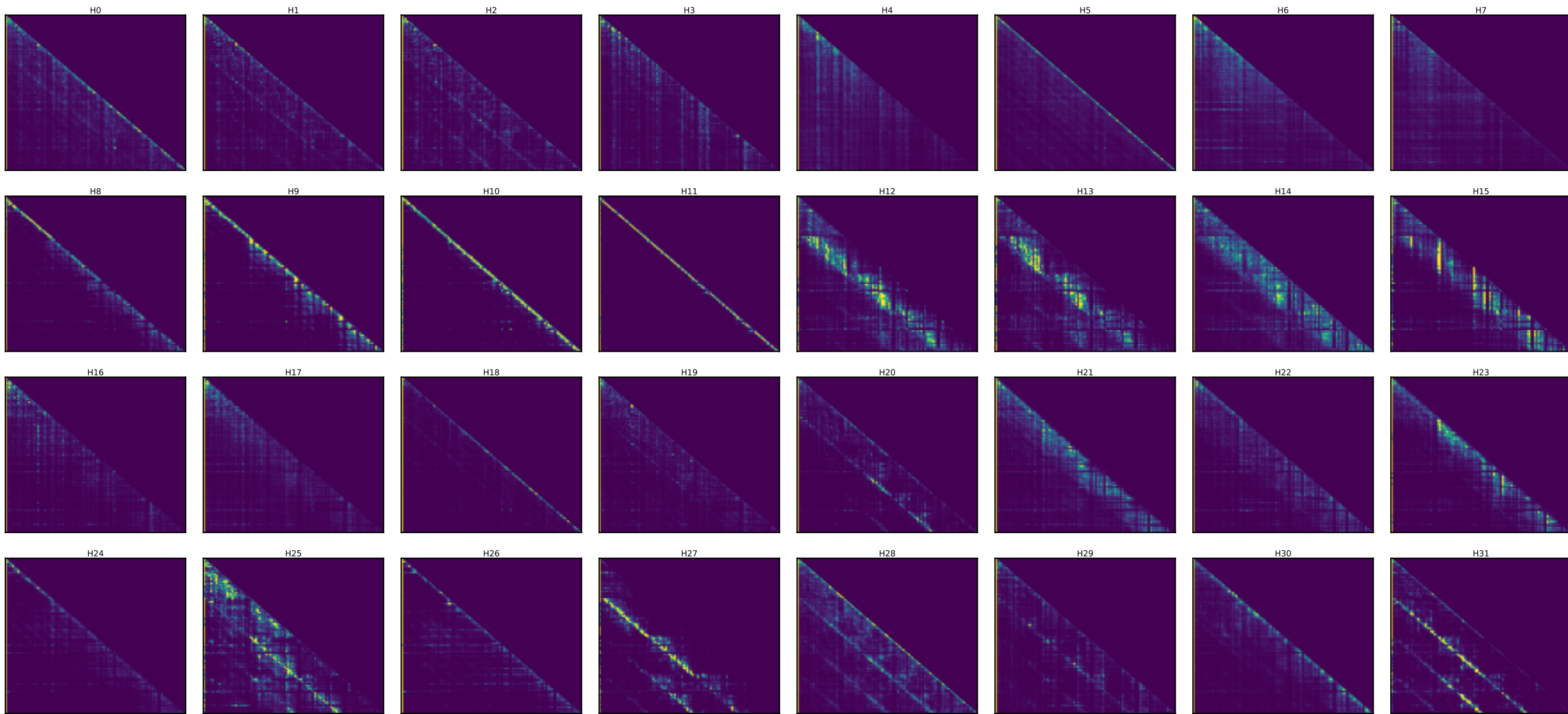
Llama layer 9 — every head's attention [25 random toks x4 + SOS] (induction stripe = diagonal at key=query-25)
