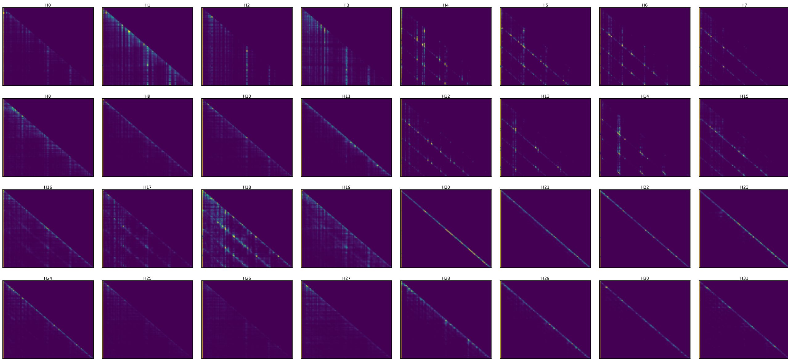
Llama layer 25 — every head's attention [25 random toks x4 + SOS] (induction stripe = diagonal at key=query-25)
