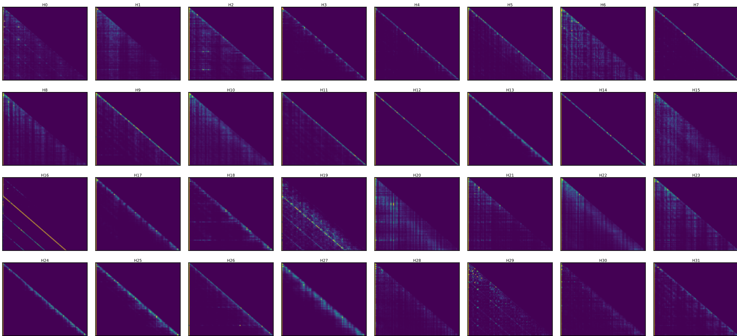
Llama layer 4 — every head's attention [25 random toks x4 + SOS] (induction stripe = diagonal at key=query-25)
