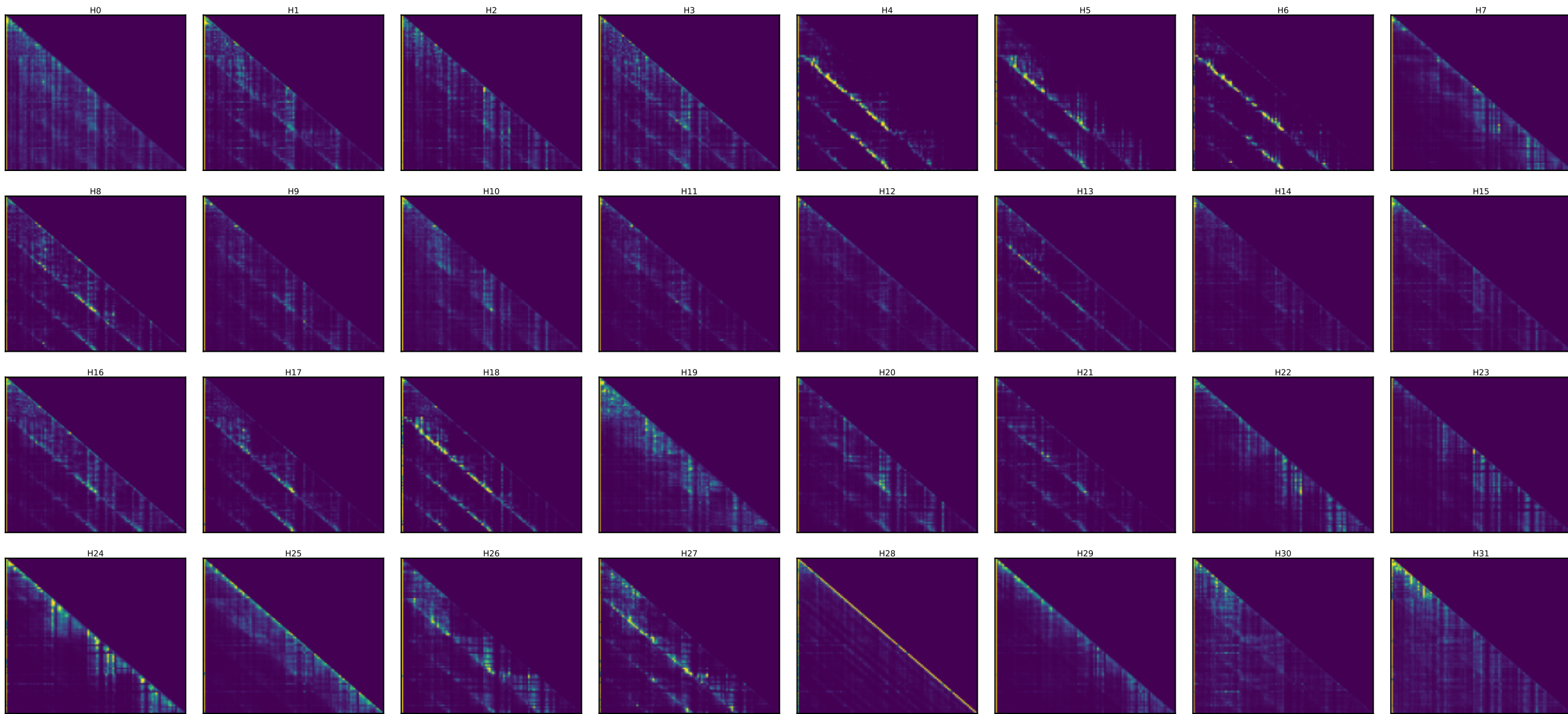
Llama layer 13 — every head's attention [25 random toks x4 + SOS] (induction stripe = diagonal at key=query-25)
