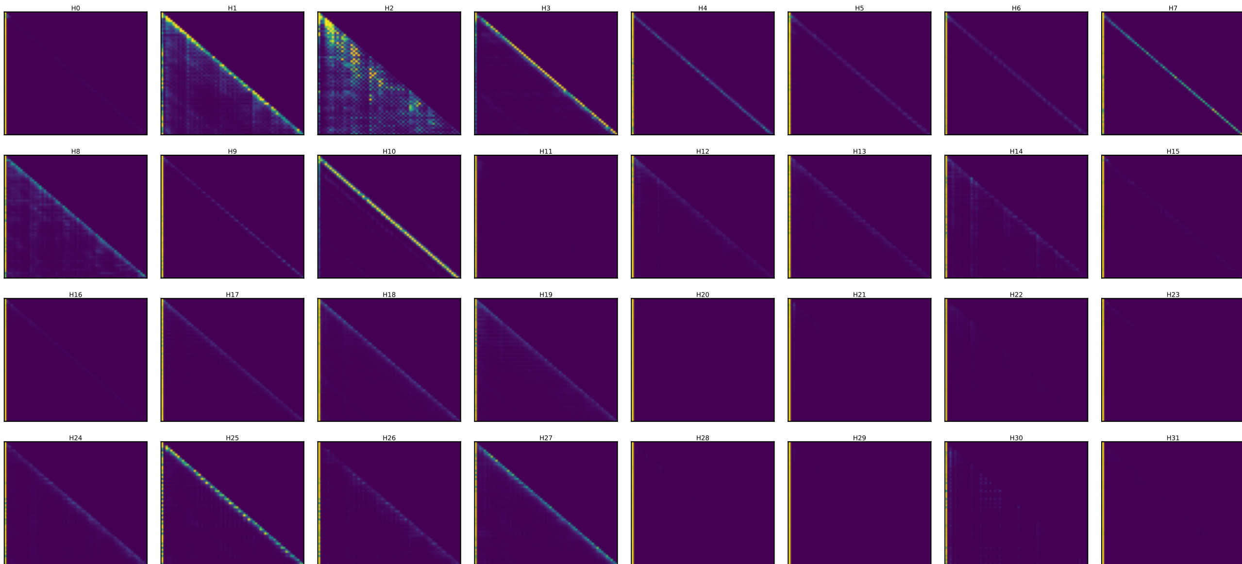
Llama layer 21 — every head's attention [days walk (60 steps)] (induction stripe = diagonal at key=query-25)
