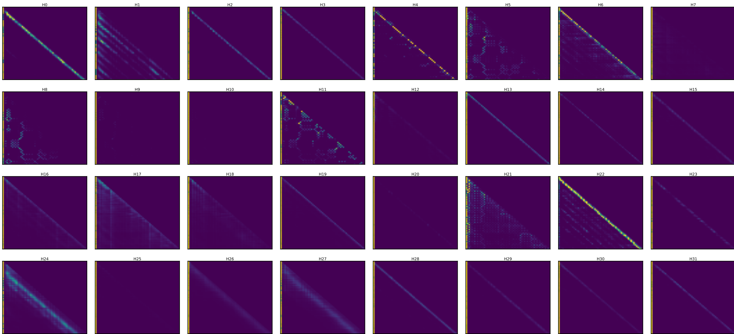
Llama layer 5 — every head's attention [days walk (60 steps)] (induction stripe = diagonal at key=query-25)
