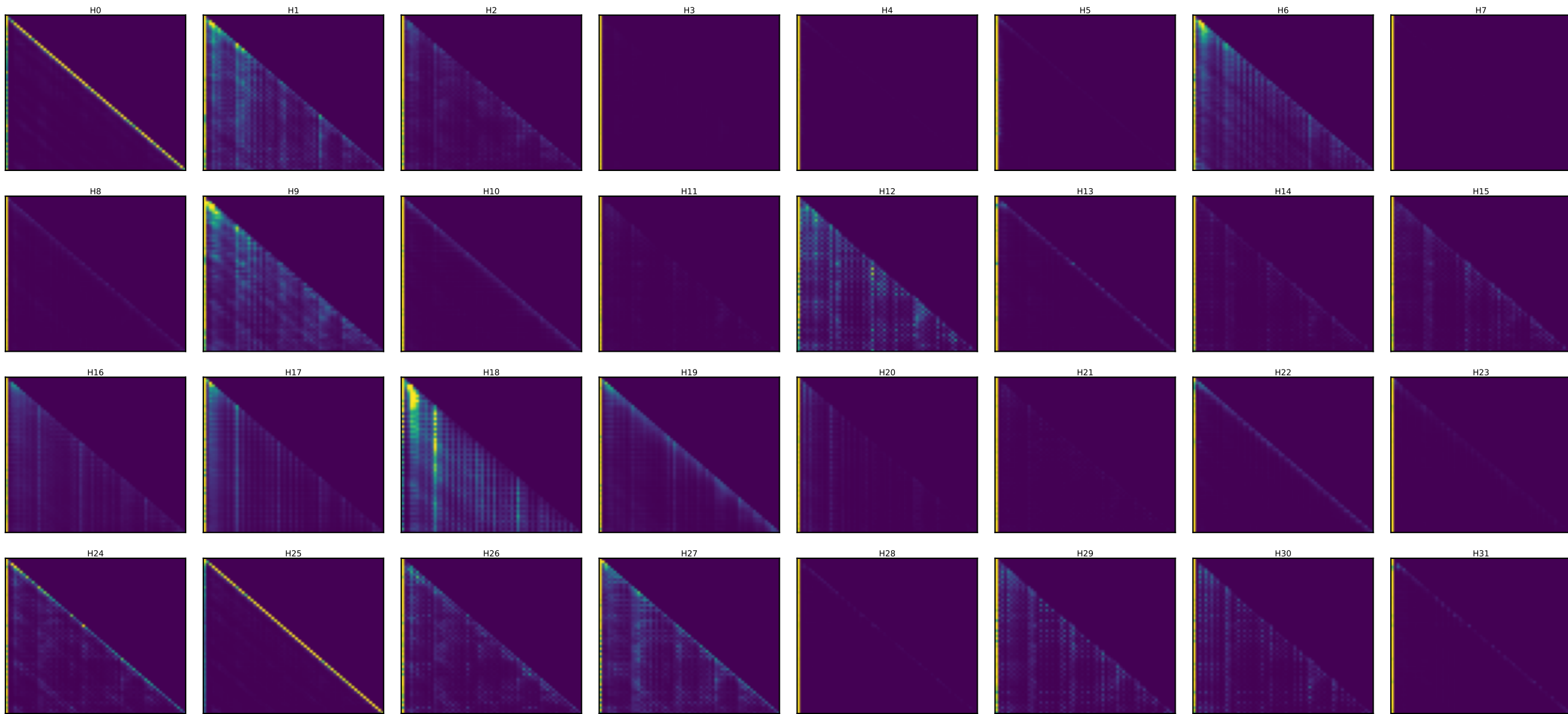
Llama layer 30 — every head's attention [days walk (60 steps)] (induction stripe = diagonal at key=query-25)
