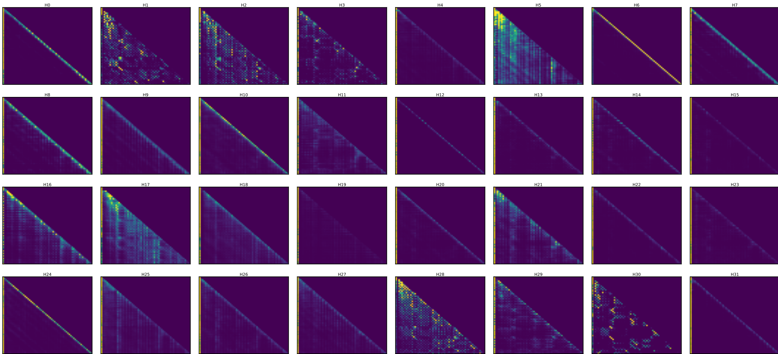
Llama layer 15 — every head's attention [days walk (60 steps)] (induction stripe = diagonal at key=query-25)
