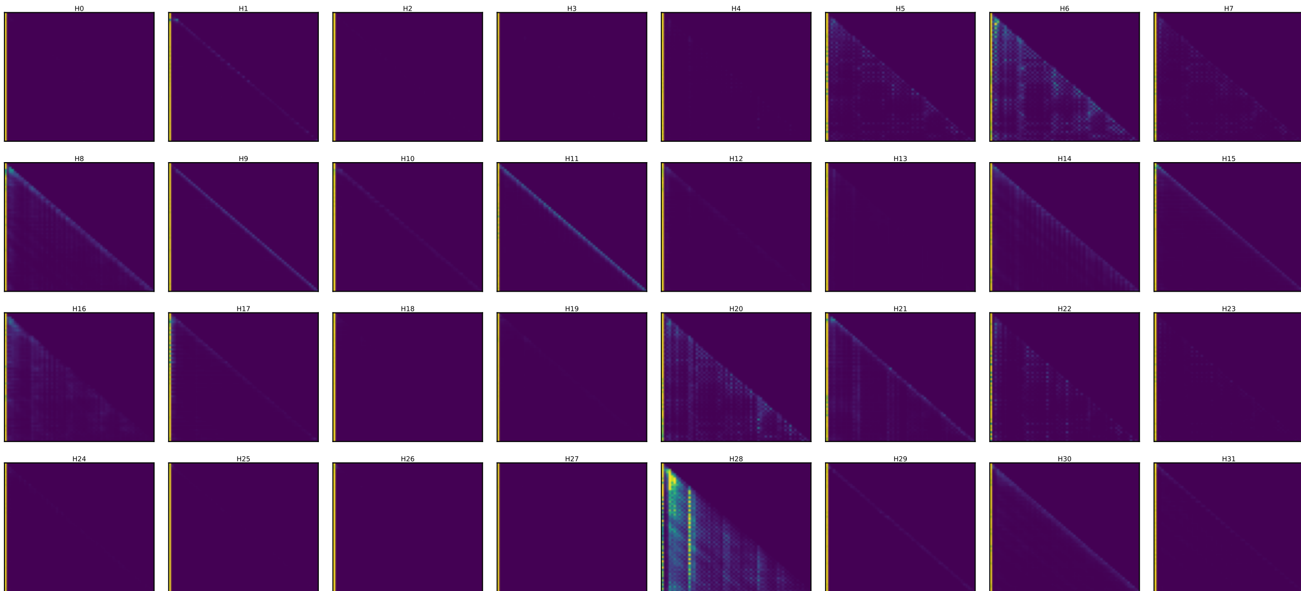
Llama layer 27 — every head's attention [days walk (60 steps)] (induction stripe = diagonal at key=query-25)
