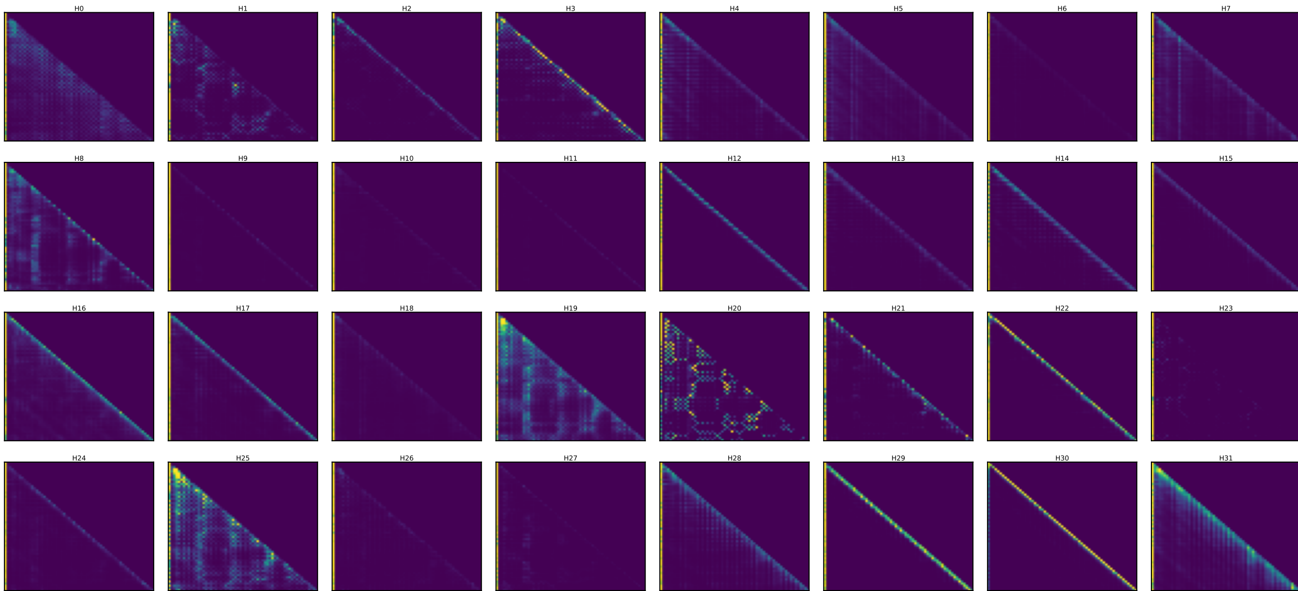
Llama layer 16 — every head's attention [days walk (60 steps)] (induction stripe = diagonal at key=query-25)
