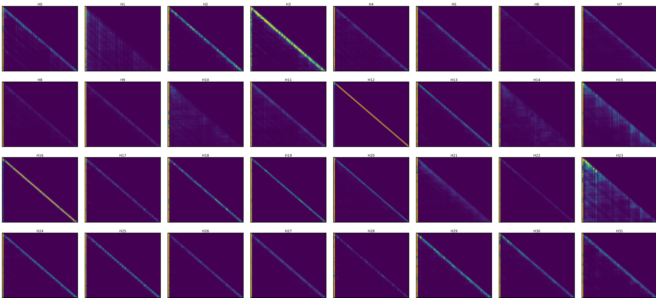
Llama layer 12 — every head's attention [days walk (60 steps)] (induction stripe = diagonal at key=query-25)
