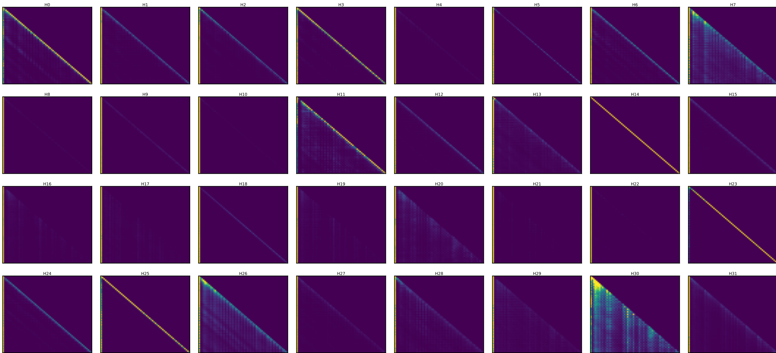
Llama layer 31 — every head's attention [days walk (60 steps)] (induction stripe = diagonal at key=query-25)
