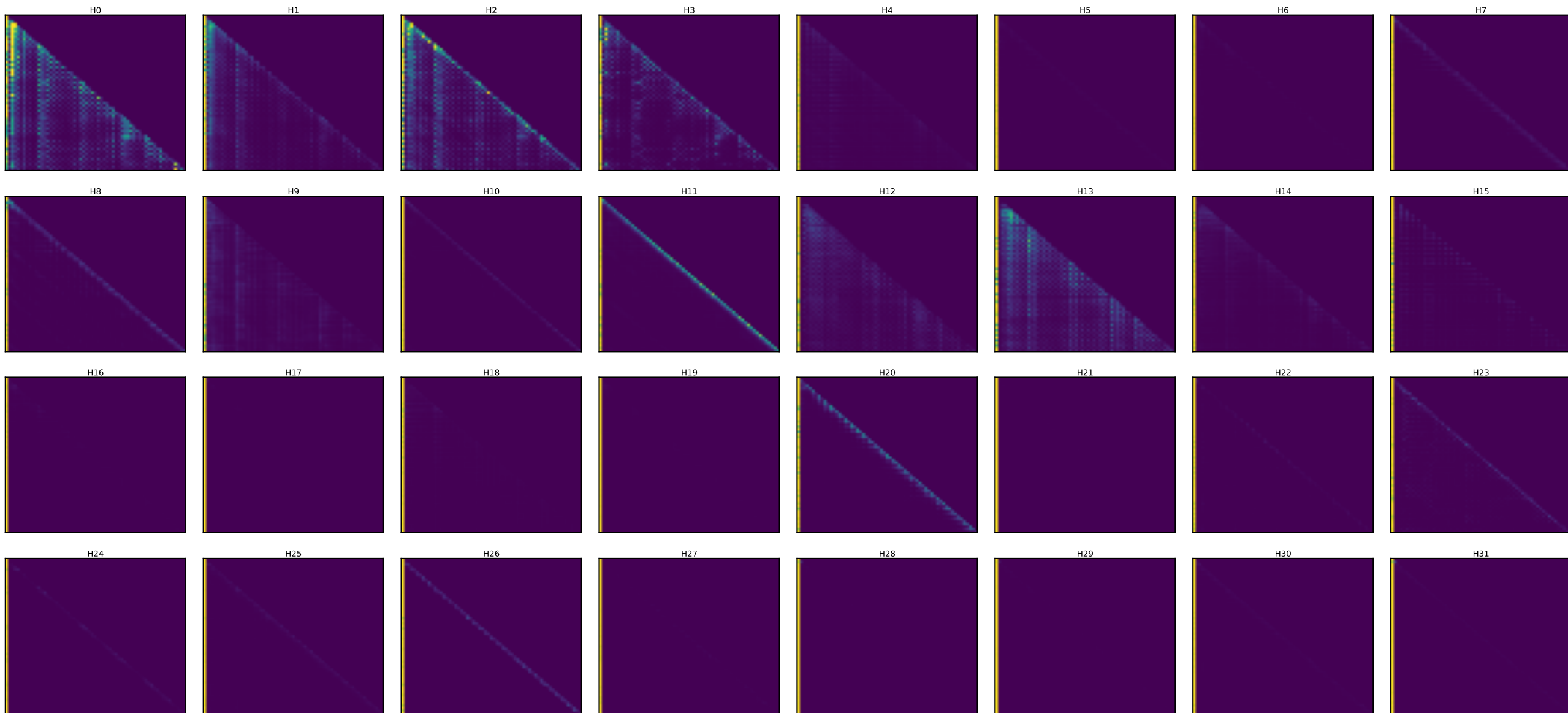
Llama layer 19 — every head's attention [days walk (60 steps)] (induction stripe = diagonal at key=query-25)
