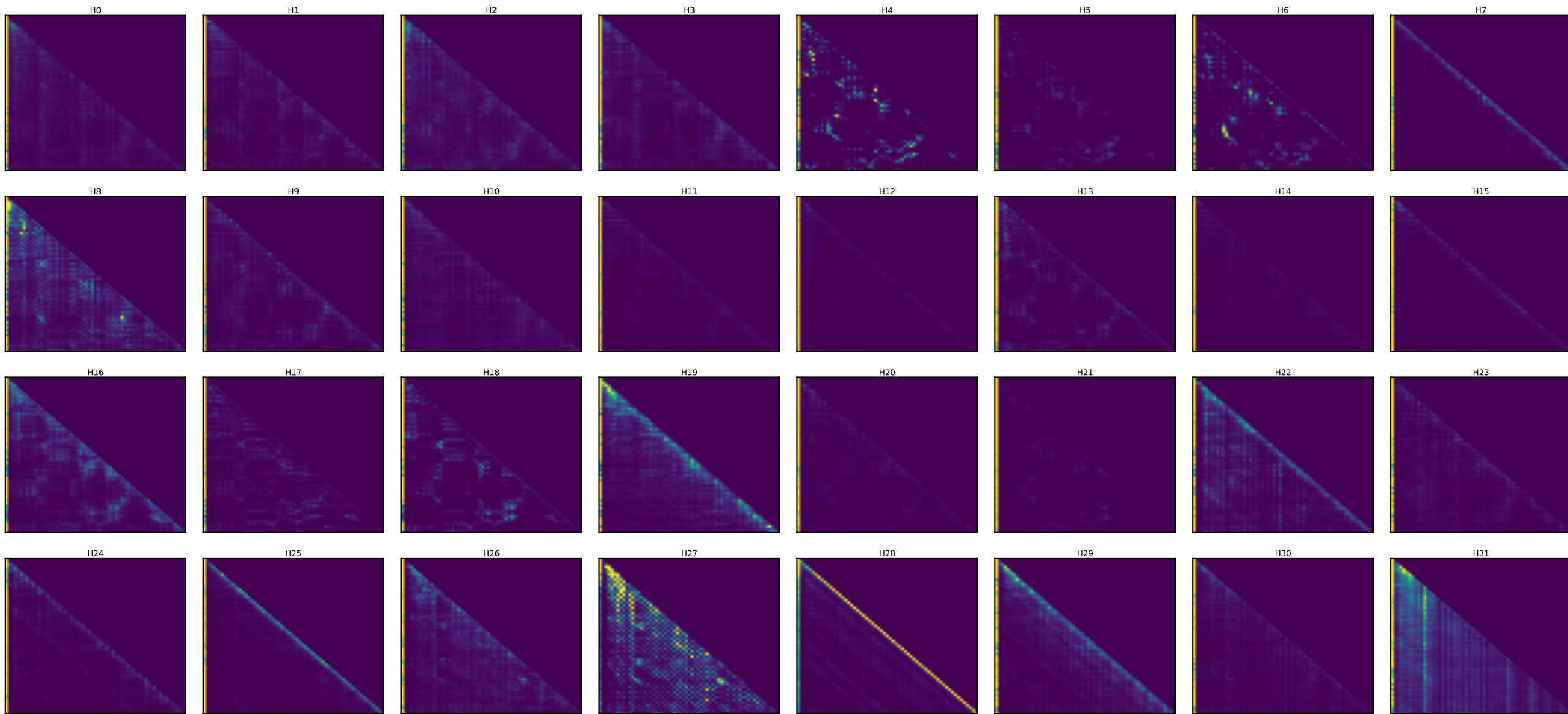
Llama layer 13 — every head's attention [days walk (60 steps)] (induction stripe = diagonal at key=query-25)
