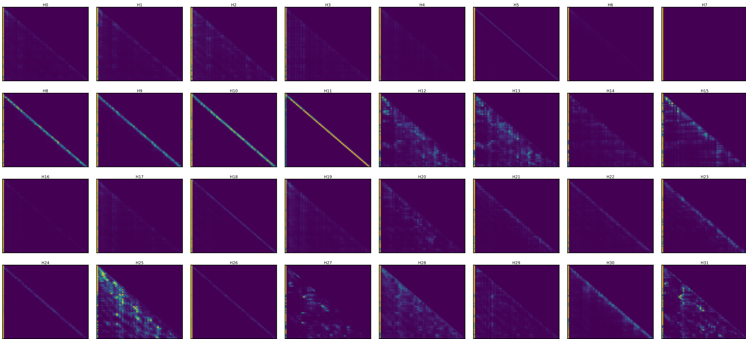
Llama layer 9 — every head's attention [days walk (60 steps)] (induction stripe = diagonal at key=query-25)
