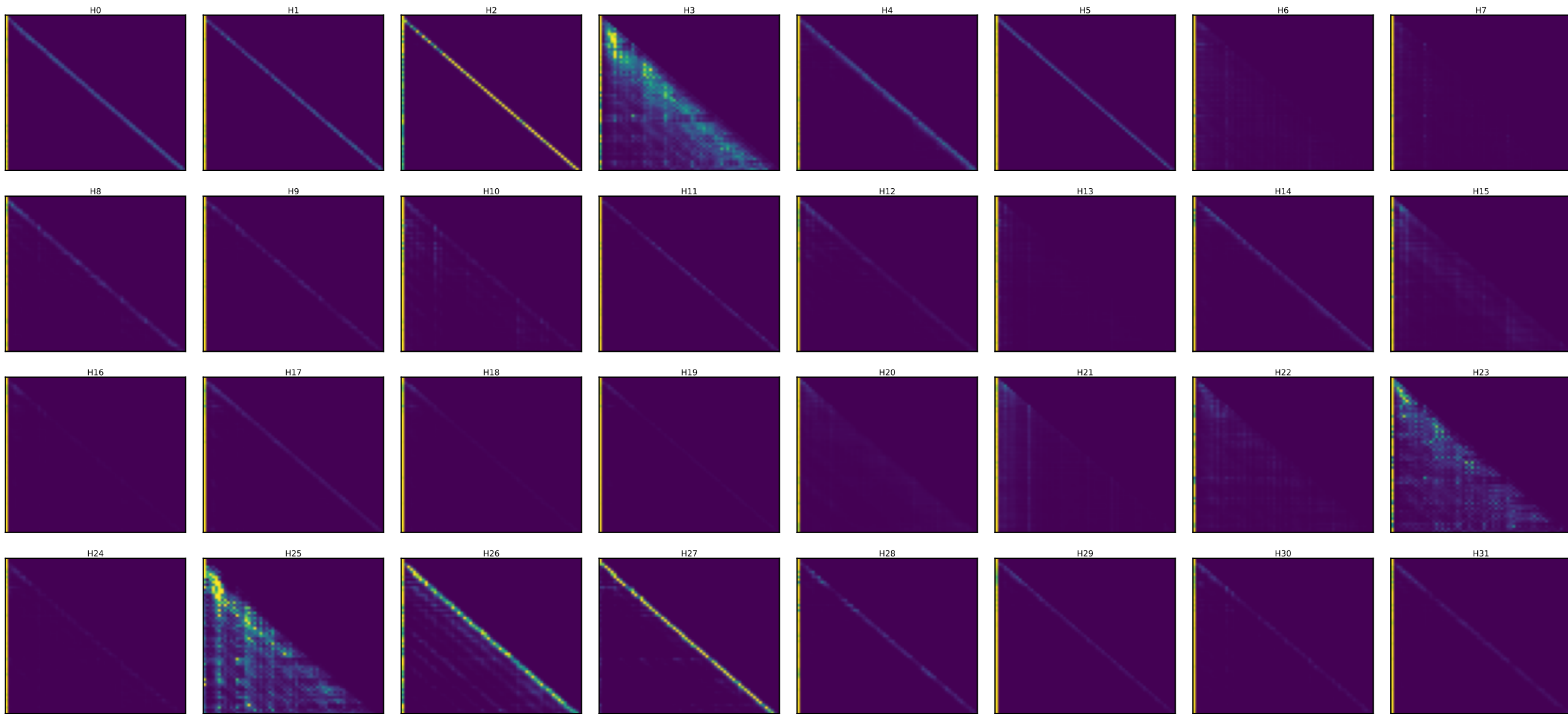
Llama layer 7 — every head's attention [days walk (60 steps)] (induction stripe = diagonal at key=query-25)
