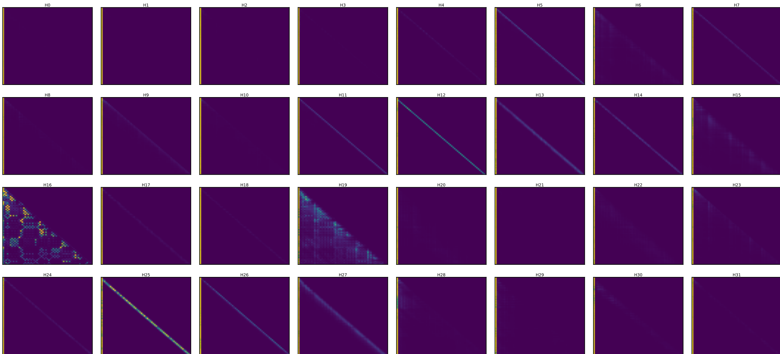
Llama layer 4 — every head's attention [days walk (60 steps)] (induction stripe = diagonal at key=query-25)
