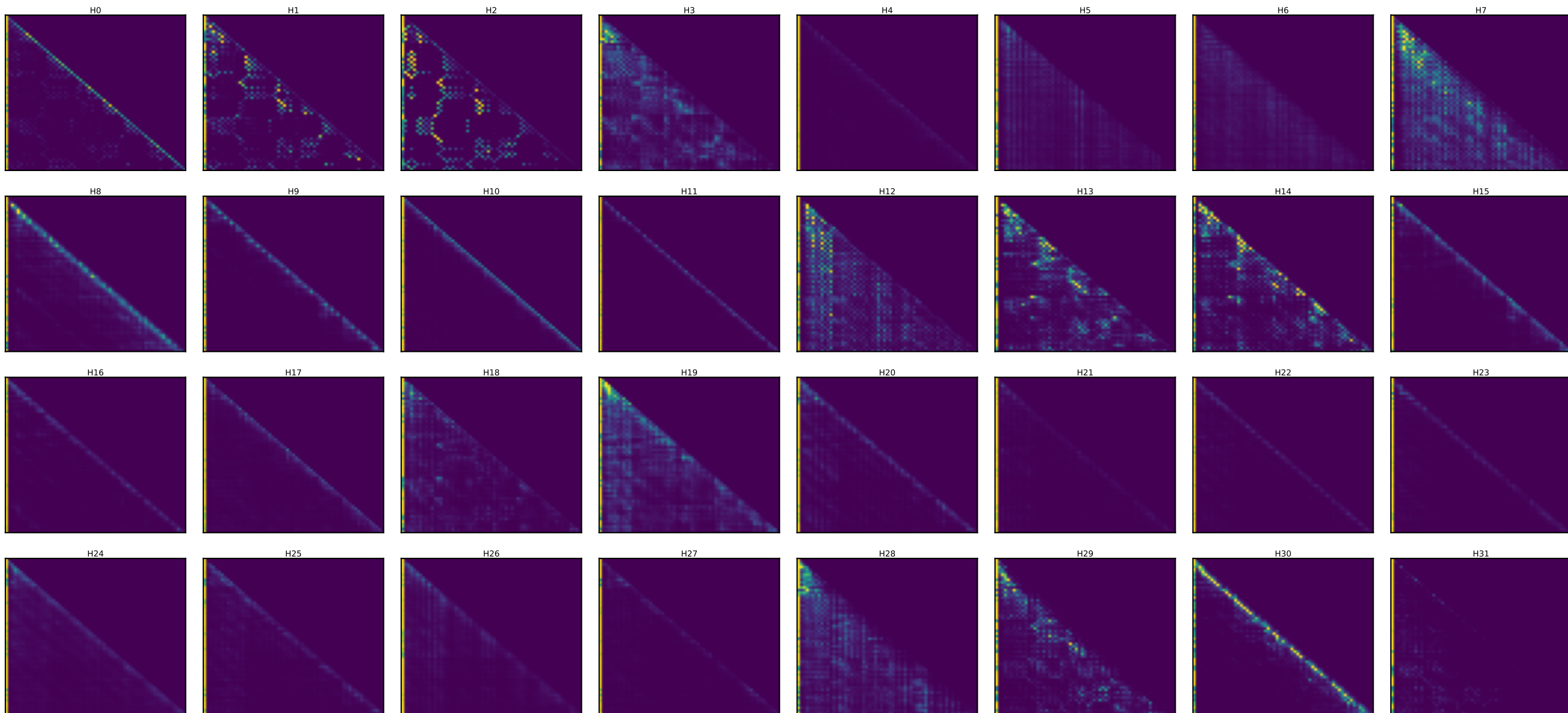
Llama layer 10 — every head's attention [days walk (60 steps)] (induction stripe = diagonal at key=query-25)
