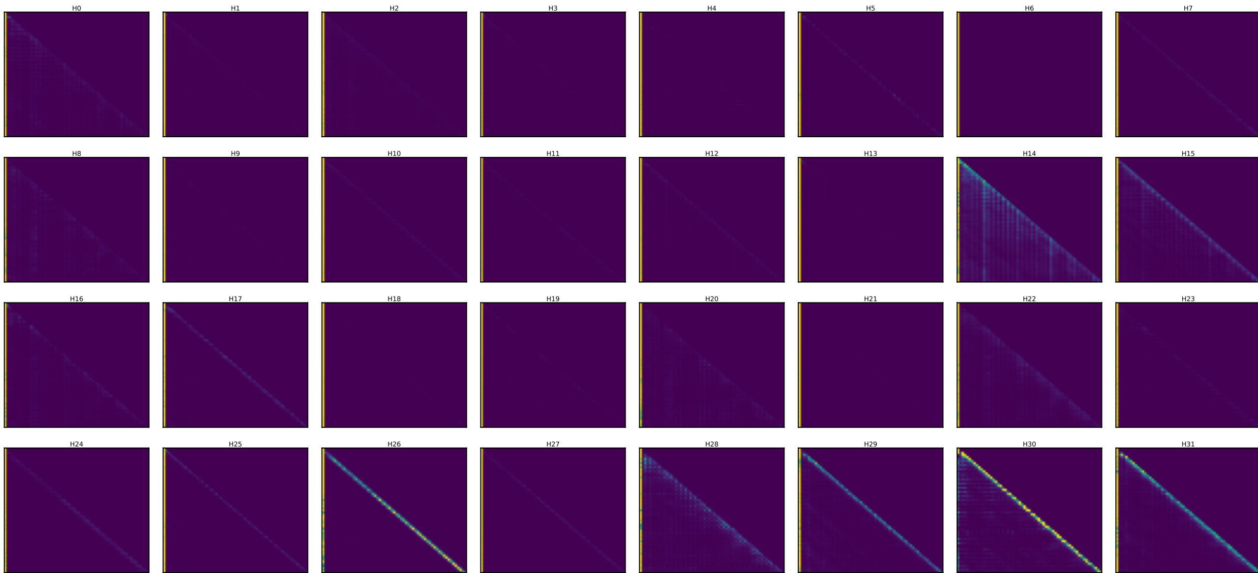
Llama layer 18 — every head's attention [days walk (60 steps)] (induction stripe = diagonal at key=query-25)
