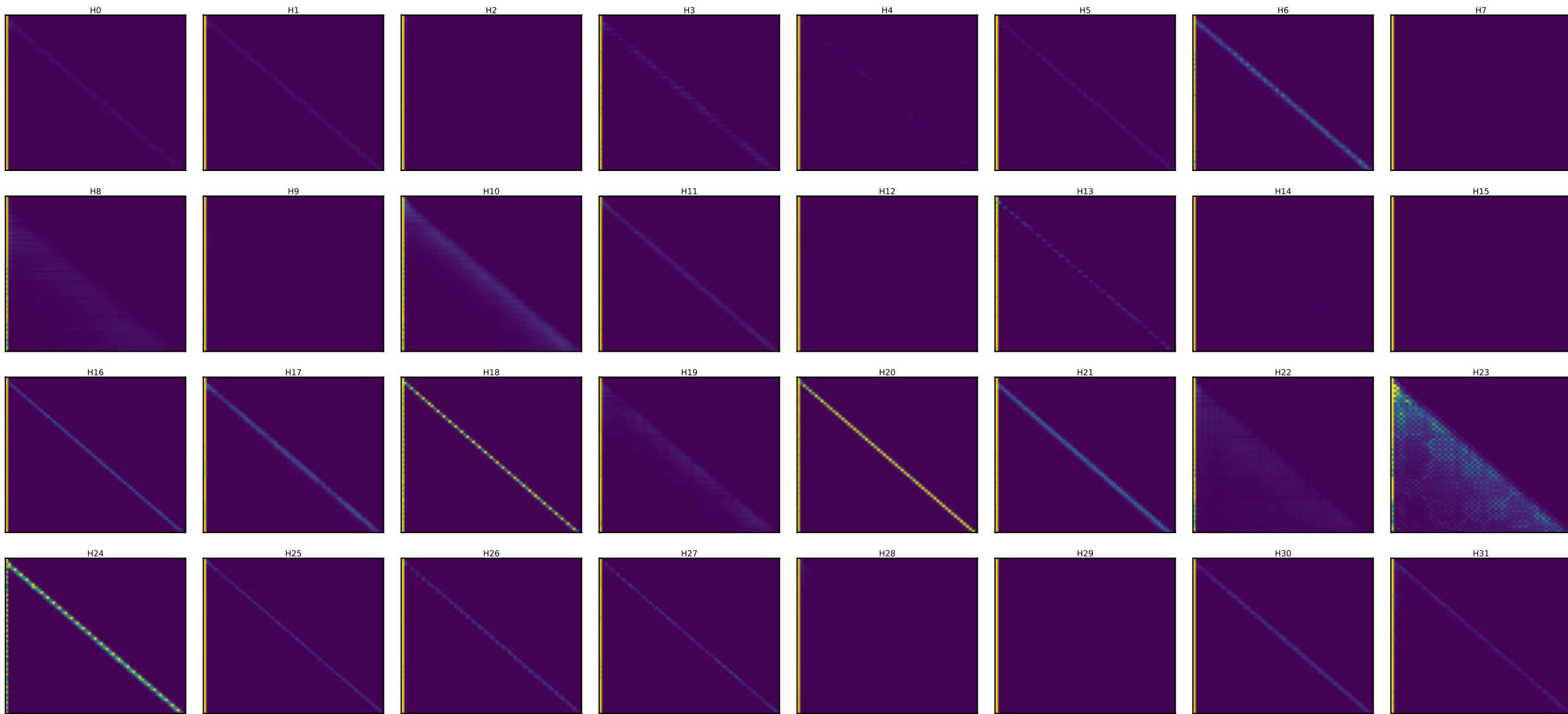
Llama layer 1 — every head's attention [days walk (60 steps)] (induction stripe = diagonal at key=query-25)
