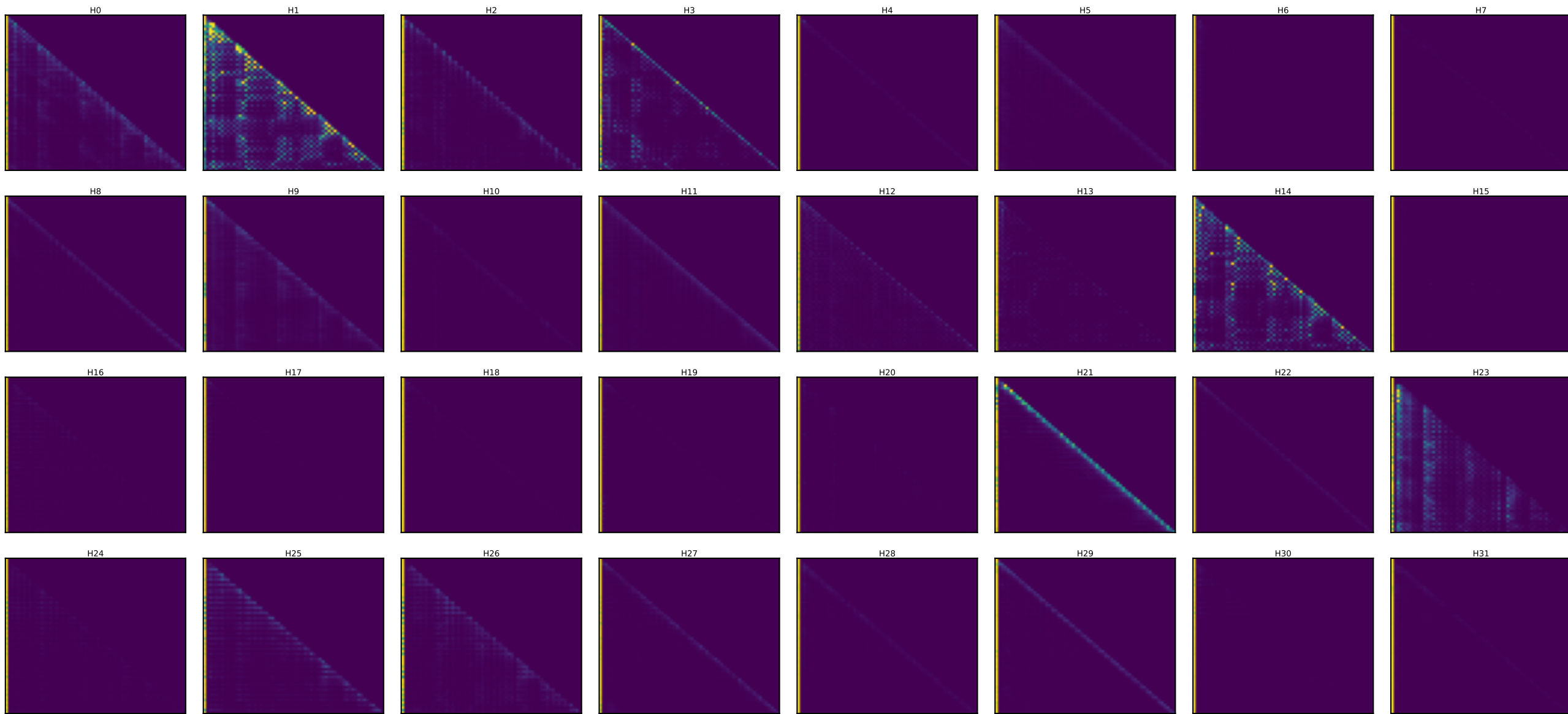
Llama layer 20 — every head's attention [days walk (60 steps)] (induction stripe = diagonal at key=query-25)
