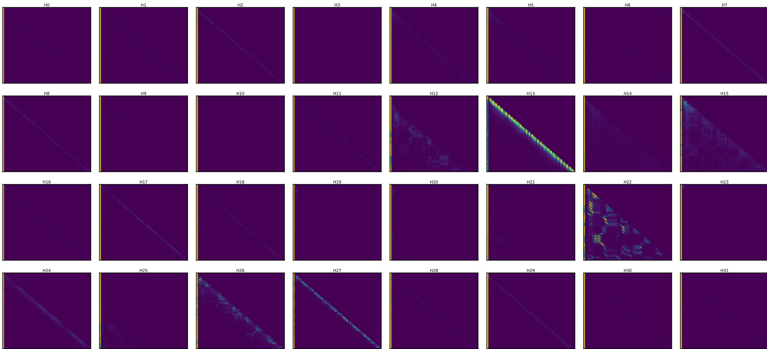
Llama layer 2 — every head's attention [days walk (60 steps)] (induction stripe = diagonal at key=query-25)
