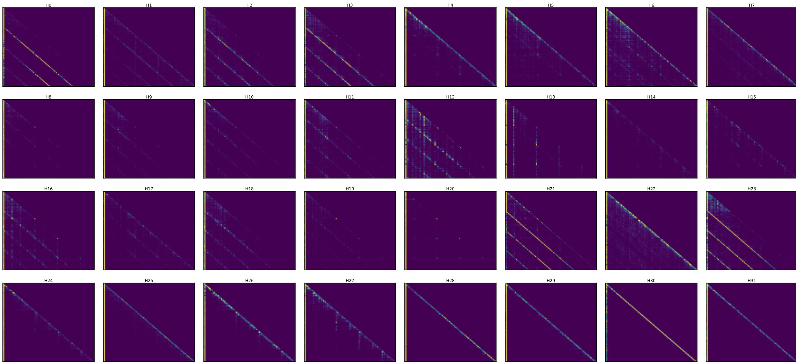
Qwen layer 28 — every head's attention [25 random toks x4 + SOS] (induction stripe = diagonal at key=query-25)
