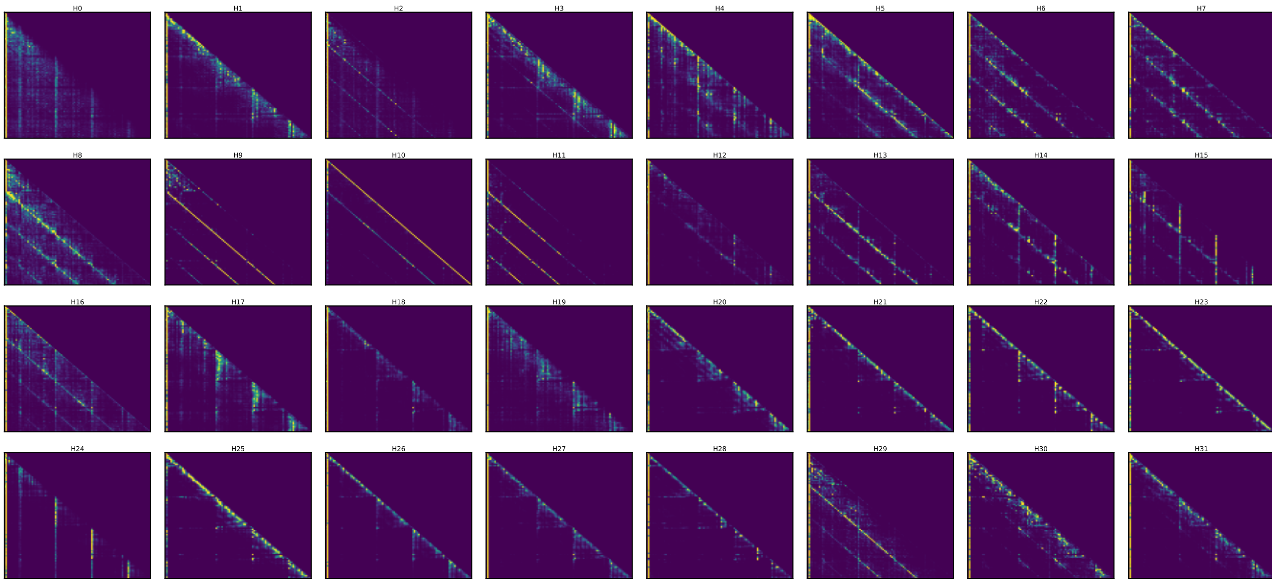
Qwen layer 15 — every head's attention [25 random toks x4 + SOS] (induction stripe = diagonal at key=query-25)
