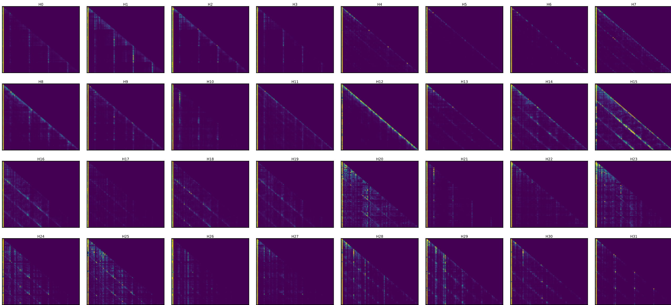
Qwen layer 27 — every head's attention [25 random toks x4 + SOS] (induction stripe = diagonal at key=query-25)
