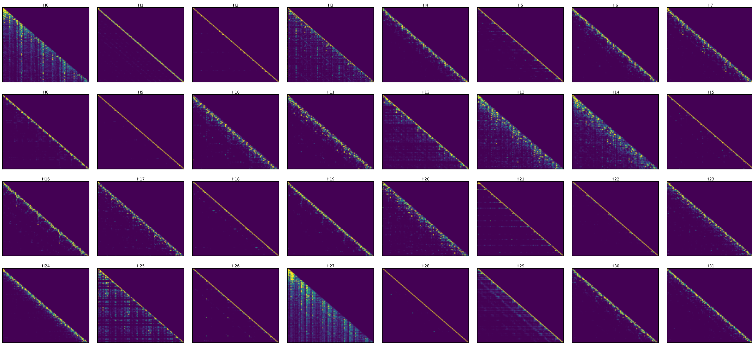
Qwen layer 0 — every head's attention [25 random toks x4 + SOS] (induction stripe = diagonal at key=query-25)
