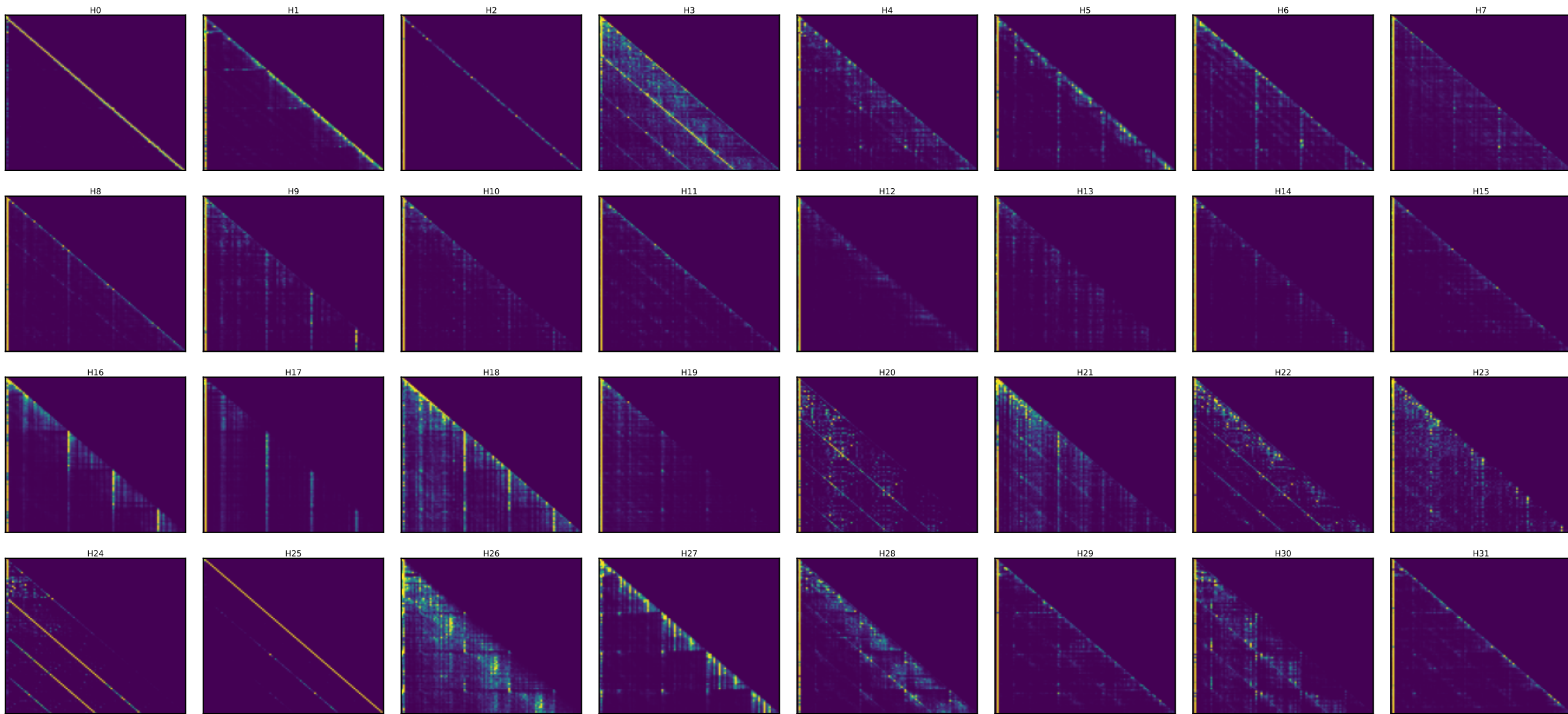
Qwen layer 12 — every head's attention [25 random toks x4 + SOS] (induction stripe = diagonal at key=query-25)
