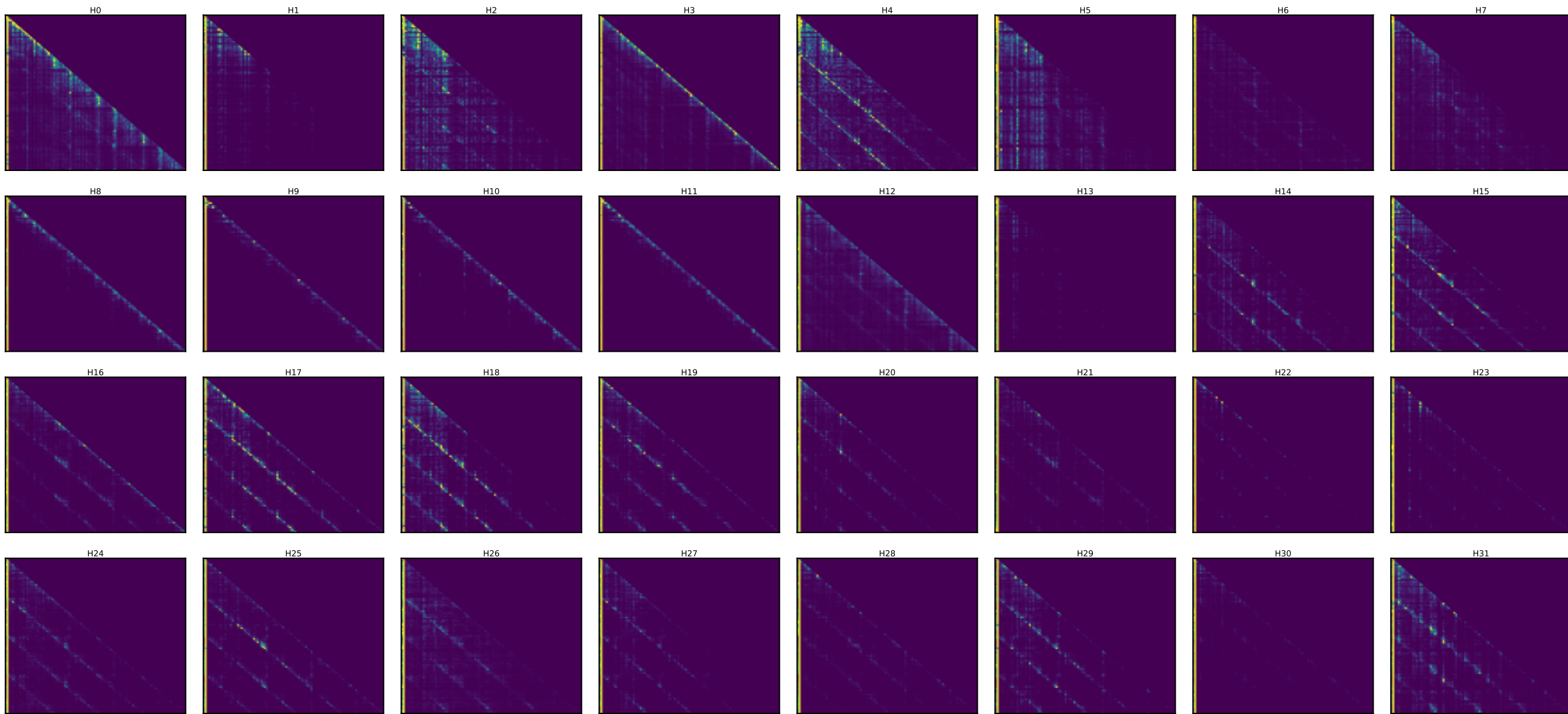
Qwen layer 26 — every head's attention [25 random toks x4 + SOS] (induction stripe = diagonal at key=query-25)
