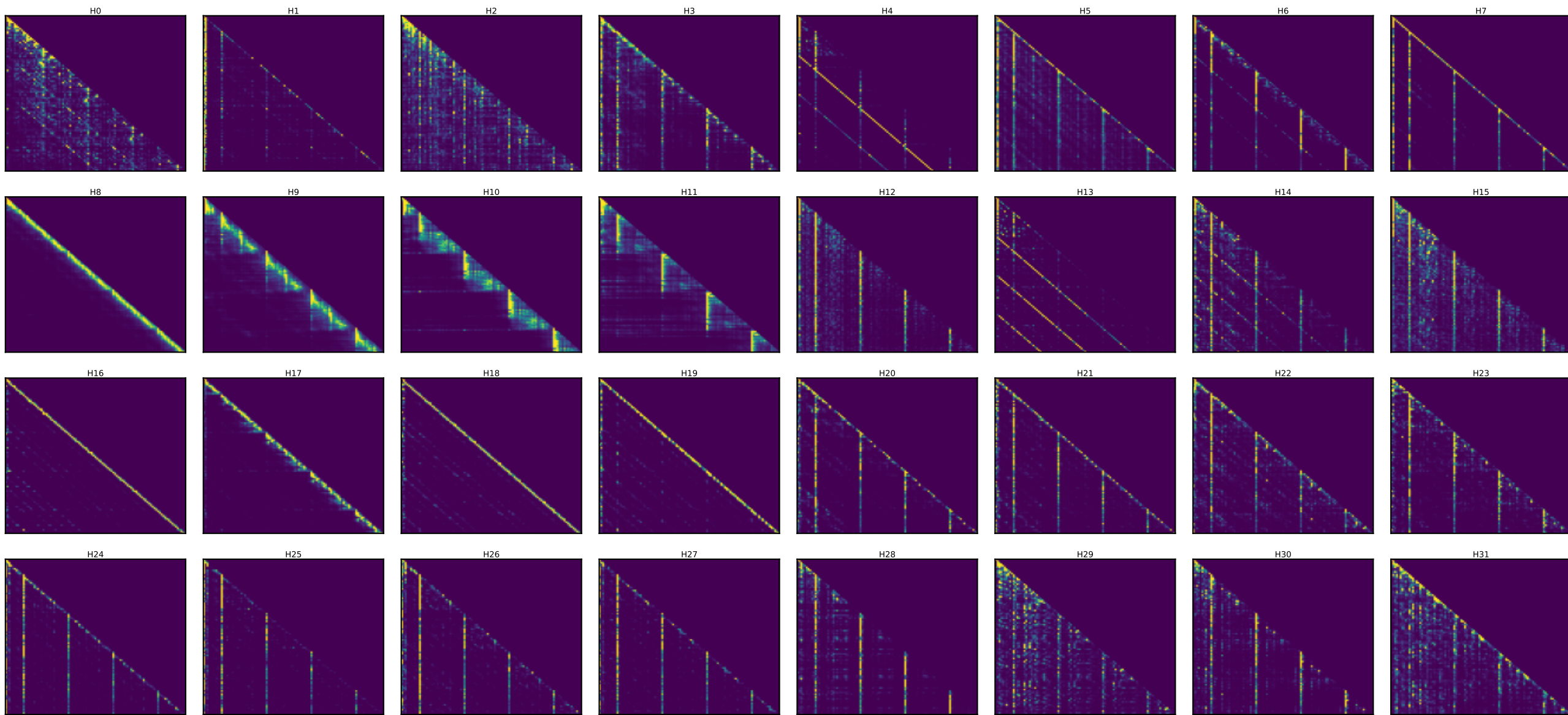
Qwen layer 5 — every head's attention [25 random toks x4 + SOS] (induction stripe = diagonal at key=query-25)
