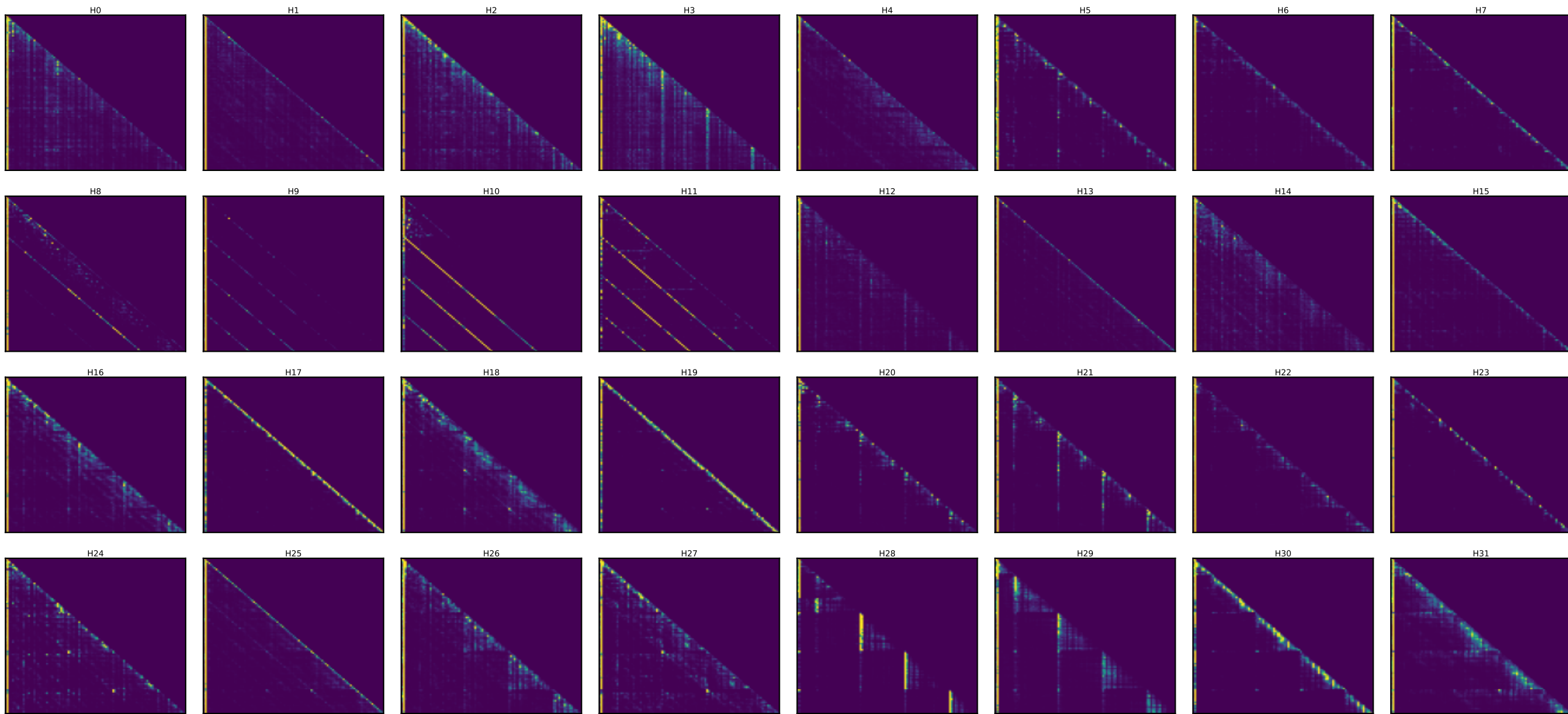
Qwen layer 11 — every head's attention [25 random toks x4 + SOS] (induction stripe = diagonal at key=query-25)
