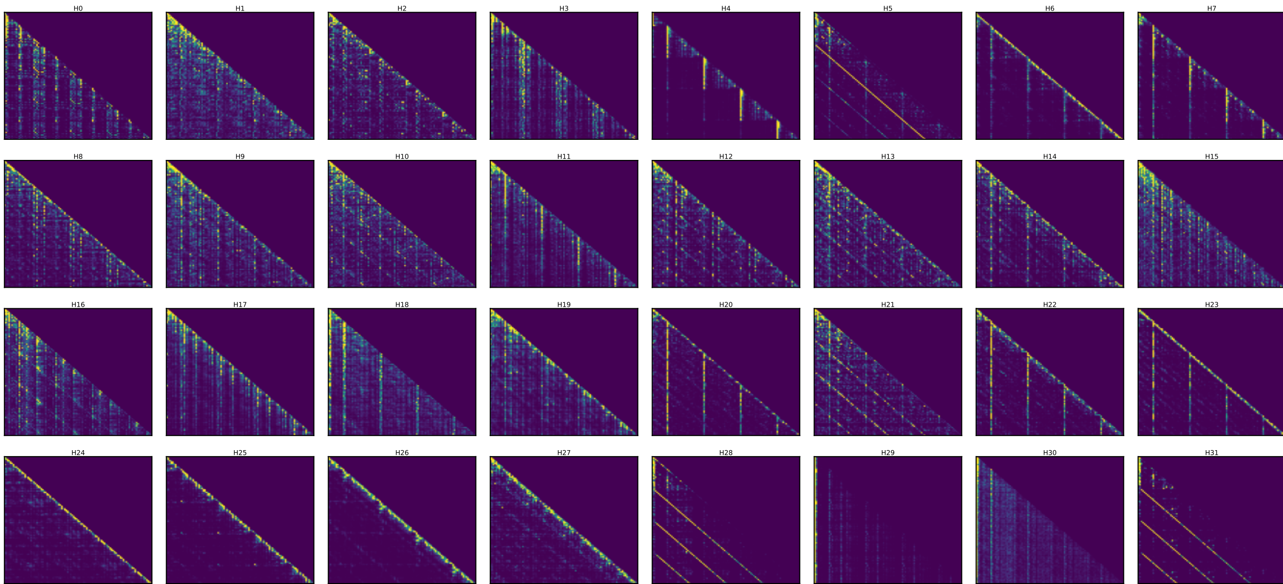
Qwen layer 2 — every head's attention [25 random toks x4 + SOS] (induction stripe = diagonal at key=query-25)
