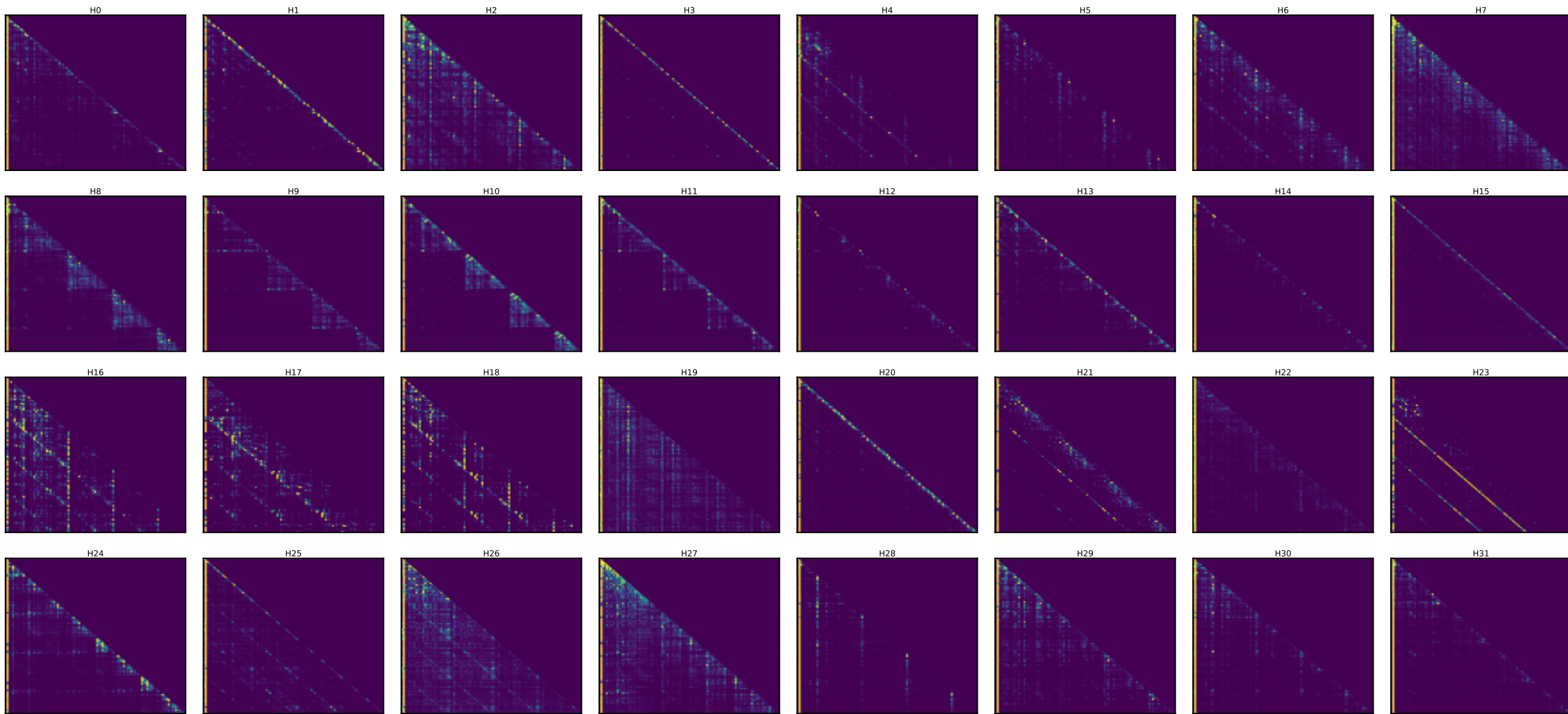
Qwen layer 8 — every head's attention [25 random toks x4 + SOS] (induction stripe = diagonal at key=query-25)
