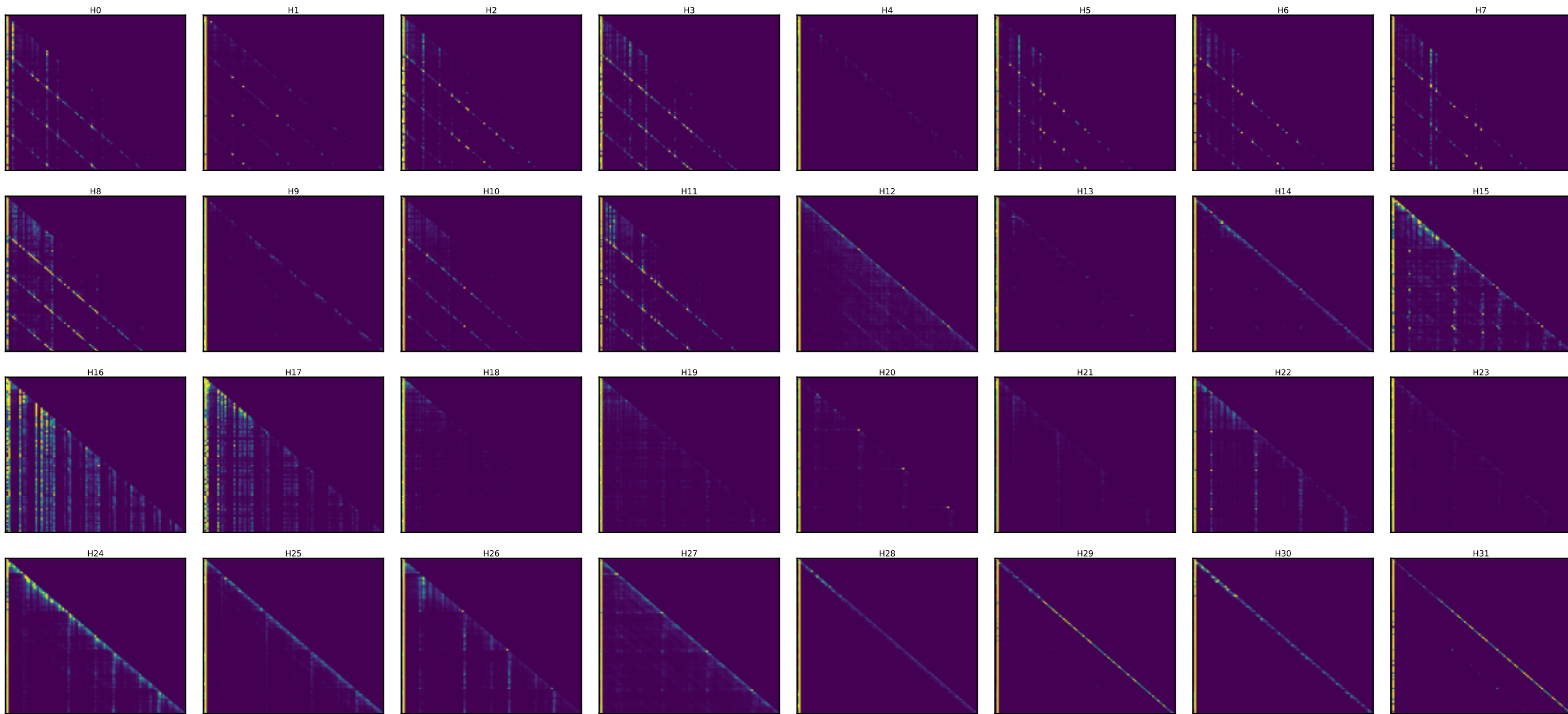
Qwen layer 32 — every head's attention [25 random toks x4 + SOS] (induction stripe = diagonal at key=query-25)
