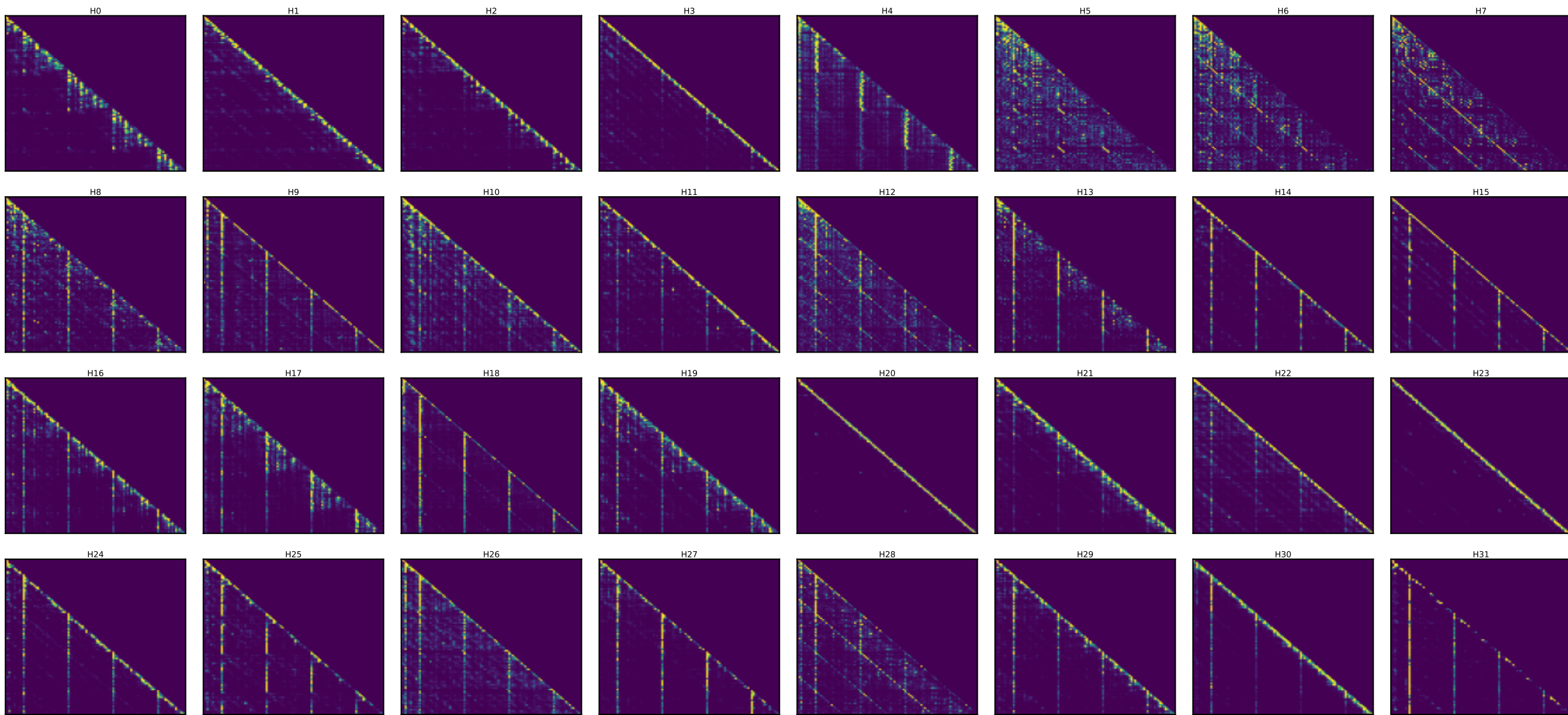
Qwen layer 6 — every head's attention [25 random toks x4 + SOS] (induction stripe = diagonal at key=query-25)
