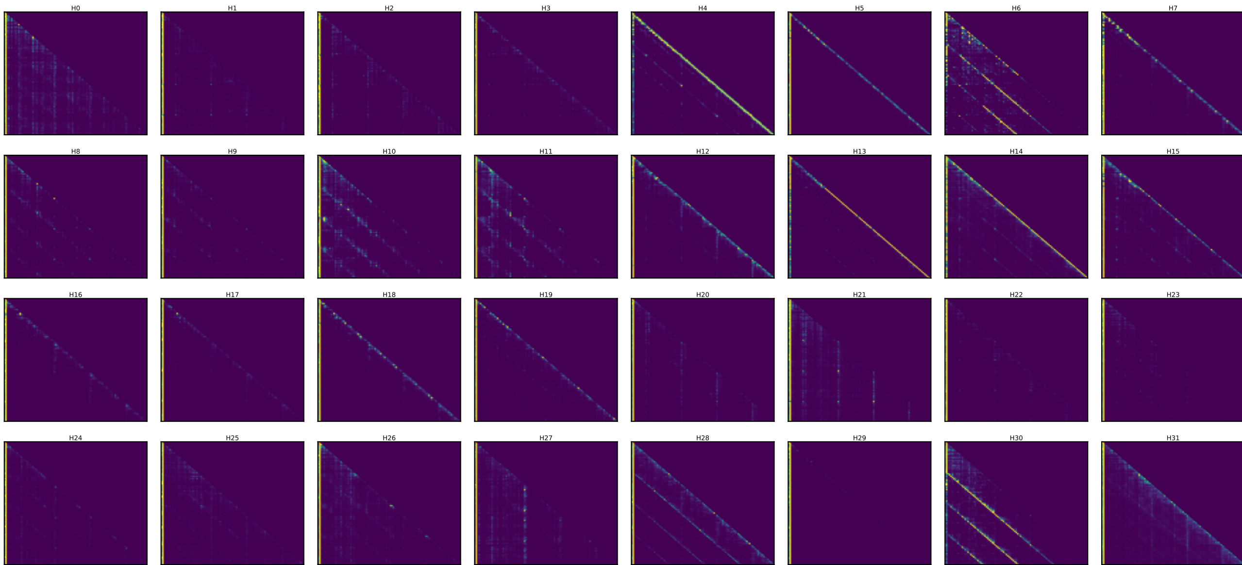
Qwen layer 25 — every head's attention [25 random toks x4 + SOS] (induction stripe = diagonal at key=query-25)
