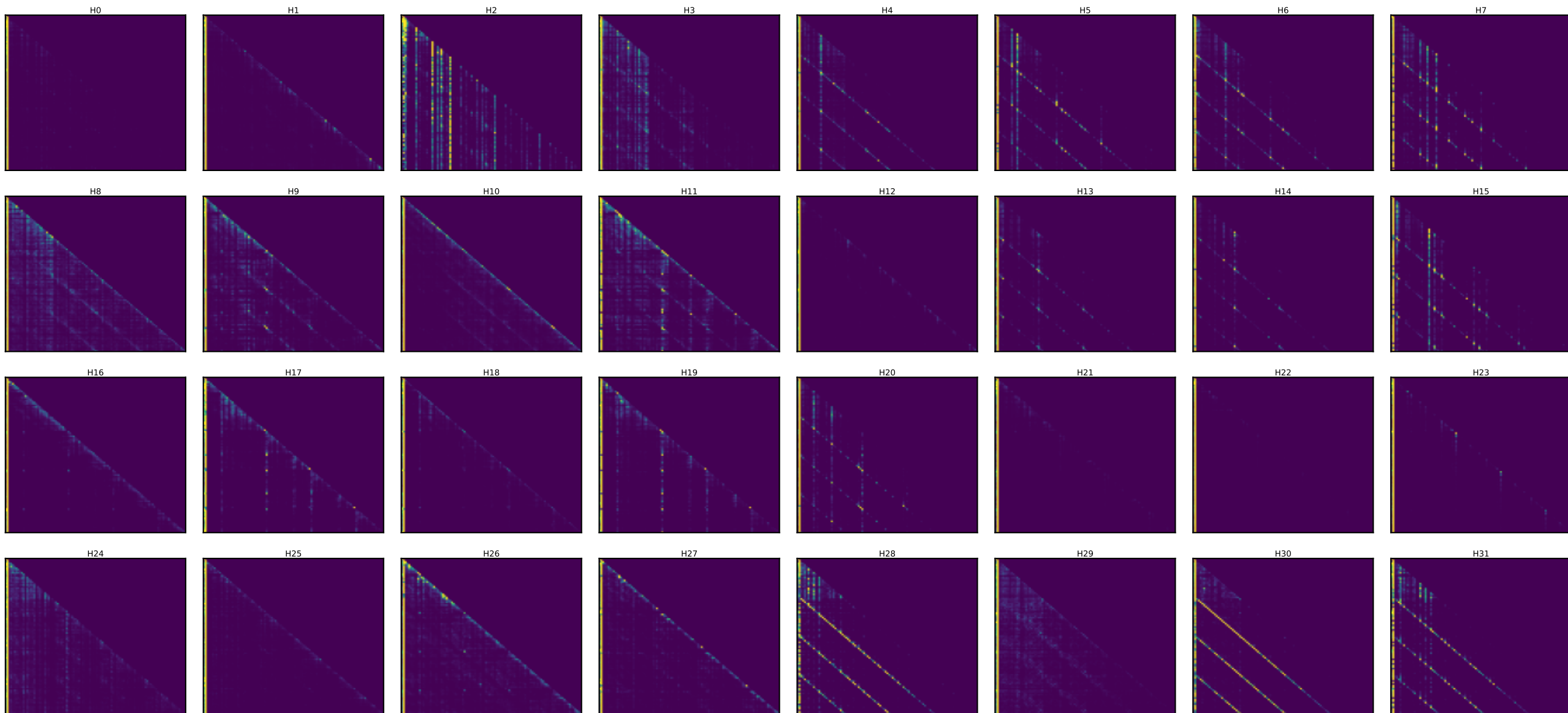
Qwen layer 31 — every head's attention [25 random toks x4 + SOS] (induction stripe = diagonal at key=query-25)
