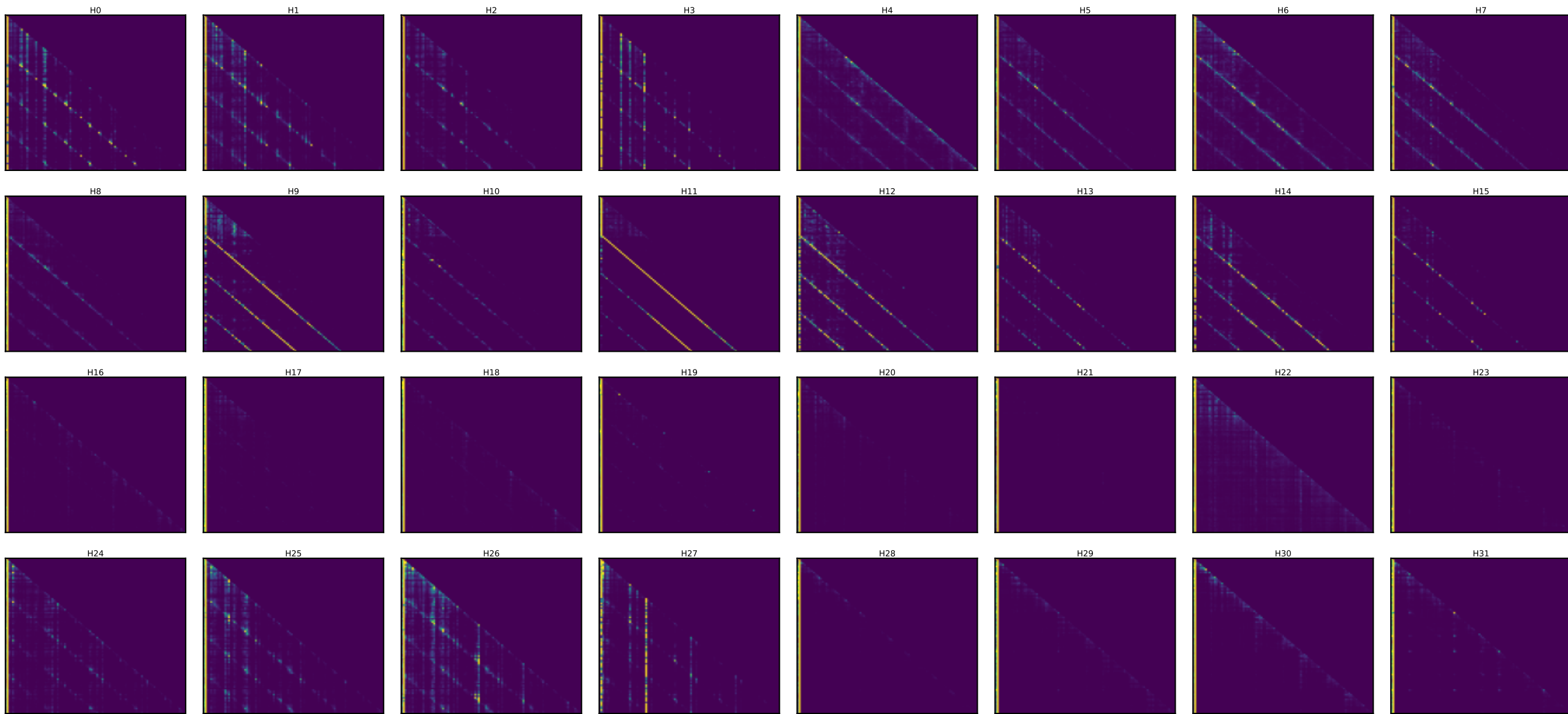
Qwen layer 29 — every head's attention [25 random toks x4 + SOS] (induction stripe = diagonal at key=query-25)
