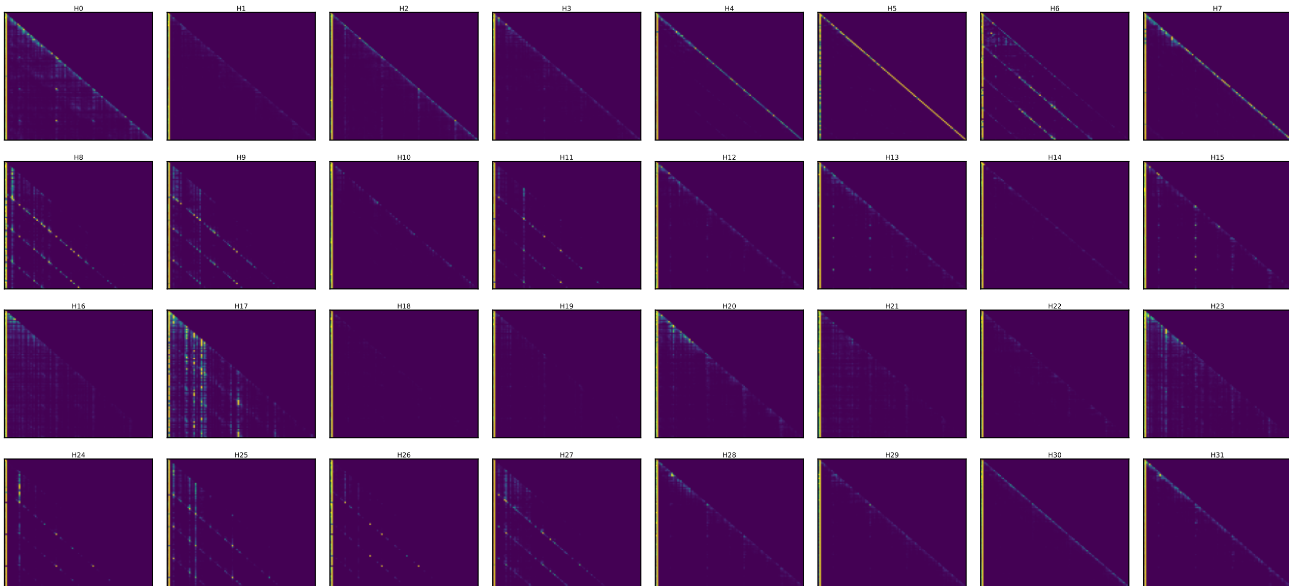
Qwen layer 30 — every head's attention [25 random toks x4 + SOS] (induction stripe = diagonal at key=query-25)
