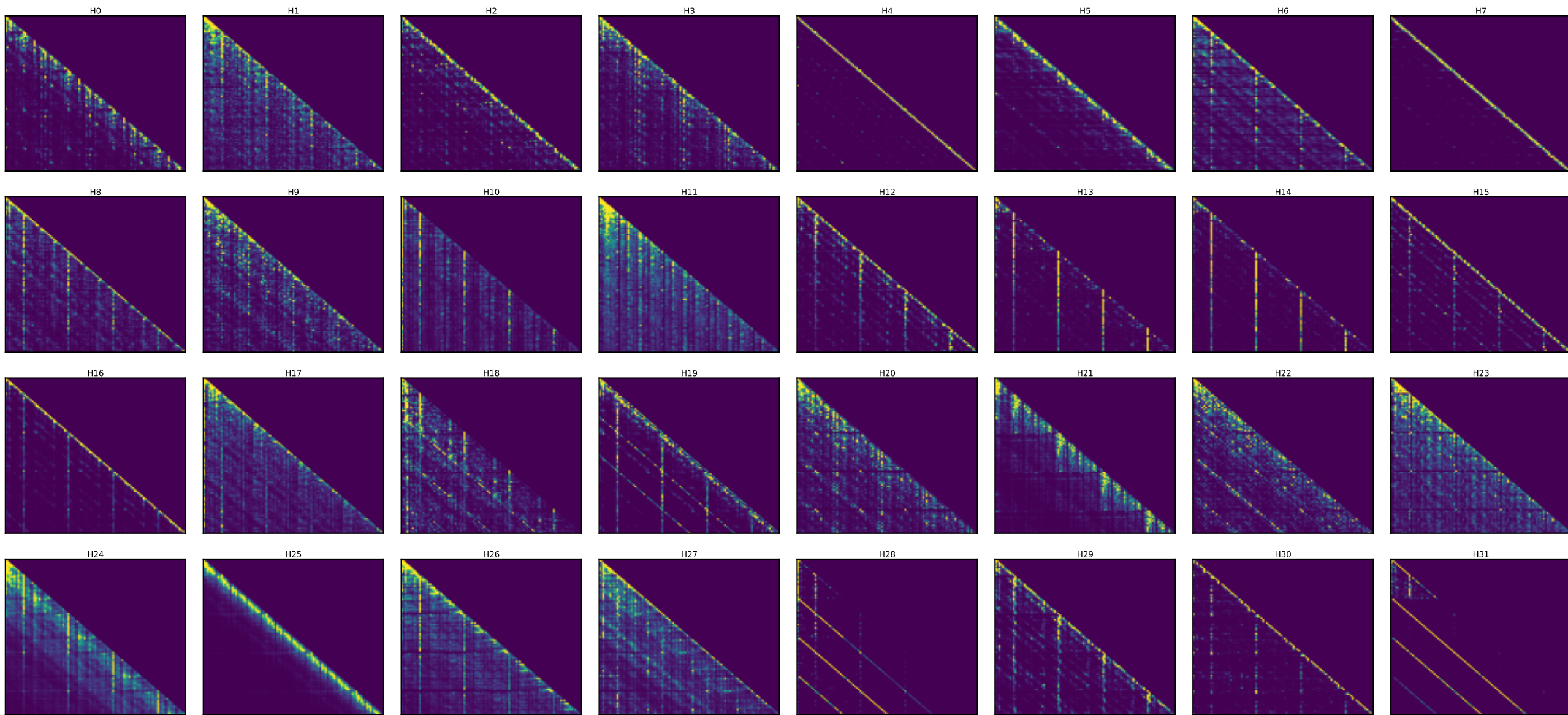
Qwen layer 1 — every head's attention [25 random toks x4 + SOS] (induction stripe = diagonal at key=query-25)
