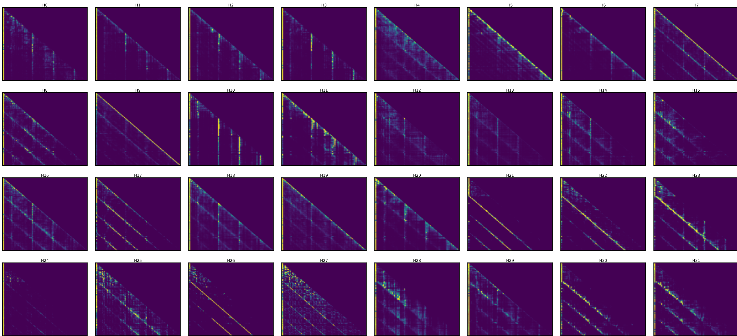
Qwen layer 20 — every head's attention [25 random toks x4 + SOS] (induction stripe = diagonal at key=query-25)
