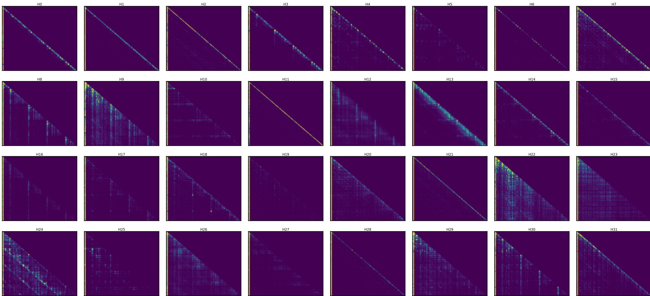
Qwen layer 10 — every head's attention [25 random toks x4 + SOS] (induction stripe = diagonal at key=query-25)
