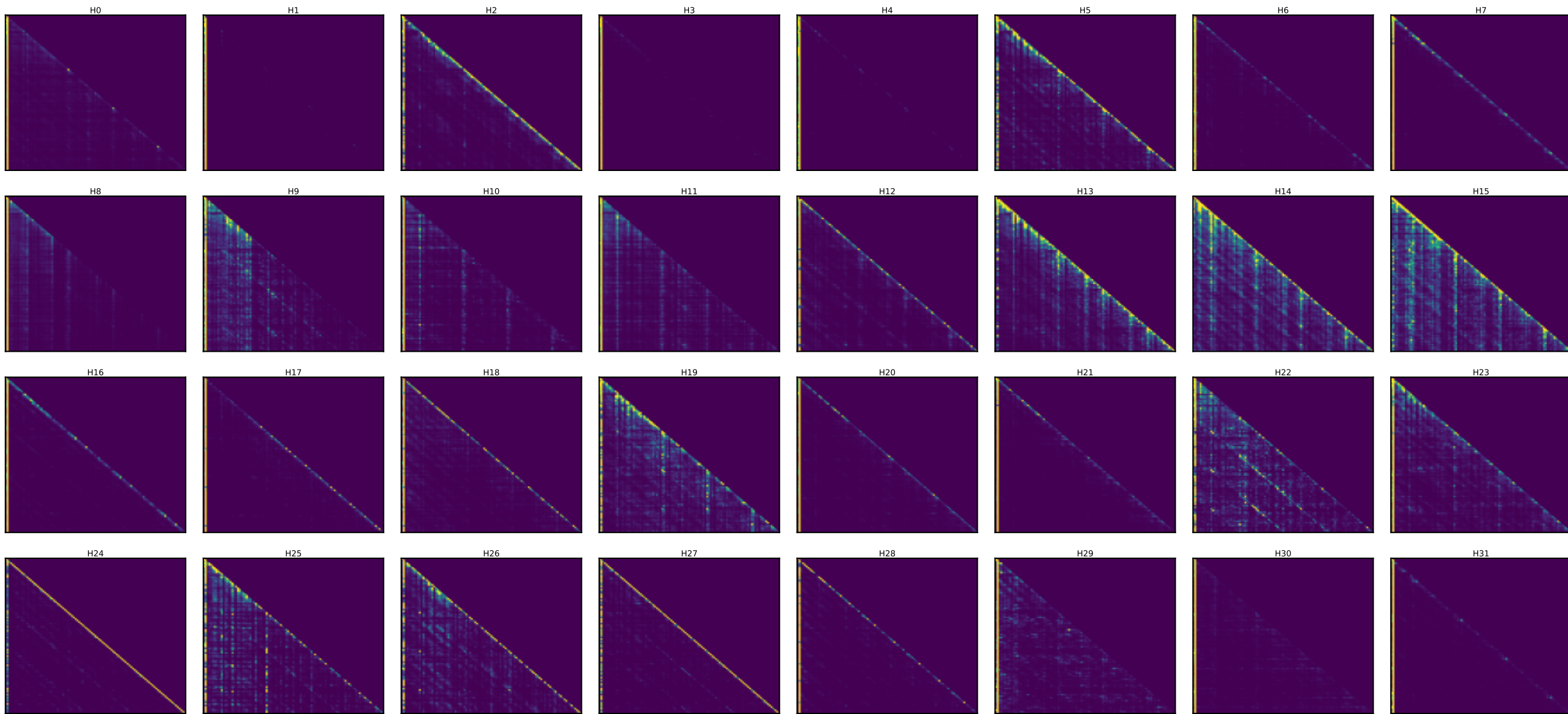
Qwen layer 35 — every head's attention [25 random toks x4 + SOS] (induction stripe = diagonal at key=query-25)
