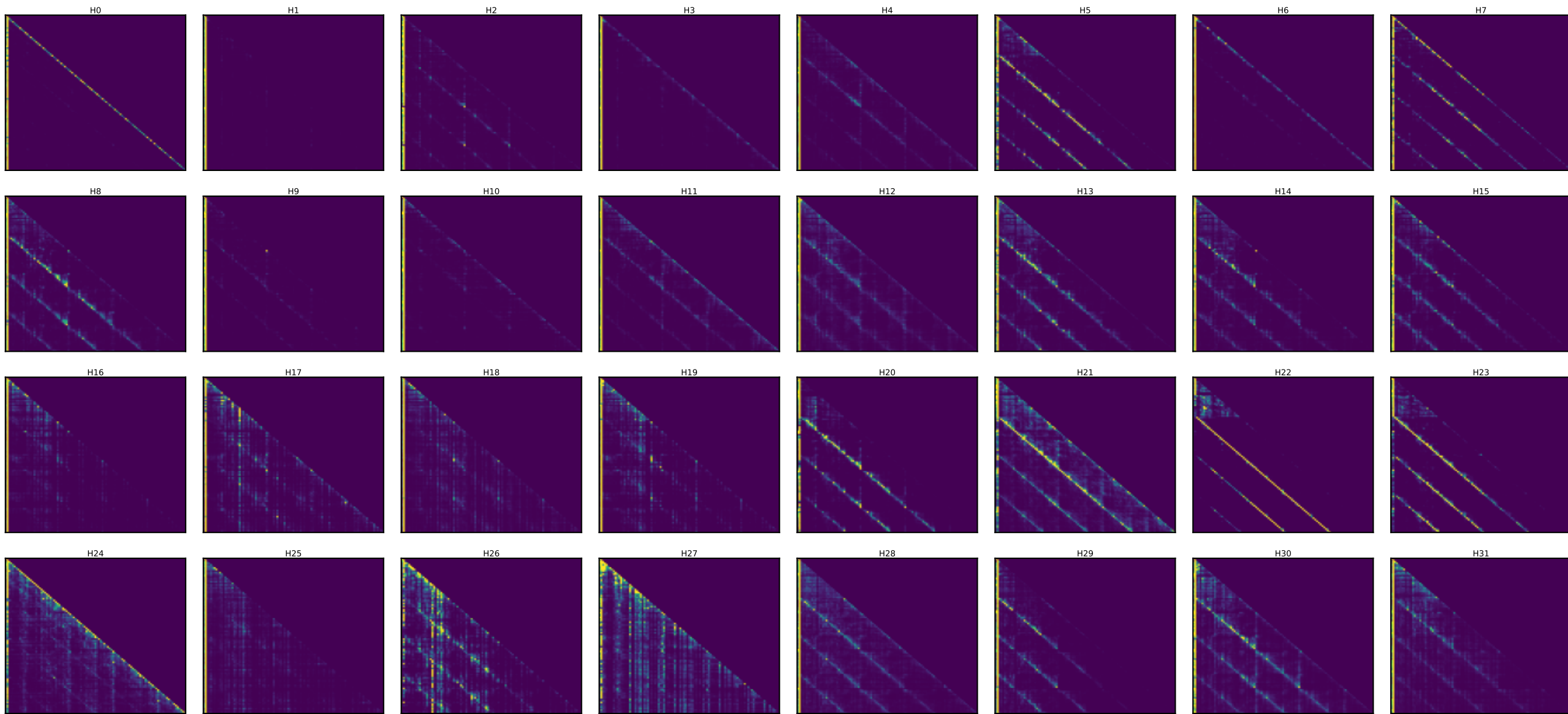
Qwen layer 24 — every head's attention [25 random toks x4 + SOS] (induction stripe = diagonal at key=query-25)
