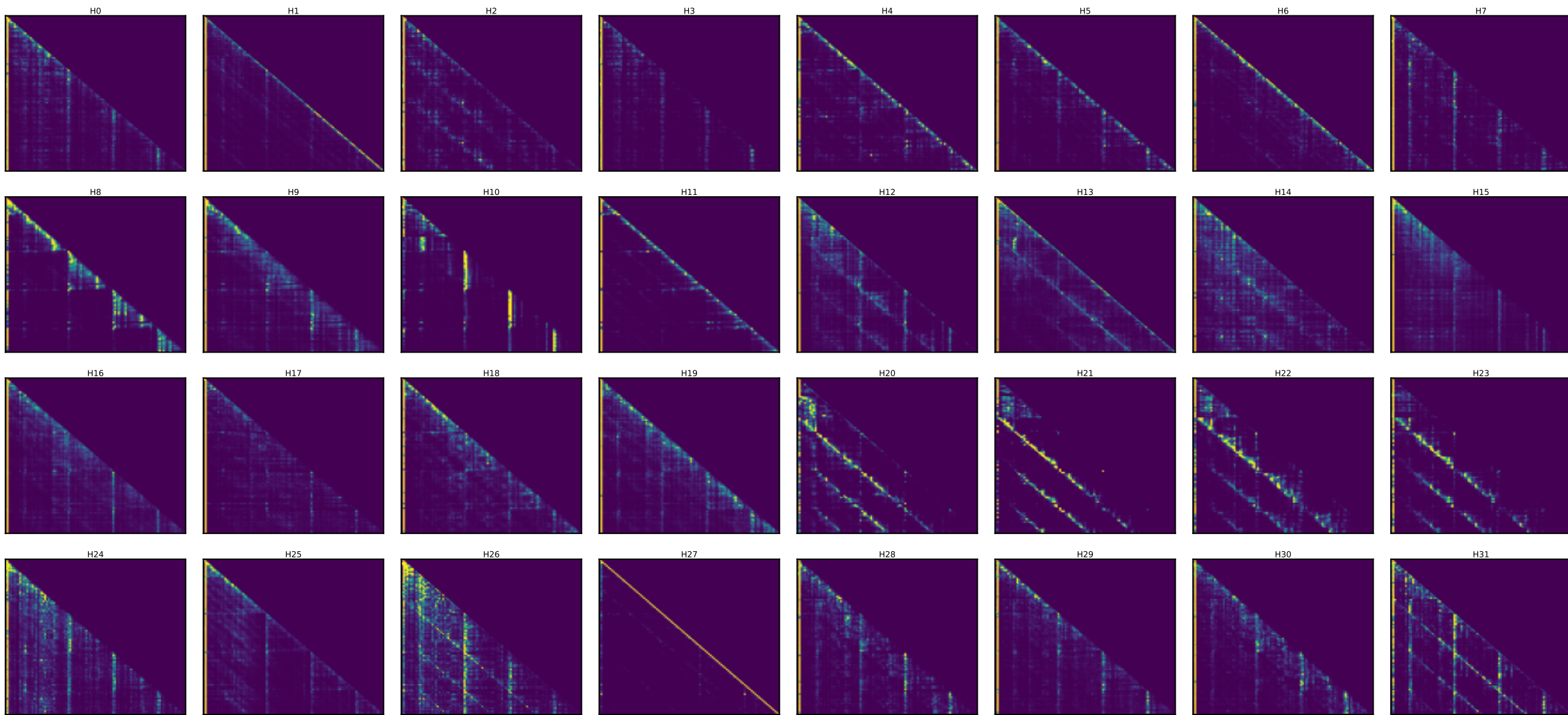
Qwen layer 16 — every head's attention [25 random toks x4 + SOS] (induction stripe = diagonal at key=query-25)
