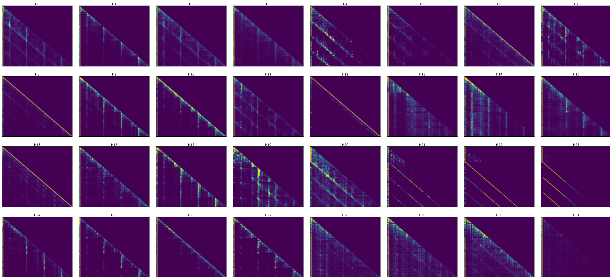
Qwen layer 22 — every head's attention [25 random toks x4 + SOS] (induction stripe = diagonal at key=query-25)
