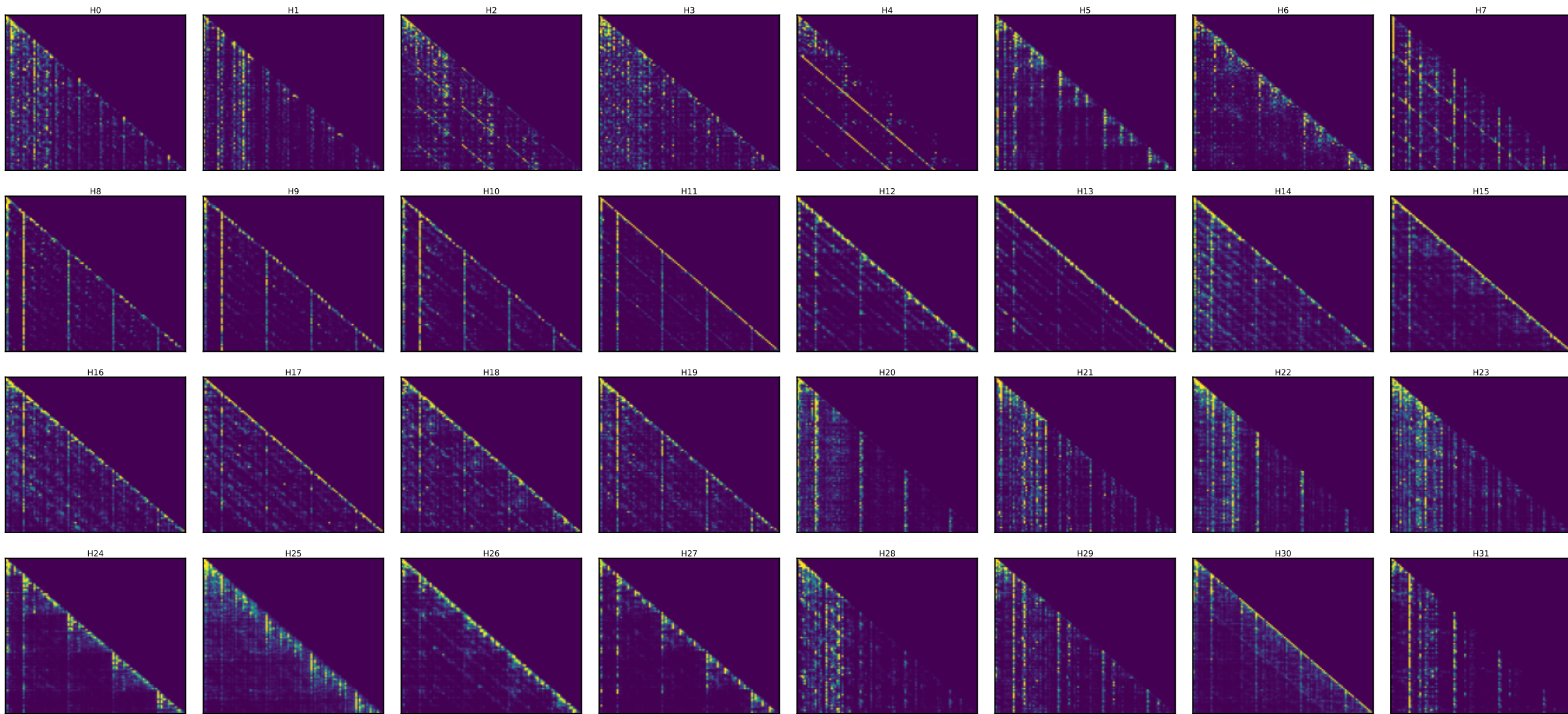
Qwen layer 4 — every head's attention [25 random toks x4 + SOS] (induction stripe = diagonal at key=query-25)
