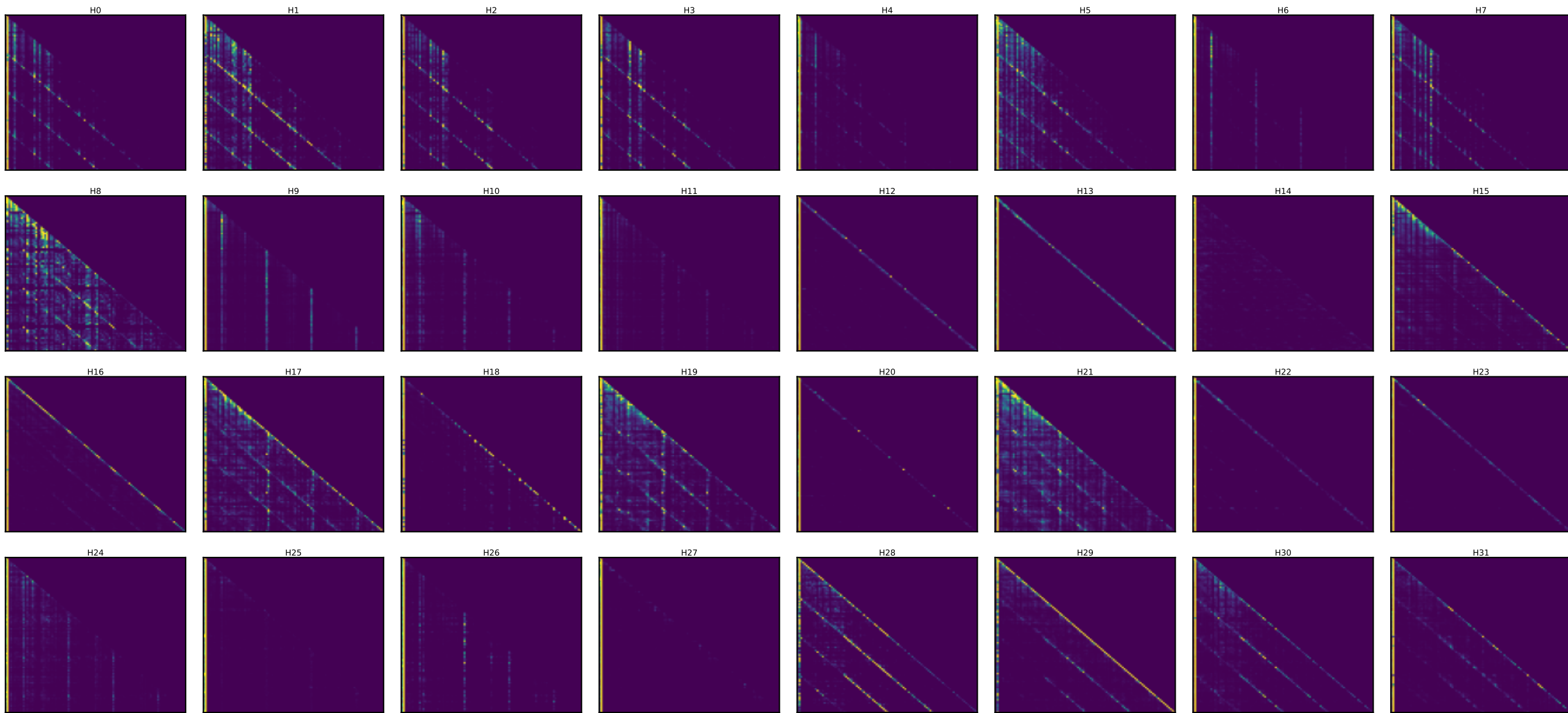
Qwen layer 34 — every head's attention [25 random toks x4 + SOS] (induction stripe = diagonal at key=query-25)
