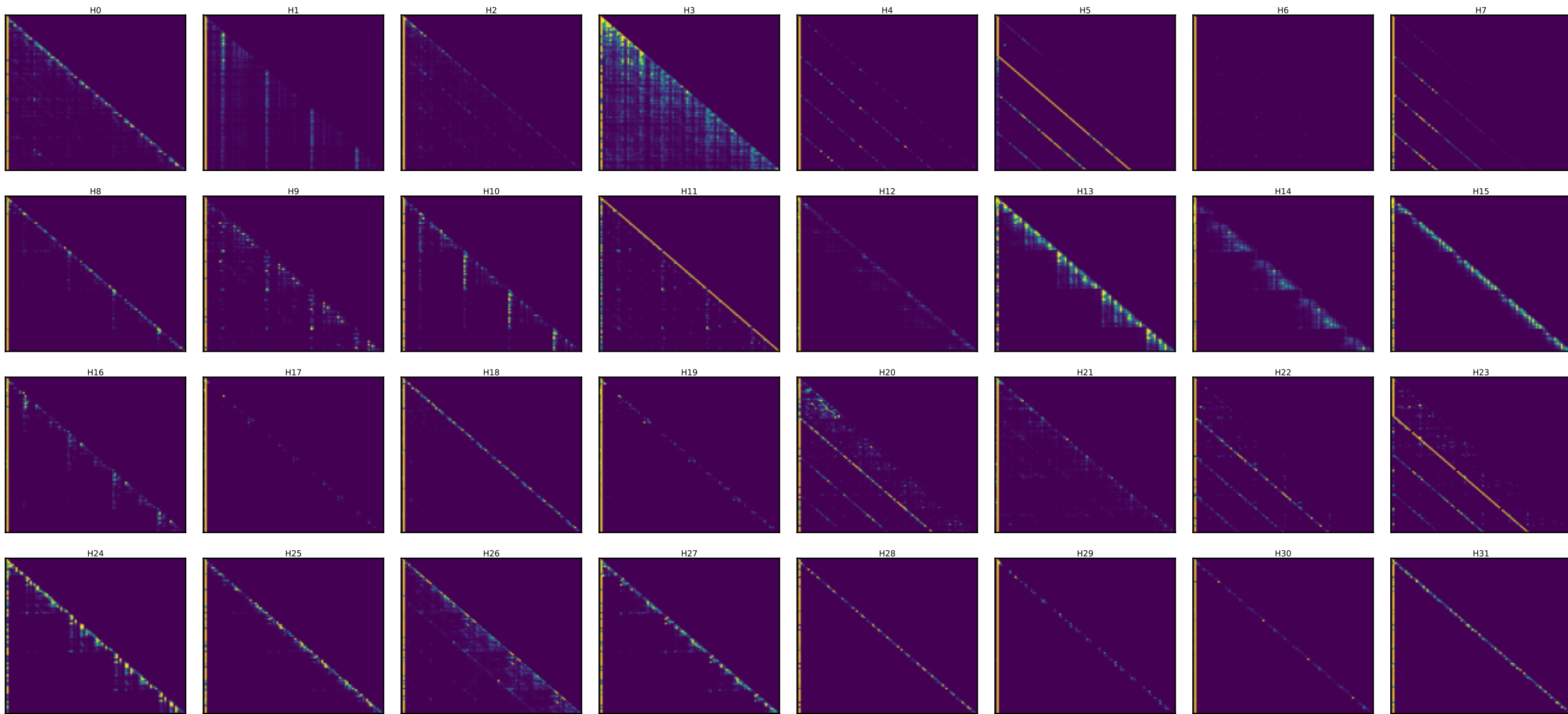
Qwen layer 7 — every head's attention [25 random toks x4 + SOS] (induction stripe = diagonal at key=query-25)
