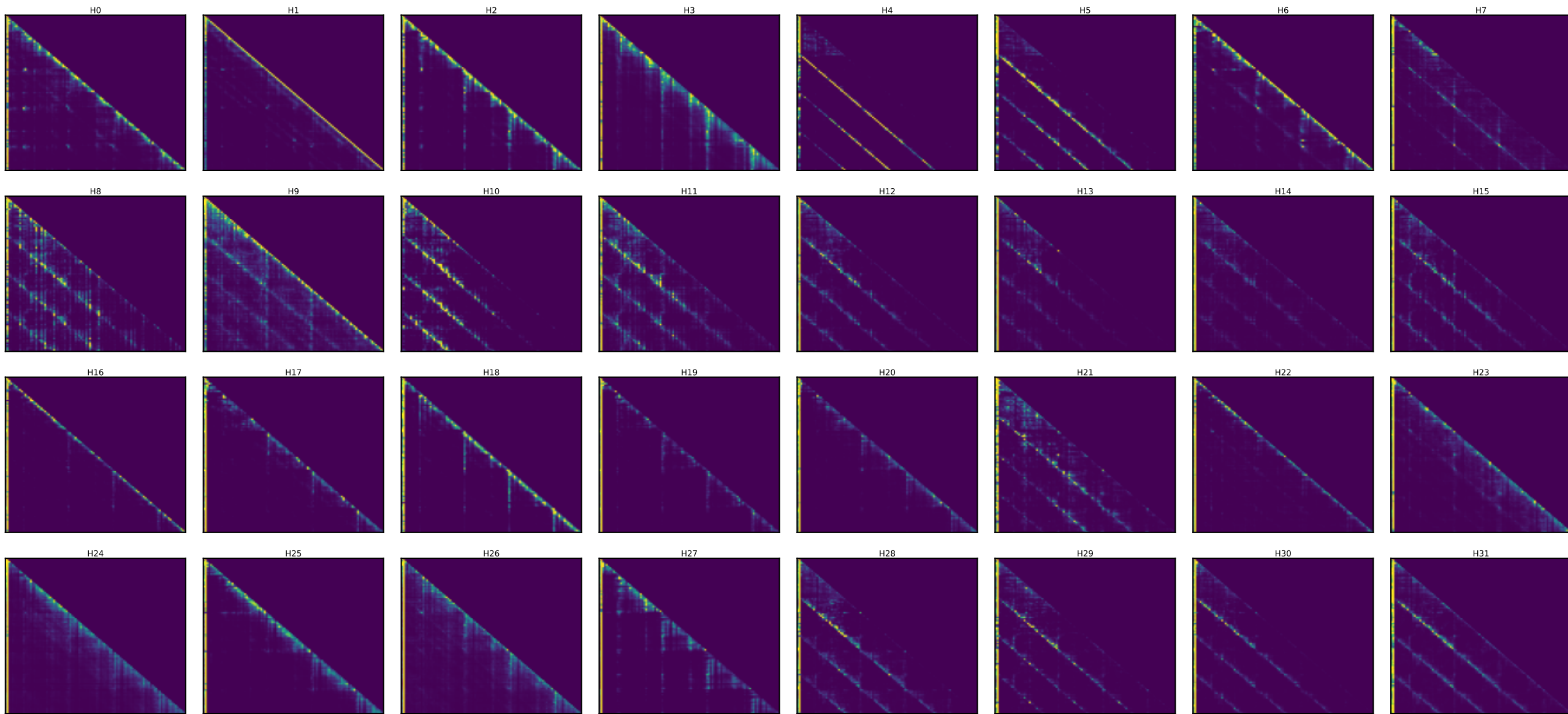
Qwen layer 23 — every head's attention [25 random toks x4 + SOS] (induction stripe = diagonal at key=query-25)
