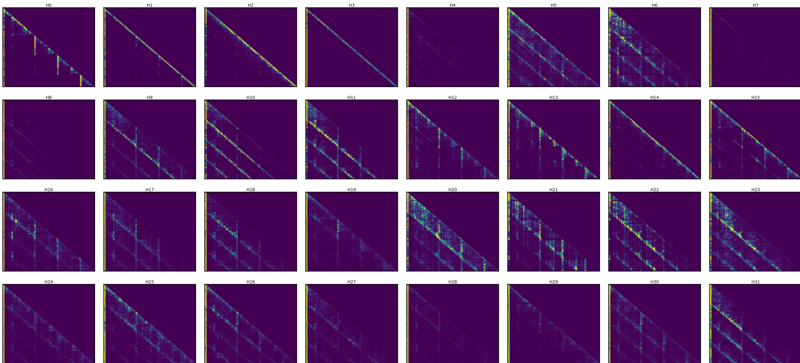
Qwen layer 21 — every head's attention [25 random toks x4 + SOS] (induction stripe = diagonal at key=query-25)
