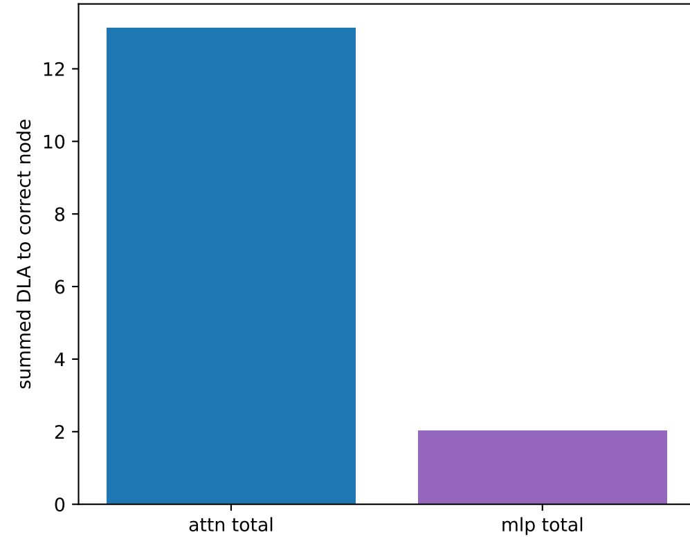
Gemma: who writes the answer? (attn +13.1 vs mlp +2.0)
