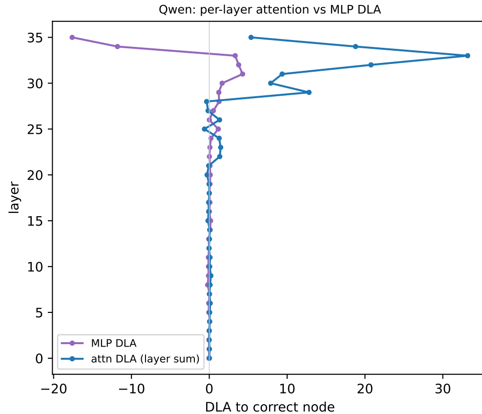
Qwen [square_grid]: direct logit attribution of the next-step prediction
