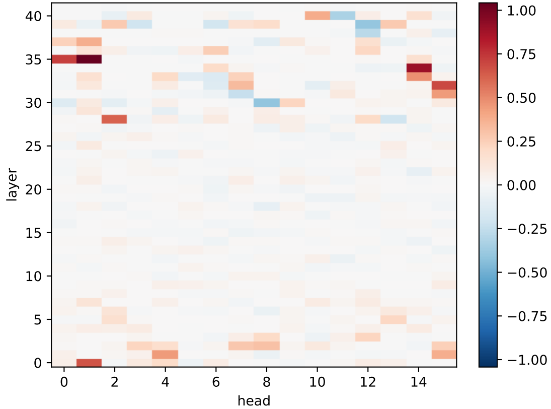
Gemma: per-head DLA to correct next node
